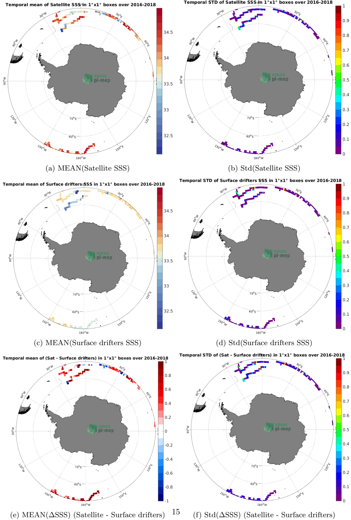
Figure 5: Temporal mean (left) and Std (right) of SSS from SMAP SSS L3 v5.0 - Monthly (JPL) (top), Surface drifters (middle), and of \Delta SSS (Satellite - Surface drifters). Only match-up pairs are used to generate these maps.
