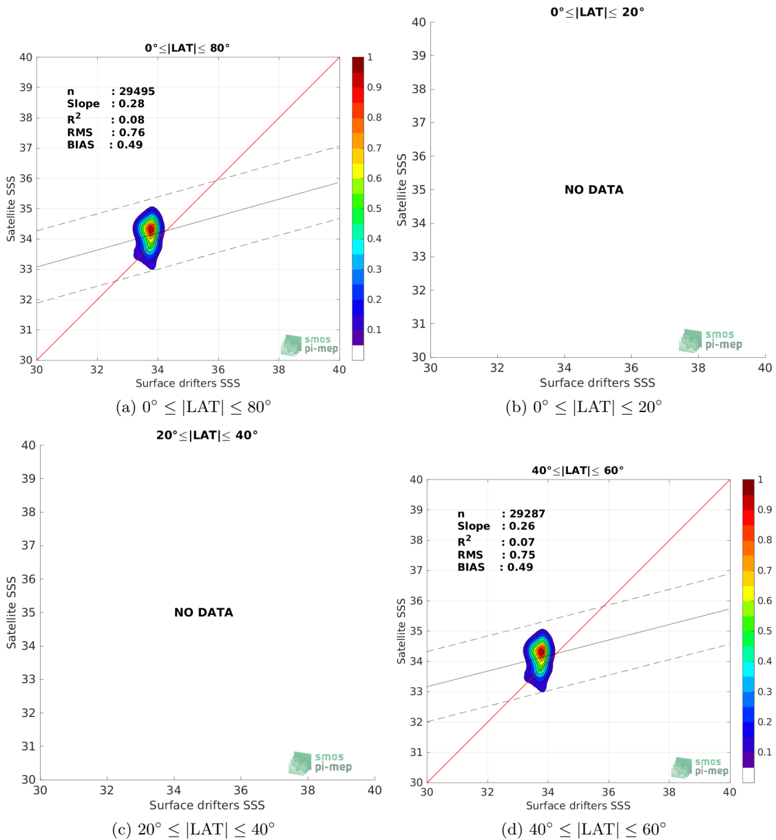
Figure 8: Contour maps of the concentration of SMAP SSS L3 v5.0 - Monthly (JPL) SSS (y-axis) versus Surface drifters SSS (x-axis) at match-up pairs for different latitude bands. For each plot, the red line shows x=y . The black thin and dashed lines indicate a linear fit through the data cloud and the \pm 95\% confidence levels, respectively. The number match-up pairs n , the slope and R^2 coefficient of the linear fit, the root mean square (RMS) and the mean bias between satellite and in situ data are indicated for each latitude band in each plots.
