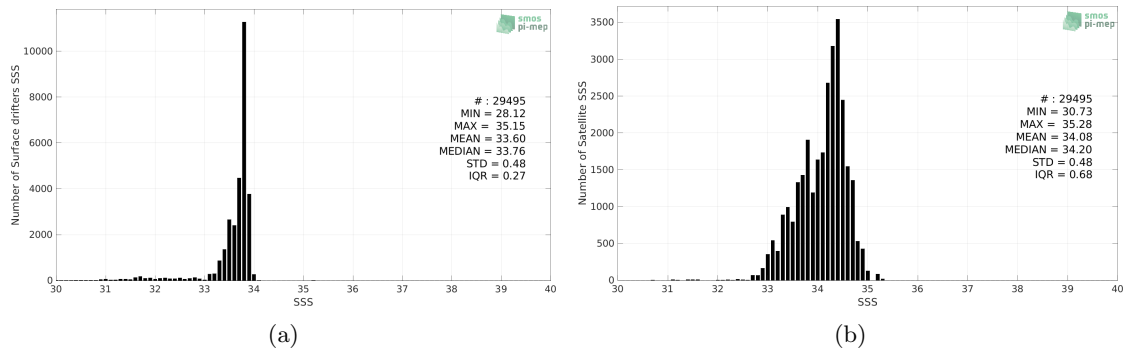
Figure 2: Histograms of SSS from Surface drifters (a) and SMAP SSS L3 v5.0 - Monthly (JPL) (b) considering all match-up pairs per bins of 0.1 over the Southern Ocean Pi-MEP region and for the full satellite product period.
