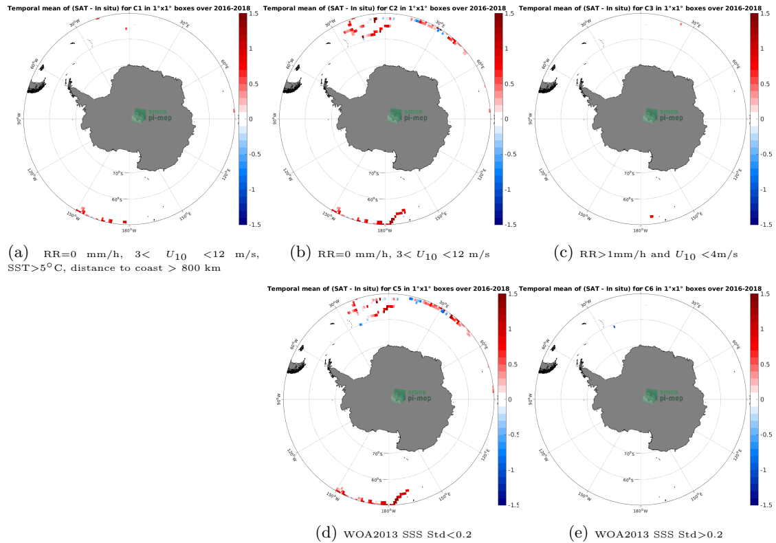
Figure 11: Temporal mean gridded over spatial boxes of size 1^{\circ}\times 1^{\circ} of \Delta\text{SSS} (SMAP SSS L3 v5.0 - Monthly (JPL) - Surface drifters) for 5 different subdatasets corresponding to:RR=0 mm/h, 3 < U_{10} < 12 m/s, SST >5^{\circ}\text{C} , distance to coast > 800 km (a), RR=0 mm/h, 3 < U_{10} < 12 m/s (b), RR >1 mm/h and U_{10} < 4 m/s (c), WOA2013 SSS Std <0.2 (d), WOA2013 SSS Std >0.2 (e).
