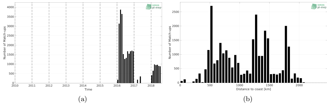
Figure 1: Number of match-ups between Surface drifters and SMAP SSS L3 v5.0 - Monthly (JPL) SSS as a function of time (a) and as function of the distance to coast (b) over the Southern Ocean Pi-MEP region and for the full satellite product period.
