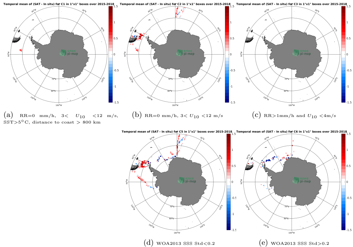
Figure 12: Temporal mean gridded over spatial boxes of size 1^\circ \times 1^\circ of \Delta SSS (SMAP-L3-JPL-V4.3-MONTHLY-60KM - TSG-POLARSTERN) for 5 different subdatasets corresponding to:RR=0 mm/h, 3 < U_{10} < 12 m/s, SST >5^\circ\text{C} , distance to coast > 800 km (a), RR=0 mm/h, 3 < U_{10} < 12 m/s (b), RR >1 mm/h and U_{10} < 4 m/s (c), WOA2013 SSS Std <0.2 (d), WOA2013 SSS Std >0.2 (e).
