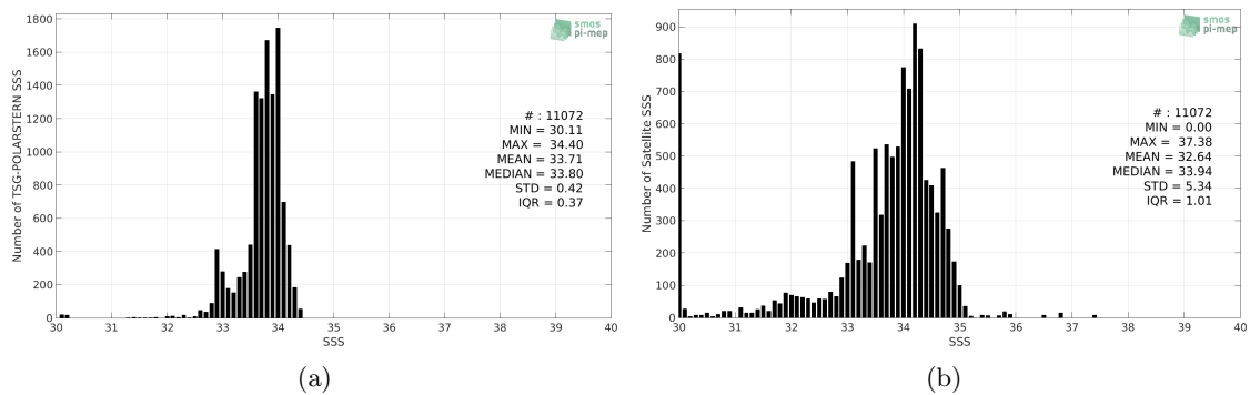
Figure 2: Histograms of SSS from TSG-POLARSTERN (a) and SMAP-L3-JPL-V4.3-MONTHLY-60KM (b) considering all match-up pairs per bins of 0.1 over the Southern Ocean Pi-MEP region and for the full satellite product period.
