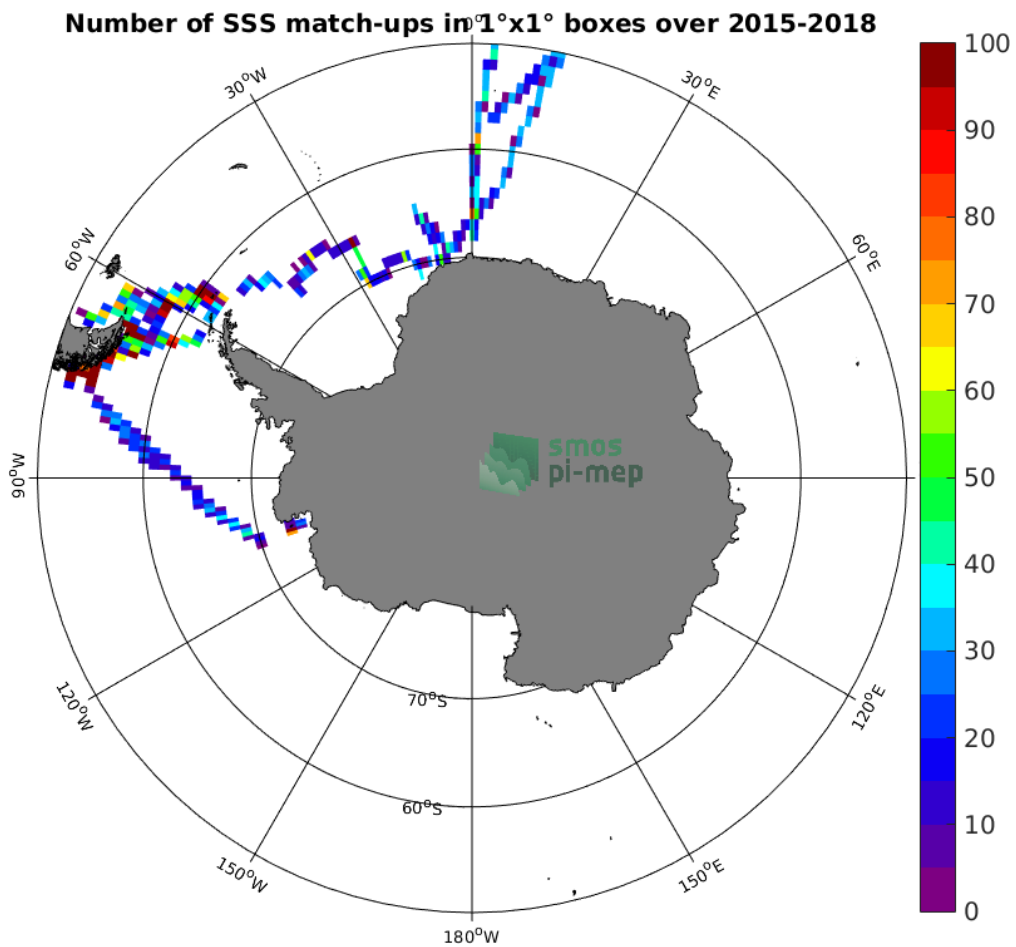
Figure 4: Number of SSS match-ups between TSG-POLARSTERN SSS and the SMAP-L3-JPL-V4.3-MONTHLY-60KM SSS product for the Southern Ocean Pi-MEP region over 1^\circ \times 1^\circ boxes and for the full satellite product period.
