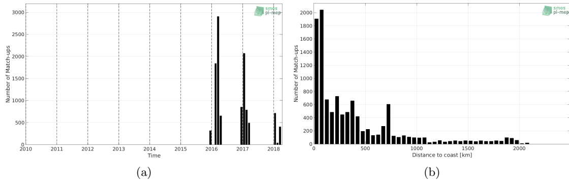
Figure 1: Number of match-ups between TSG-POLARSTERN and SMAP-L3-JPL-V4.3-MONTHLY-60KM SSS as a function of time (a) and as function of the distance to coast (b) over the Southern Ocean Pi-MEP region and for the full satellite product period.
