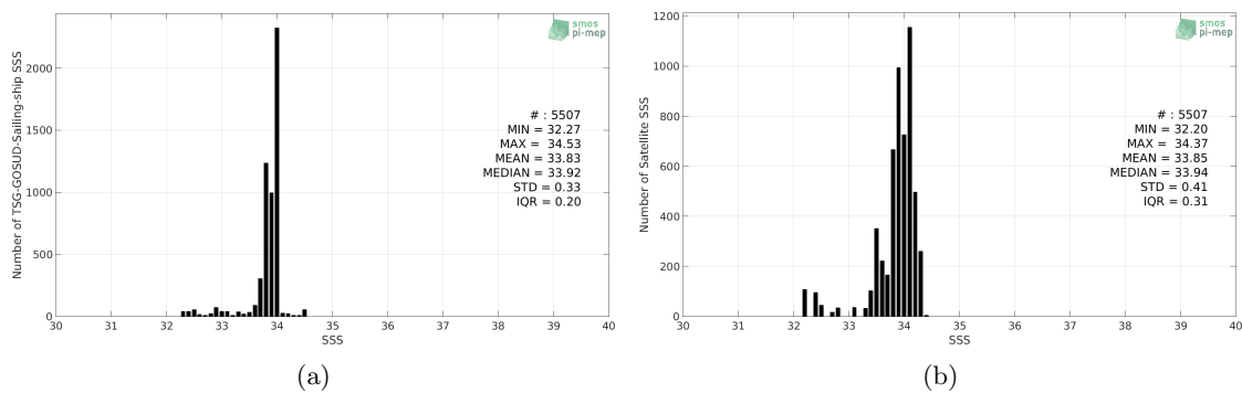
Figure 2: Histograms of SSS from TSG-GOSUD-Sailing-ship (a) and SMAP-L3-JPL-V4.3-MONTHLY-60KM (b) considering all match-up pairs per bins of 0.1 over the Southern Ocean Pi-MEP region and for the full satellite product period.
