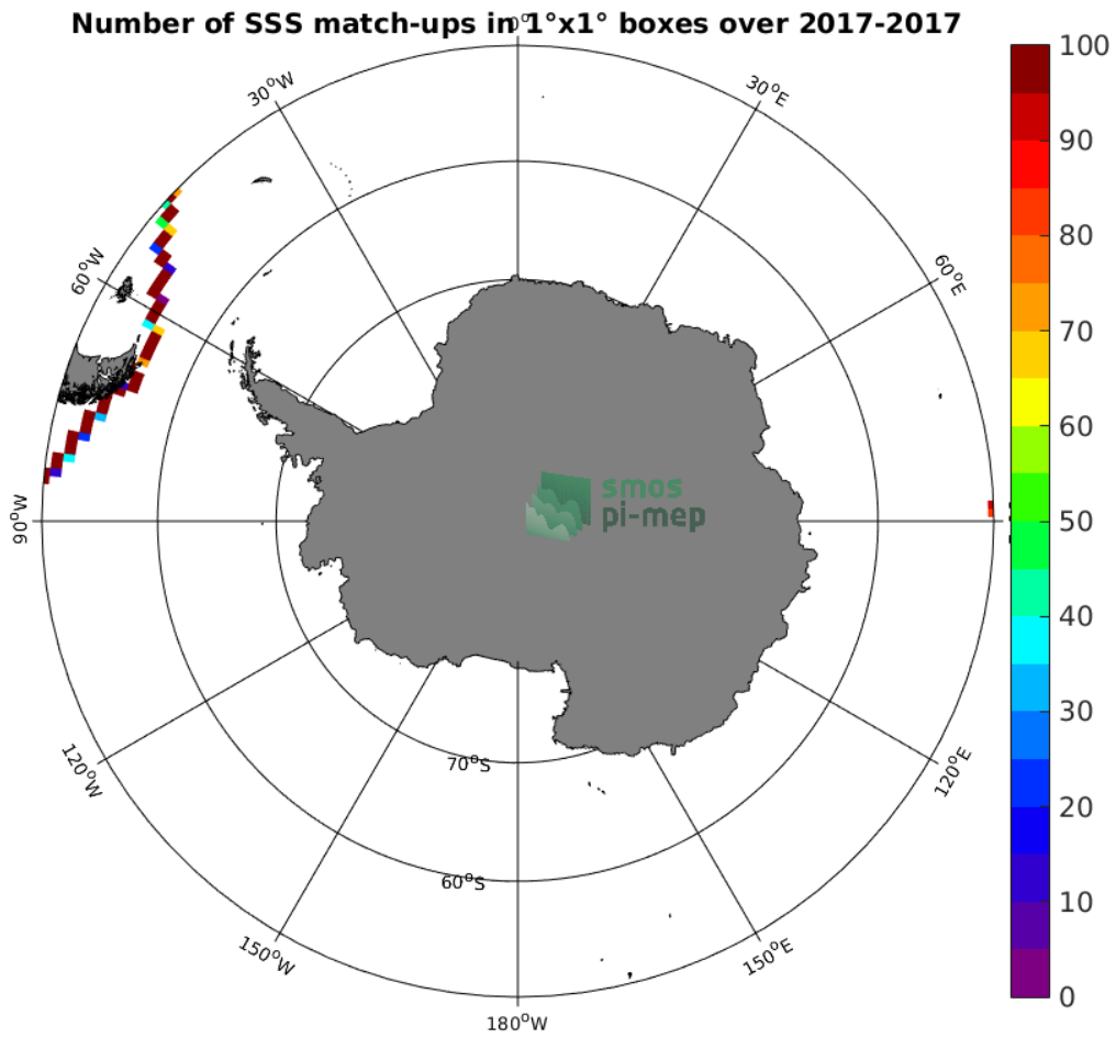
Figure 4: Number of SSS match-ups between TSG-GOSUD-Sailing-ship SSS and the SMAP-L3-JPL-V4.3-MONTHLY-60KM SSS product for the Southern Ocean Pi-MEP region over 1°x1° boxes and for the full satellite product period.
