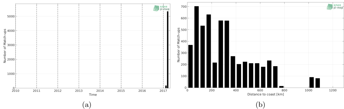
Figure 1: Number of match-ups between TSG-GOSUD-Sailing-ship and SMAP-L3-JPL-V4.3-MONTHLY-60KM SSS as a function of time (a) and as function of the distance to coast (b) over the Southern Ocean Pi-MEP region and for the full satellite product period.
