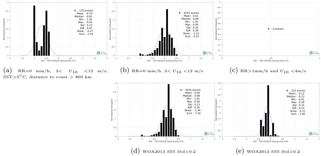
Figure 13: Normalized histogram of \Delta SSS (SMAP-L3-JPL-V4.3-MONTHLY-60KM - TSG-GOSUD-Sailing-ship) for 5 different subdatasets corresponding to: RR=0 mm/h, 3 < U_{10} < 12 m/s, SST > 5°C, distance to coast > 800 km (a), RR=0 mm/h, 3 < U_{10} < 12 m/s (b), RR > 1mm/h and U_{10} < 4 m/s (c), WOA2013 SSS Std < 0.2 (d), WOA2013 SSS Std > 0.2 (e).
