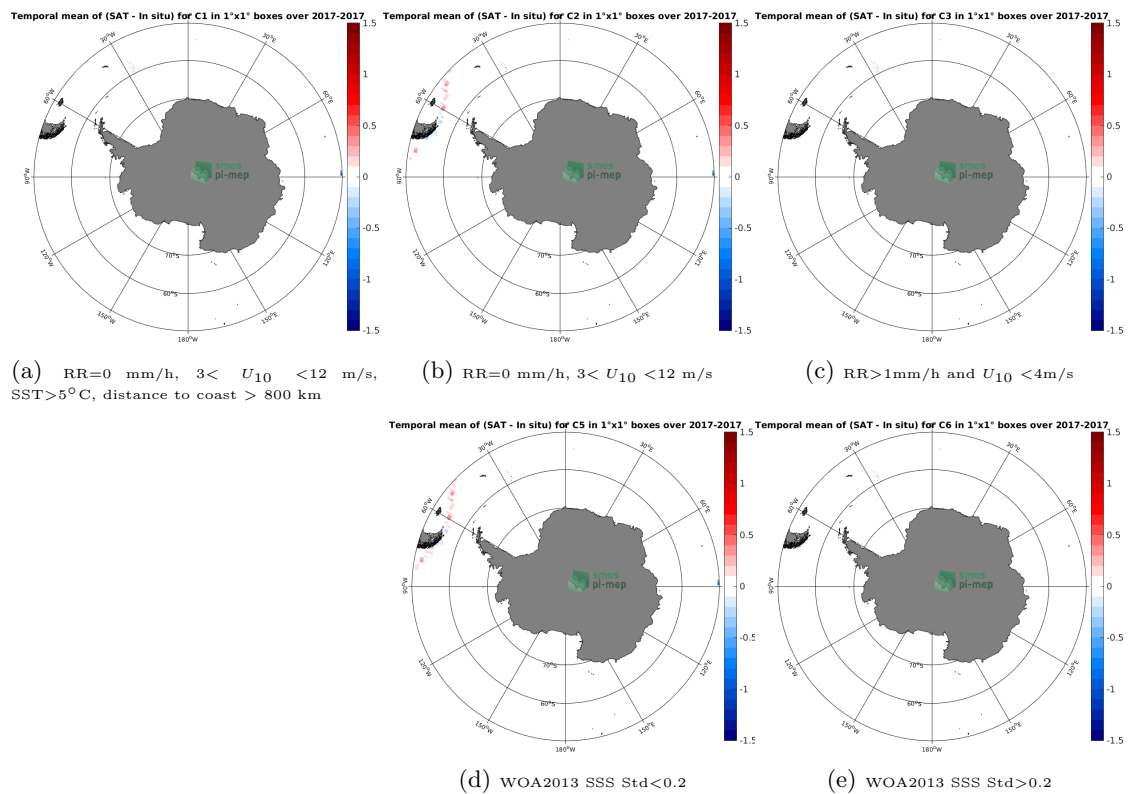
Figure 12: Temporal mean gridded over spatial boxes of size 1^\circ \times 1^\circ of \Delta SSS (SMAP-L3-JPL-V4.3-MONTHLY-60KM - TSG-GOSUD-Sailing-ship) for 5 different subdatasets corresponding to:RR=0 mm/h, 3 < U_{10} < 12 m/s, SST>5°C, distance to coast > 800 km (a), RR=0 mm/h, 3 < U_{10} < 12 m/s (b), RR>1mm/h and U_{10} < 4 m/s (c), WOA2013 SSS Std<0.2 (d), WOA2013 SSS Std>0.2 (e).
