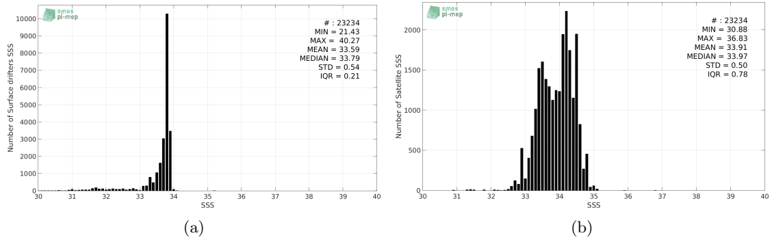
Figure 2: Histograms of SSS from Surface drifters (a) and SMAP-L3-JPL-V4-MONTHLY-60KM (b) considering all match-up pairs per bins of 0.1 over the Southern Ocean Pi-MEP region and for the full satellite product period.
