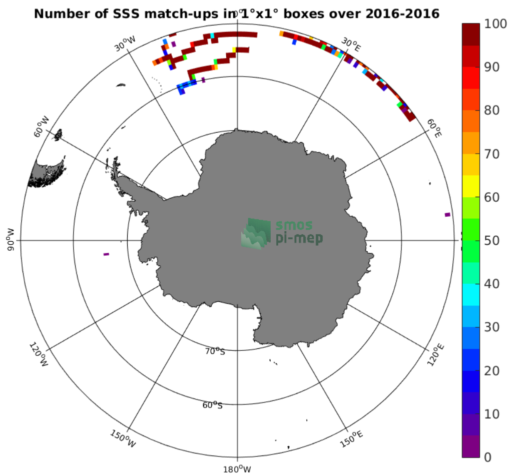
Figure 3: Number of SSS match-ups between Surface drifters SSS and the SMAP-L3-JPL-V4-MONTHLY-60KM SSS product for the Southern Ocean Pi-MEP region over 1^\circ \times 1^\circ boxes and for the full satellite product period.
