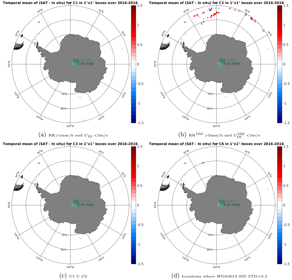
Figure 11: Temporal mean gridded over spatial boxes of size 1^\circ \times 1^\circ of \Delta SSS (SMAP-L3-JPL-V4-MONTHLY-60KM - Surface drifters) for 4 different subdatasets corresponding to: RR > 1mm/h and U_{10} < 5\text{m/s} (a), RR 10d > 5mm/h and U_{10}^{10d} < 5\text{m/s} (b), C1 U C2 (c), Locations where WOA2013 SSS STD > 0.2 (d).
