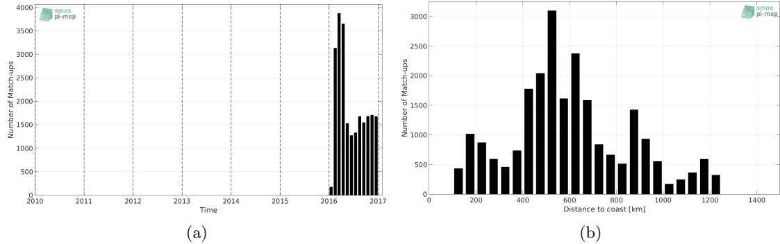
Figure 1: Number of match-ups between Surface drifters and SMAP-L3-JPL-V4-MONTHLY-60KM SSS as a function of time (a) and as function of the distance to coast (b) over the Southern Ocean Pi-MEP region and for the full satellite product period.
