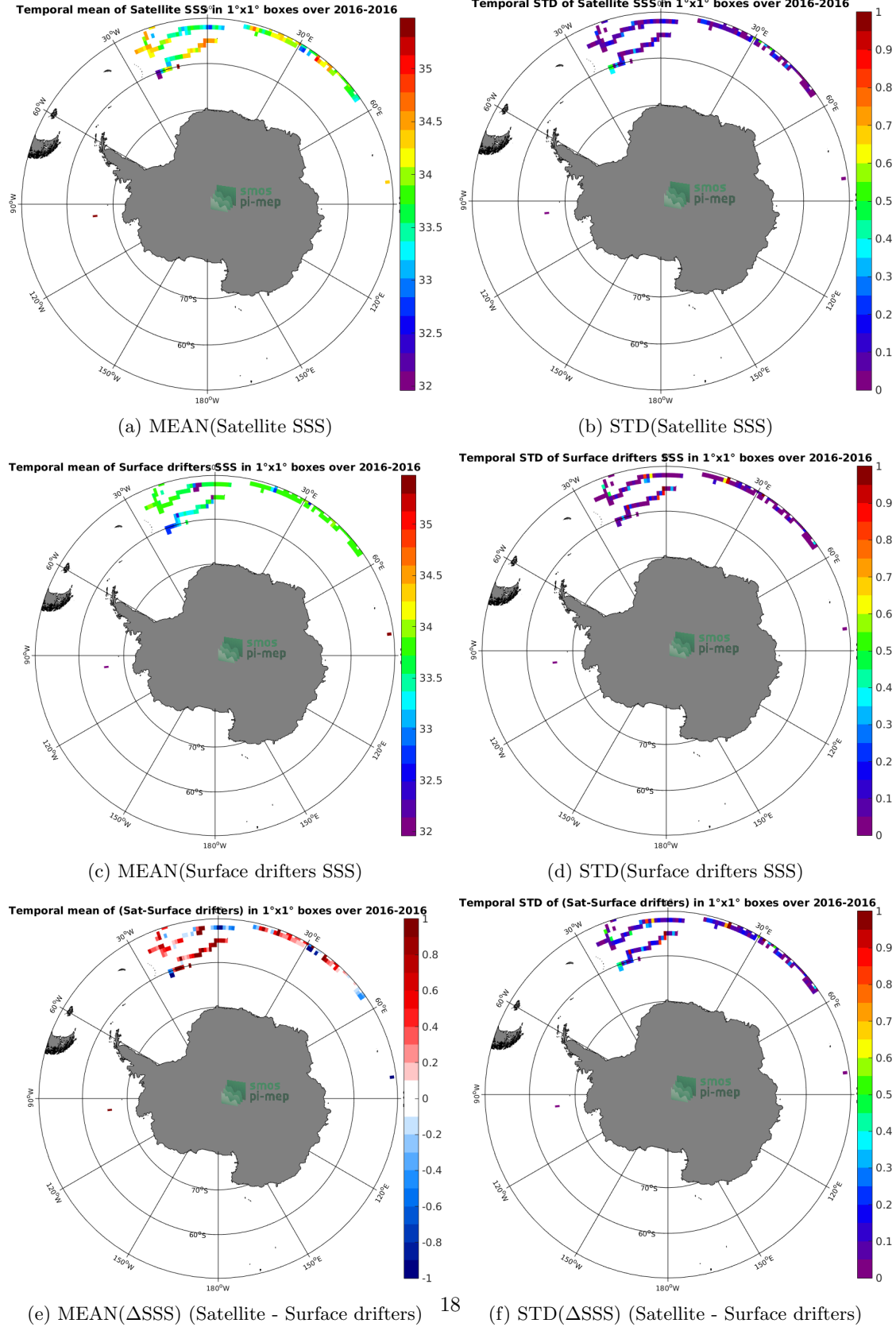
Figure 5: Temporal mean (left) and STD (right) of SSS from SMAP-L3-JPL-V4-MONTHLY-60KM (top), Surface drifters (middle), and of \Delta SSS (Satellite - Surface drifters). Only match-up pairs are used to generate these maps.
