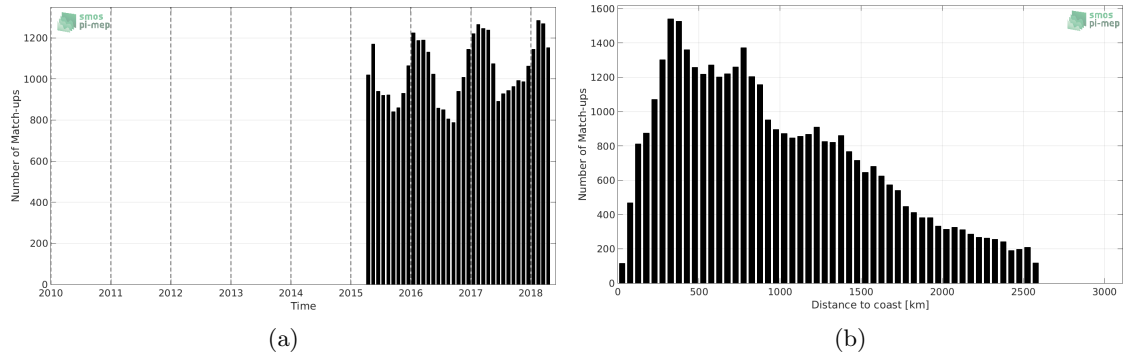
Figure 1: Number of match-ups between Argo and SMAP-L3-JPL-V4-MONTHLY-60KM SSS as a function of time (a) and as function of the distance to coast (b) over the Southern Ocean Pi-MEP region and for the full satellite product period.
