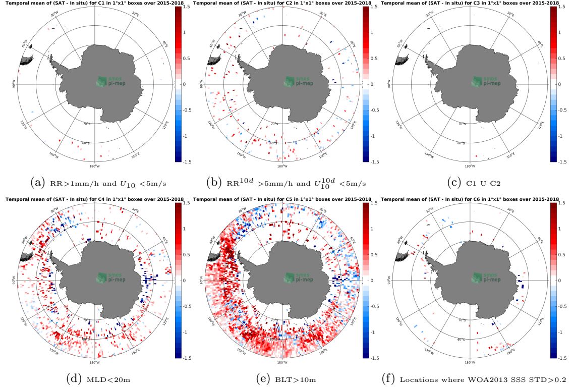
Figure 12: Temporal mean gridded over spatial boxes of size 1^\circ \times 1^\circ of \Delta\text{SSS} (SMAP-L3-JPL-V4-MONTHLY-60KM - Argo) for 6 different subdatasets corresponding to: \text{RR} > 1\text{mm/h} and U_{10} < 5\text{m/s} (a), \text{RR}^{10d} > 5\text{mm/h} and U_{10}^{10d} < 5\text{m/s} (b), C1 U C2 (c), \text{MLD} < 20\text{m} (d), \text{BLT} > 10\text{m} (e), Locations where WOA2013 SSS STD > 0.2 (f).
