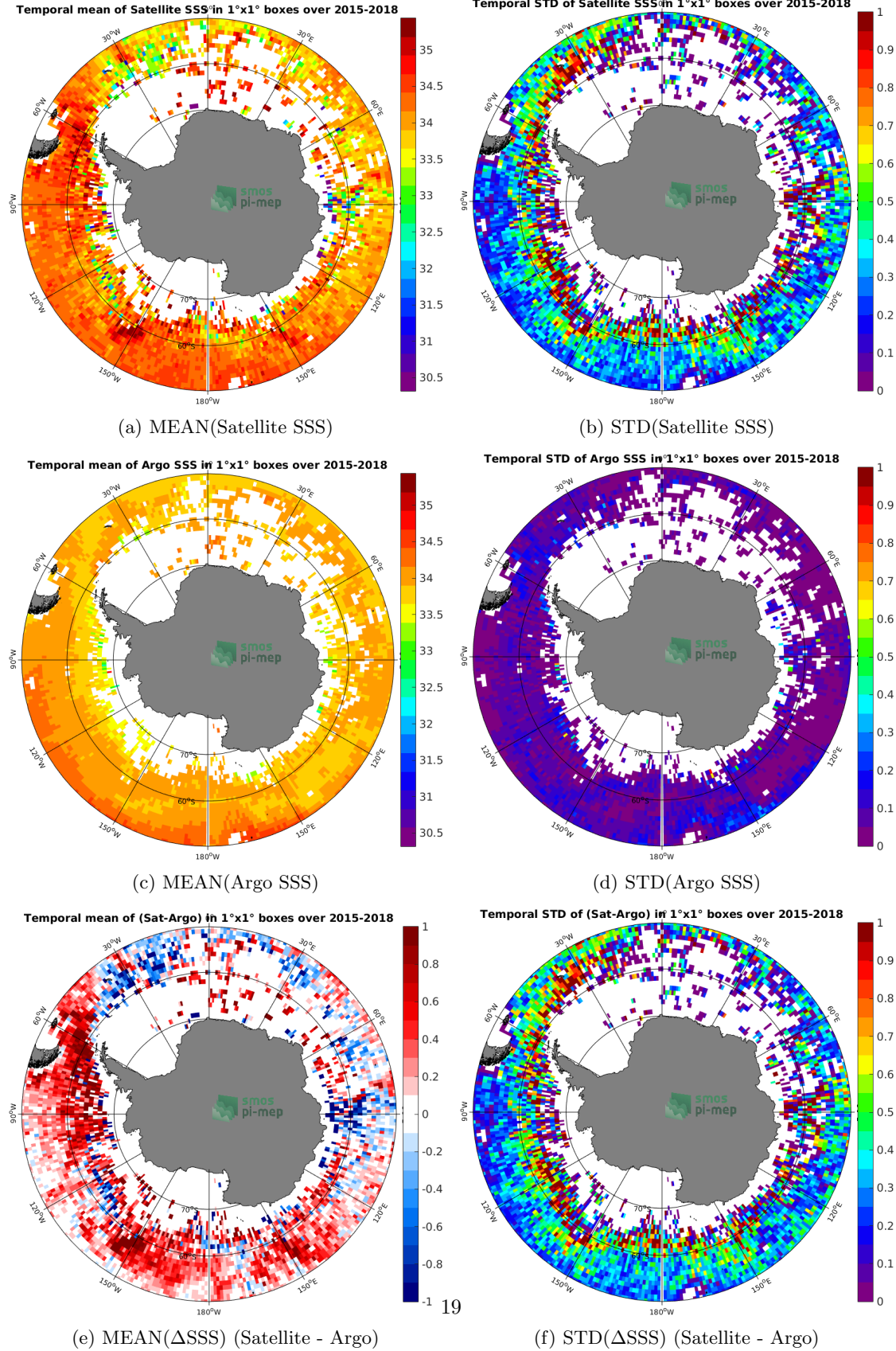
Figure 6: Temporal mean (left) and STD (right) of SSS from SMAP-L3-JPL-V4-MONTHLY-60KM (top), Argo (middle), and of \Delta SSS (Satellite - Argo). Only match-up pairs are used to generate these maps.
