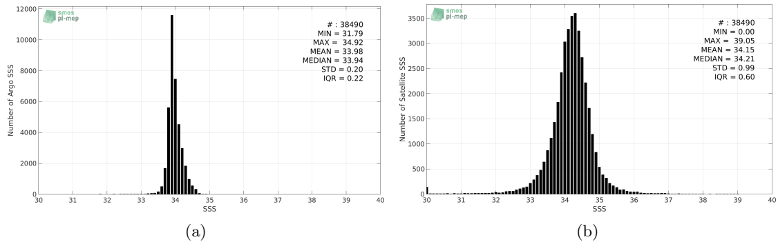
Figure 2: Histograms of SSS from Argo (a) and SMAP-L3-JPL-V4-MONTHLY-60KM (b) considering all match-up pairs per bins of 0.1 over the Southern Ocean Pi-MEP region and for the full satellite product period.
