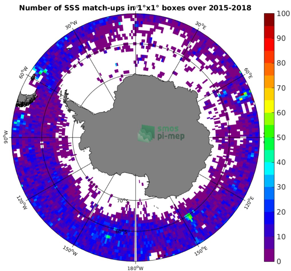
Figure 4: Number of SSS match-ups between Argo SSS and the SMAP-L3-JPL-V4-MONTHLY-60KM SSS product for the Southern Ocean Pi-MEP region over 1^\circ \times 1^\circ boxes and for the full satellite product period.
