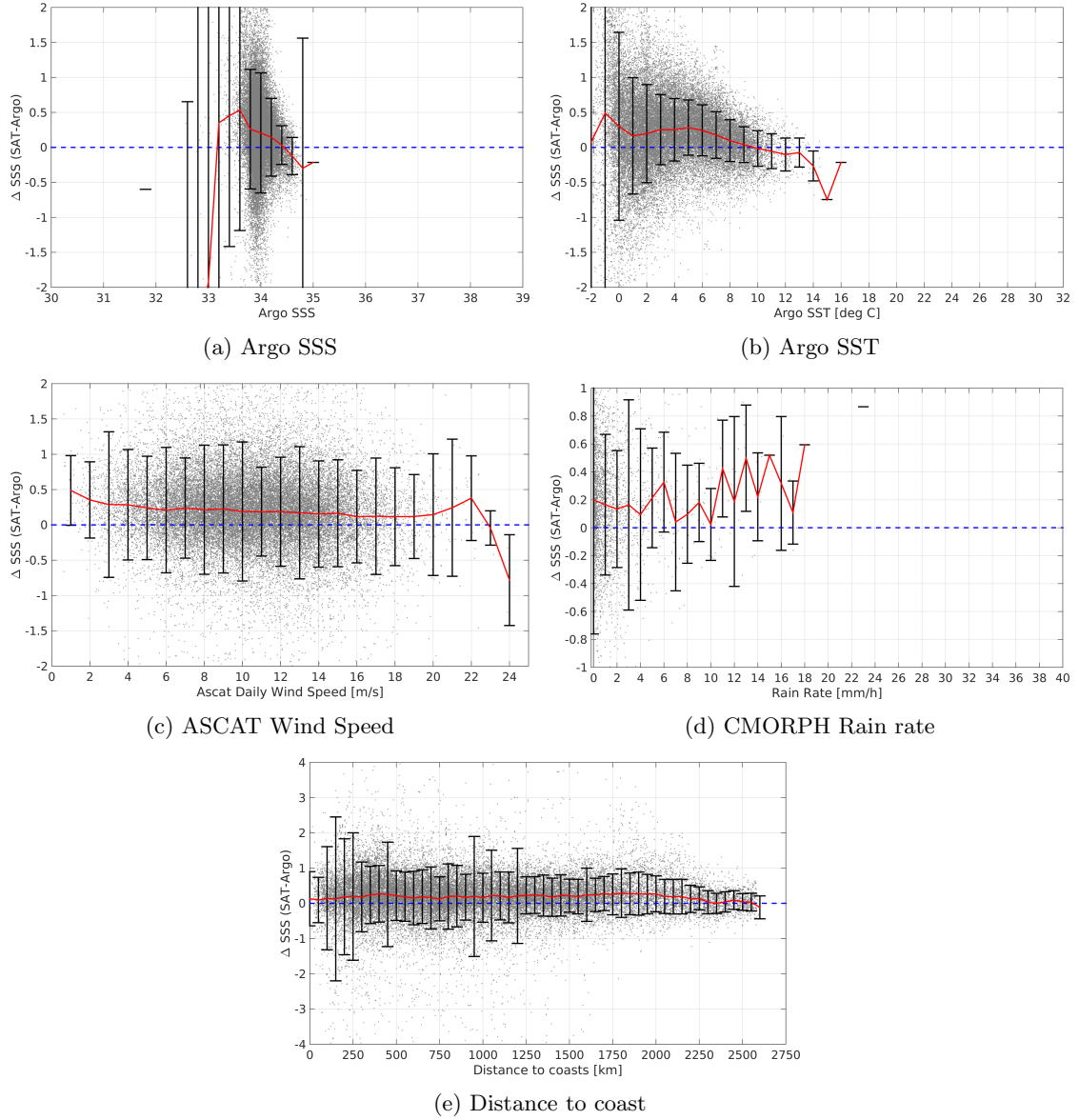
Figure 11: \Delta SSS (Satellite - Argo) sorted as function of Argo SSS a), Argo SST b), ASCAT Wind speed c), CMORPH rain rate d) and distance to coast (e). In all plots the mean and STD of \Delta SSS for each bin is indicated by the red curves and black vertical thick bars ( \pm 1 STD)
