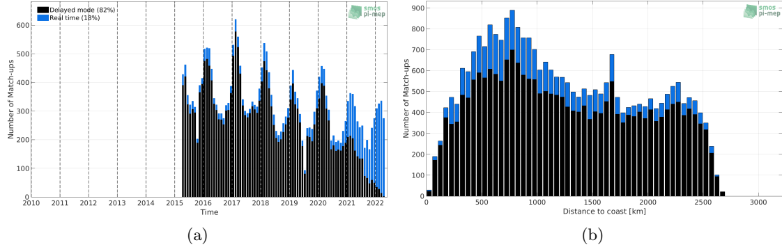
Figure 1: Number of match-ups between Argo and SMAP SSS L2-AVERAGED v5 (RSS) SSS as a function of time (a) and as function of the distance to coast (b) over the Southern Ocean Pi-MEP region and for the full satellite product period.
