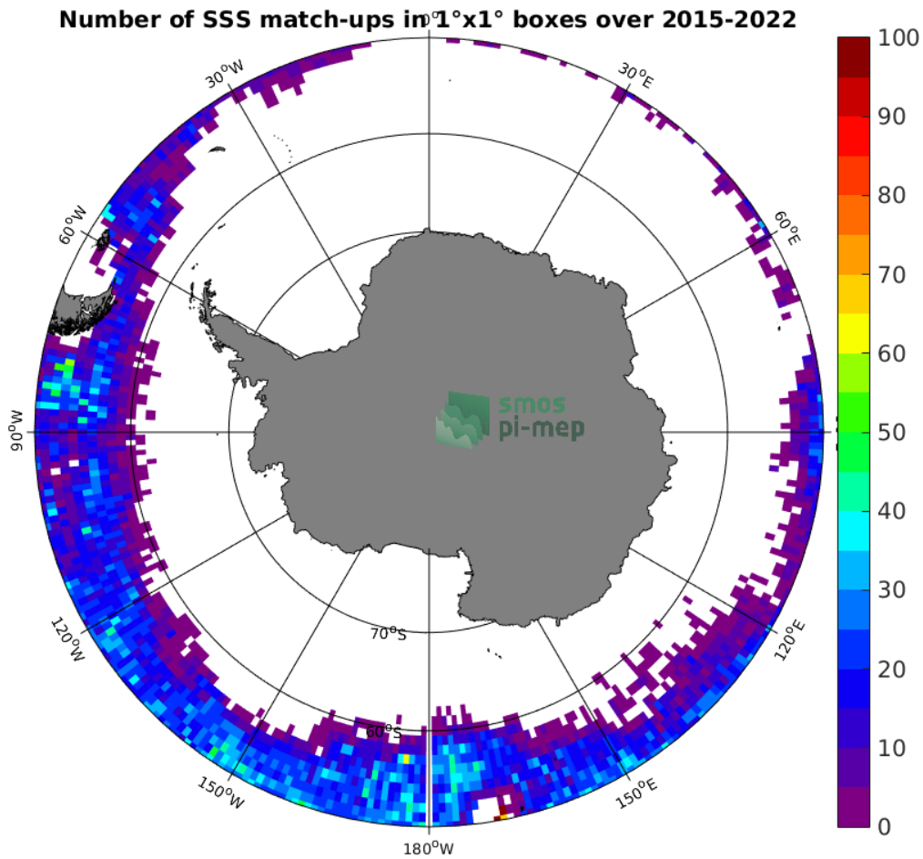
Figure 4: Number of SSS match-ups between Argo SSS and the SMAP SSS L2-AVERAGED v5 (RSS) SSS product for the Southern Ocean Pi-MEP region over 1^\circ \times 1^\circ boxes and for the full satellite product period.
