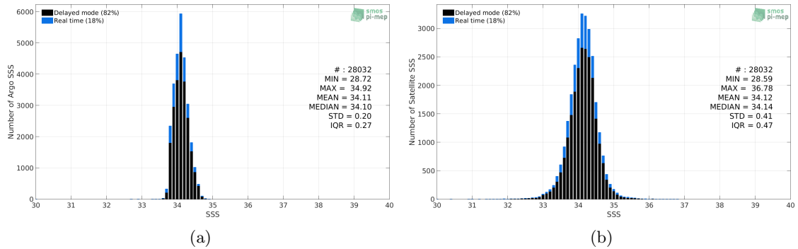
Figure 2: Histograms of SSS from Argo (a) and SMAP SSS L2-AVERAGED v5 (RSS) (b) considering all match-up pairs per bins of 0.1 over the Southern Ocean Pi-MEP region and for the full satellite product period.
