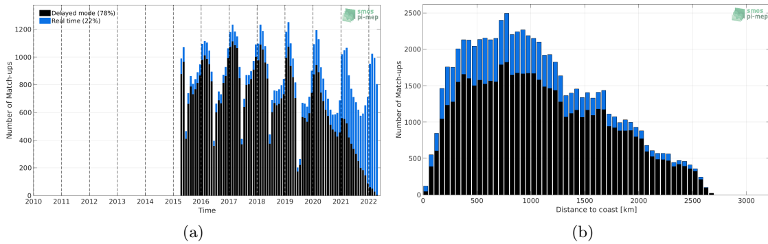
Figure 1: Number of match-ups between Argo and SMAP SSS L2-AVERAGED v5.0 (JPL) SSS as a function of time (a) and as function of the distance to coast (b) over the Southern Ocean Pi-MEP region and for the full satellite product period.
