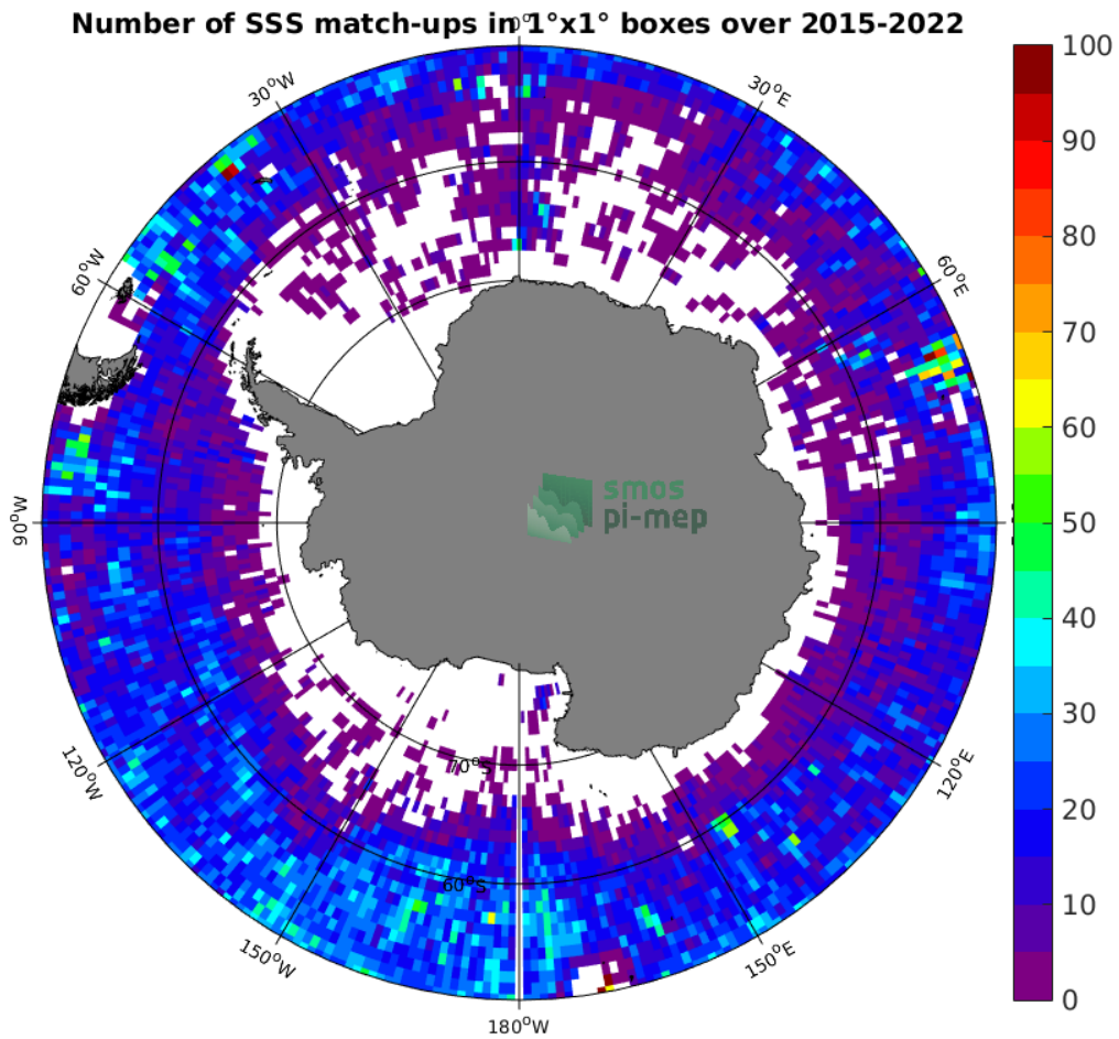
Figure 4: Number of SSS match-ups between Argo SSS and the SMAP SSS L2-AVERAGED v5.0 (JPL) SSS product for the Southern Ocean Pi-MEP region over 1^\circ \times 1^\circ boxes and for the full satellite product period.
