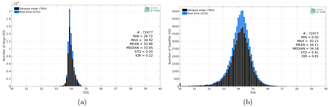
Figure 2: Histograms of SSS from Argo (a) and SMAP SSS L2-AVERAGED v5.0 (JPL) (b) considering all match-up pairs per bins of 0.1 over the Southern Ocean Pi-MEP region and for the full satellite product period.
