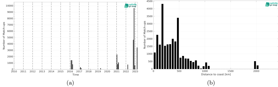
Figure 2: Number of match-ups between TSG (Polarstern) and SMAP SSS L2 v6 (RSS) SSS as a function of time (a) and as function of the distance to coast (b) over the Southern Ocean Pi-MEP region and for the full satellite product period.
