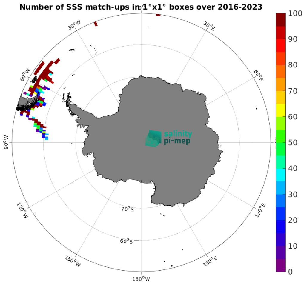
Figure 5: Number of SSS match-ups between TSG (Polarstern) SSS and the SMAP SSS L2 v6 (RSS) SSS product for the Southern Ocean Pi-MEP region over 1^\circ \times 1^\circ boxes and for the full satellite product period.
