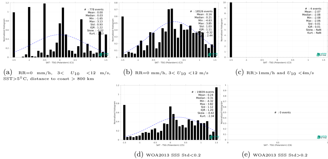
Figure 15: Normalized histogram of \Delta\text{SSS} (SMAP SSS L2 v6 (RSS) - TSG (Polarstern)) for 5 different subdatasets corresponding to: RR=0 mm/h, 3 < U_{10} < 12 m/s, SST > 5^\circ\text{C} , distance to coast > 800 km (a), RR=0 mm/h, 3 < U_{10} < 12 m/s (b), RR > 1\text{mm/h} and U_{10} < 4\text{m/s} (c), WOA2013 SSS \text{Std} < 0.2 (d), WOA2013 SSS \text{Std} > 0.2 (e).
