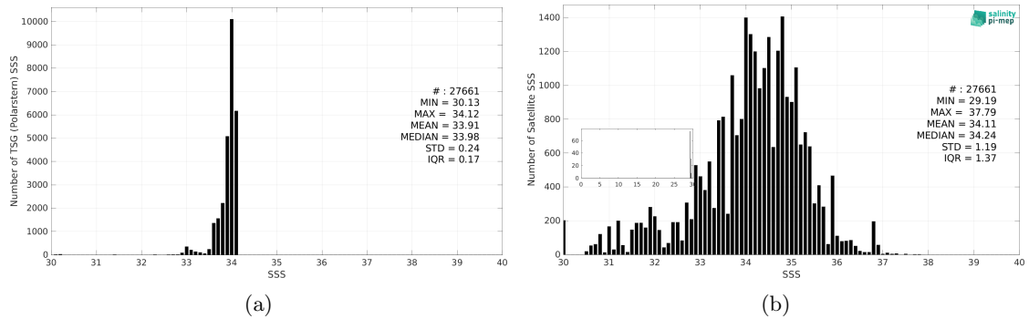
Figure 3: Histograms of SSS from TSG (Polarstern) (a) and SMAP SSS L2 v6 (RSS) (b) considering all match-up pairs per bins of 0.1 over the Southern Ocean Pi-MEP region and for the full satellite product period.
