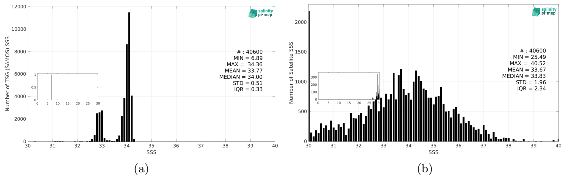
Figure 3: Histograms of SSS from TSG (SAMOS) (a) and SMAP SSS L2 v6 - 40 km (RSS) (b) considering all match-up pairs per bins of 0.1 over the Southern Ocean Pi-MEP region and for the full satellite product period.
