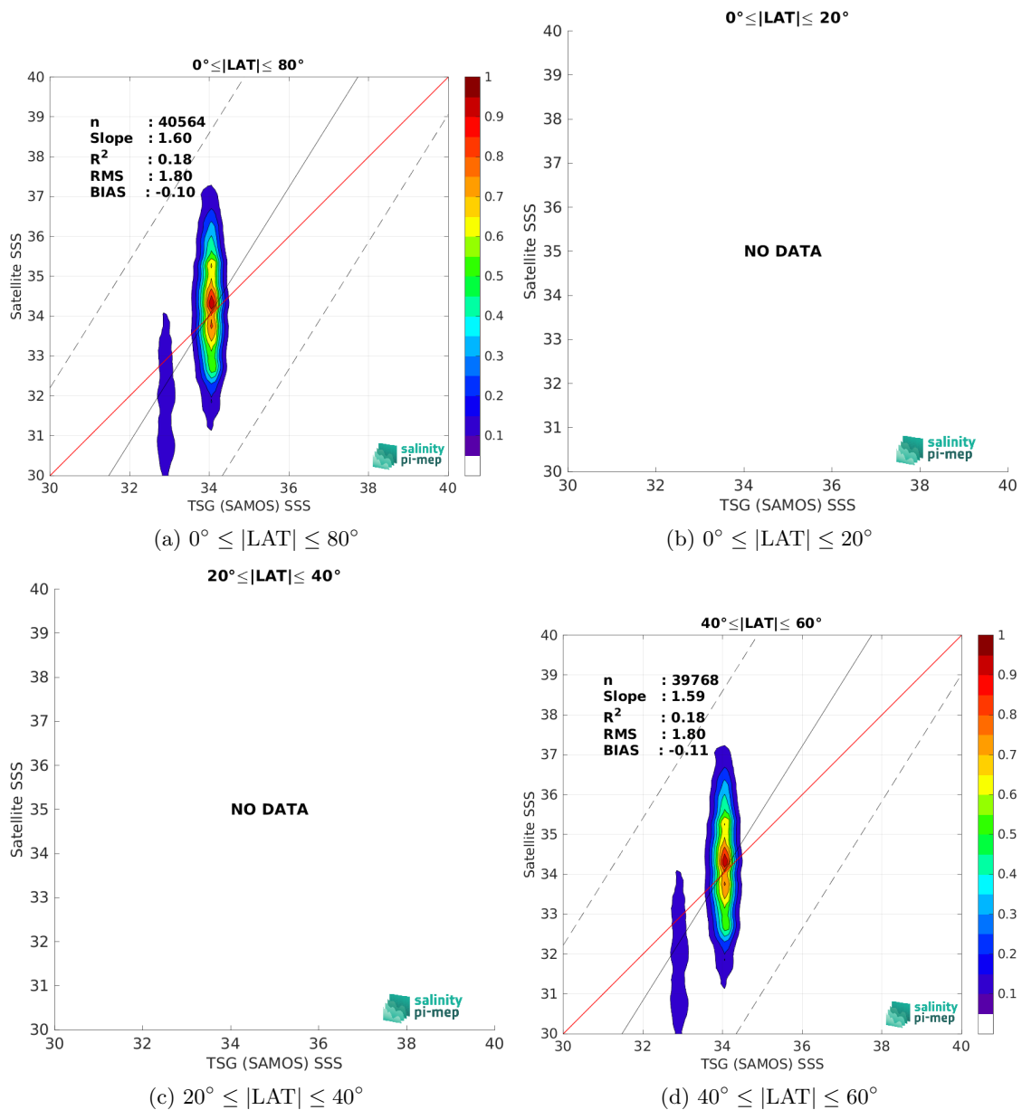
Figure 10: Contour maps of the concentration of SMAP SSS L2 v6 - 40 km (RSS) SSS (y-axis) versus TSG (SAMOS) SSS (x-axis) at match-up pairs for different latitude bands. For each plot, the red line shows x=y . The black thin and dashed lines indicate a linear fit through the data cloud and the \pm 95\% confidence levels, respectively. The number match-up pairs n , the slope and R^2 coefficient of the linear fit, the root mean square (RMS) and the mean bias between satellite and in situ data are indicated for each latitude band in each plot.
