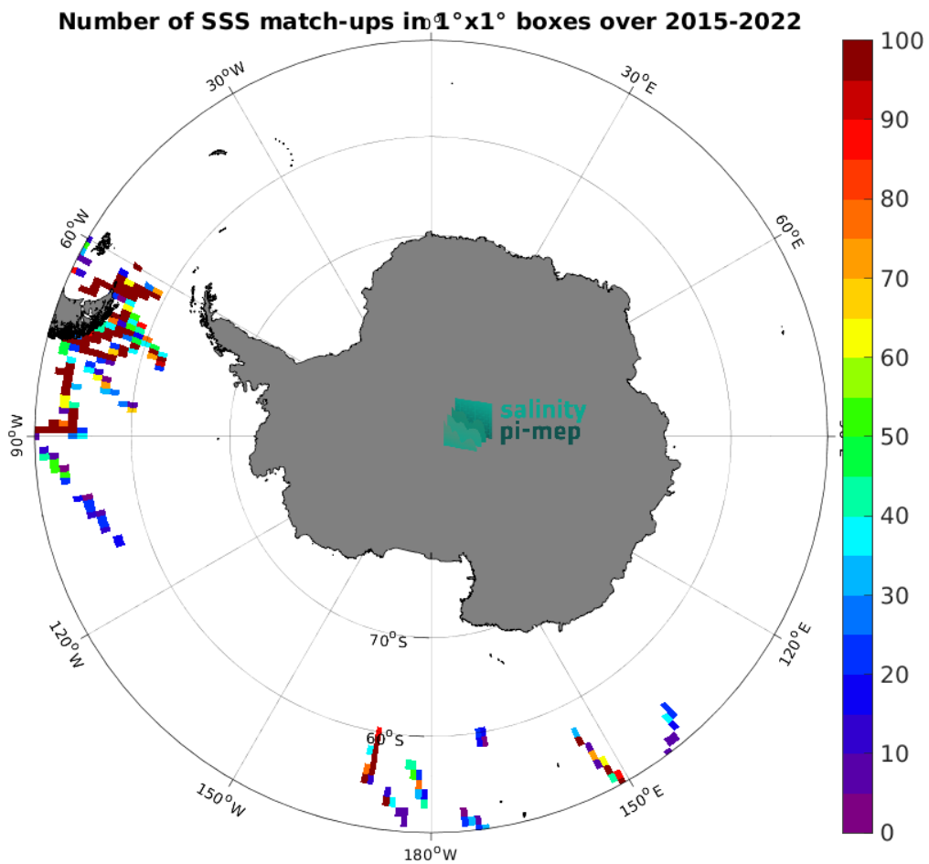
Figure 5: Number of SSS match-ups between TSG (SAMOS) SSS and the SMAP SSS L2 v6 - 40 km (RSS) SSS product for the Southern Ocean Pi-MEP region over 1^\circ \times 1^\circ boxes and for the full satellite product period.
