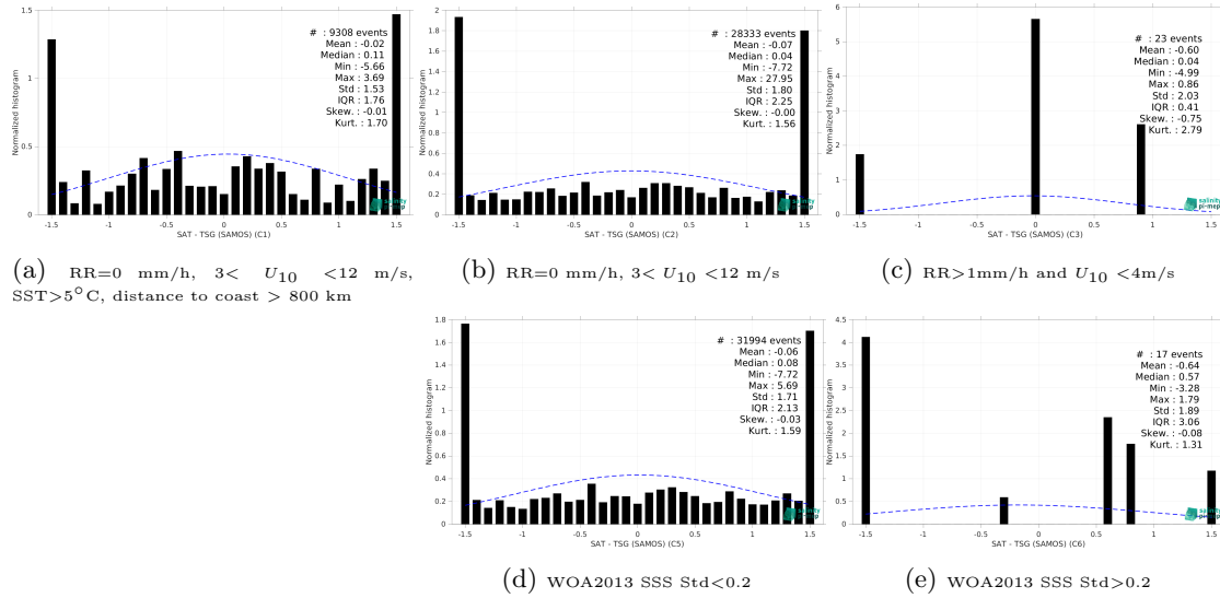
Figure 15: Normalized histogram of \Delta\text{SSS} (SMAP SSS L2 v6 - 40 km (RSS) - TSG (SAMOS)) for 5 different subdatasets corresponding to: RR=0 mm/h, 3 < U_{10} < 12 m/s, SST >5^{\circ}\text{C} , distance to coast > 800 km (a), RR=0 mm/h, 3 < U_{10} < 12 m/s (b), RR>1\text{mm/h} and U_{10} < 4\text{m/s} (c), WOA2013 SSS Std <0.2 (d), WOA2013 SSS Std >0.2 (e).
