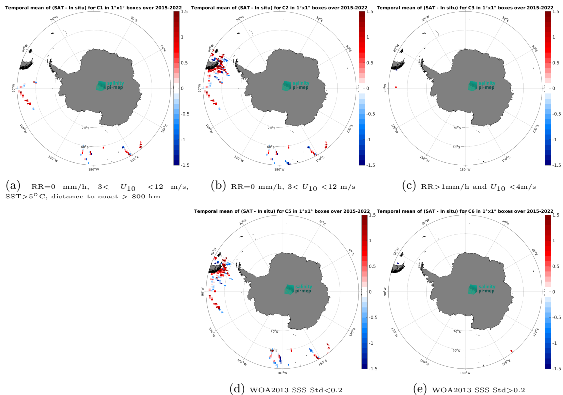
Figure 14: Temporal mean gridded over spatial boxes of size 1^\circ \times 1^\circ of \Delta SSS (SMAP SSS L2 v6 - 40 km (RSS) - TSG (SAMOS)) for 5 different subdatasets corresponding to:RR=0 mm/h, 3 < U_{10} < 12 m/s, SST >5^\circ C, distance to coast > 800 km (a), RR=0 mm/h, 3 < U_{10} < 12 m/s (b), RR >1 mm/h and U_{10} < 4 m/s (c), WOA2013 SSS Std <0.2 (d), WOA2013 SSS Std >0.2 (e).
