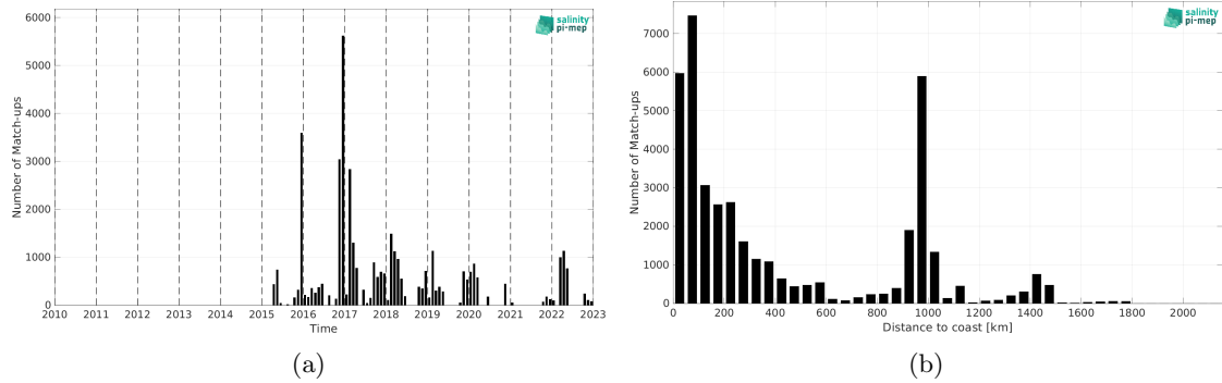
Figure 2: Number of match-ups between TSG (SAMOS) and SMAP SSS L2 v6 - 40 km (RSS) SSS as a function of time (a) and as function of the distance to coast (b) over the Southern Ocean Pi-MEP region and for the full satellite product period.
