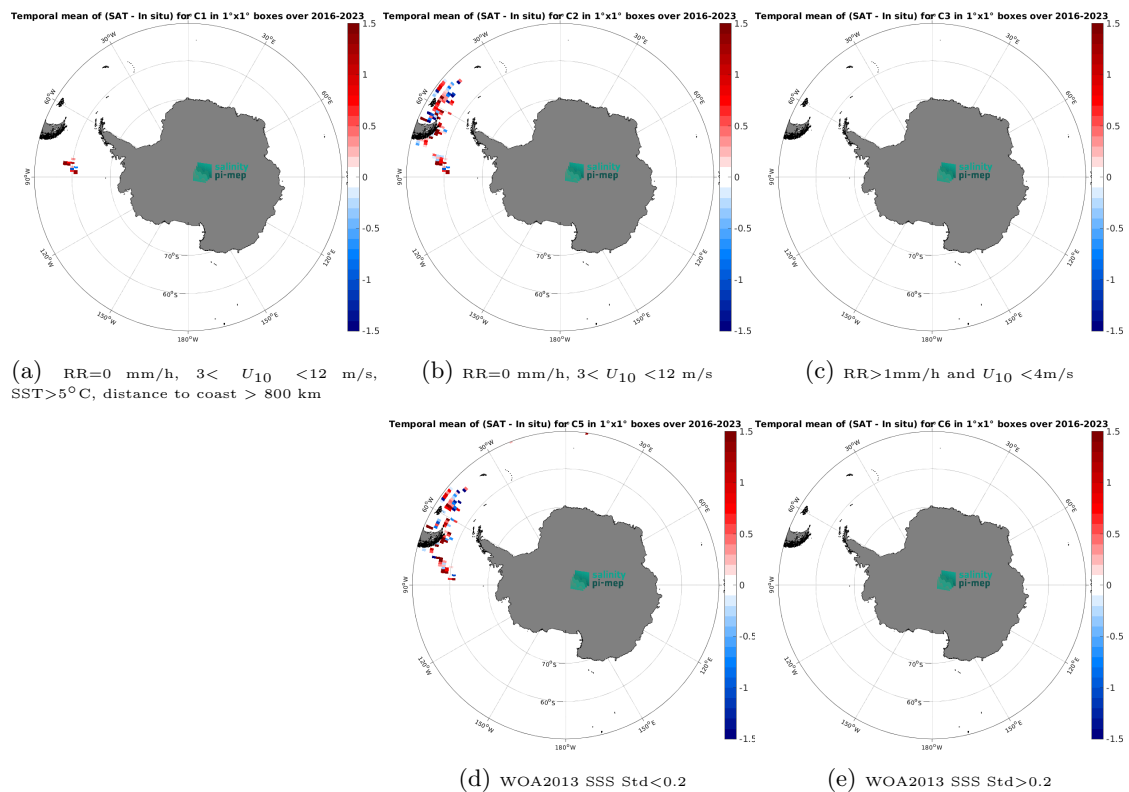
Figure 14: Temporal mean gridded over spatial boxes of size 1^\circ \times 1^\circ of \Delta SSS (SMAP SSS L2 v6 - 40 km (RSS) - TSG (Polarstern)) for 5 different subdatasets corresponding to:RR=0 mm/h, 3 < U_{10} < 12 m/s, SST>5°C, distance to coast > 800 km (a), RR=0 mm/h, 3 < U_{10} < 12 m/s (b), RR>1mm/h and U_{10} < 4 m/s (c), WOA2013 SSS Std<0.2 (d), WOA2013 SSS Std>0.2 (e).
