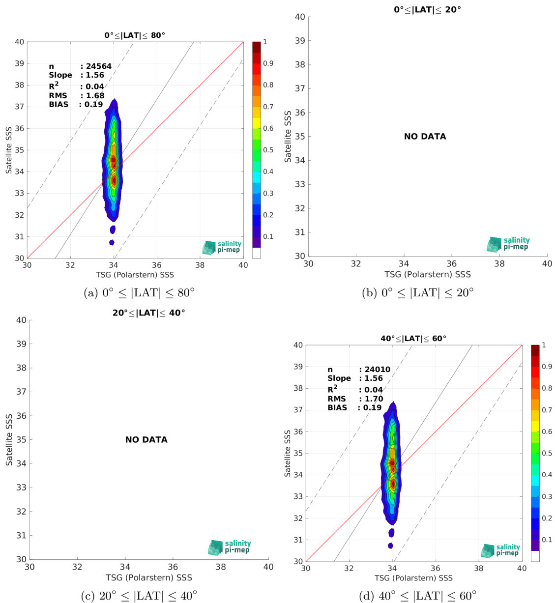
Figure 10: Contour maps of the concentration of SMAP SSS L2 v6 - 40 km (RSS) SSS (y-axis) versus TSG (Polarstern) SSS (x-axis) at match-up pairs for different latitude bands. For each plot, the red line shows x=y . The black thin and dashed lines indicate a linear fit through the data cloud and the \pm 95\% confidence levels, respectively. The number match-up pairs n , the slope and R^2 coefficient of the linear fit, the root mean square (RMS) and the mean bias between satellite and in situ data are indicated for each latitude band in each plot.
