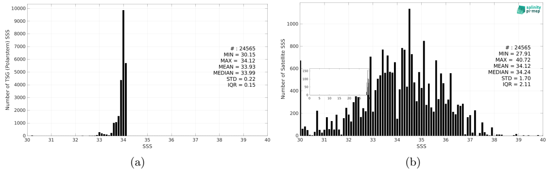
Figure 3: Histograms of SSS from TSG (Polarstern) (a) and SMAP SSS L2 v6 - 40 km (RSS) (b) considering all match-up pairs per bins of 0.1 over the Southern Ocean Pi-MEP region and for the full satellite product period.
