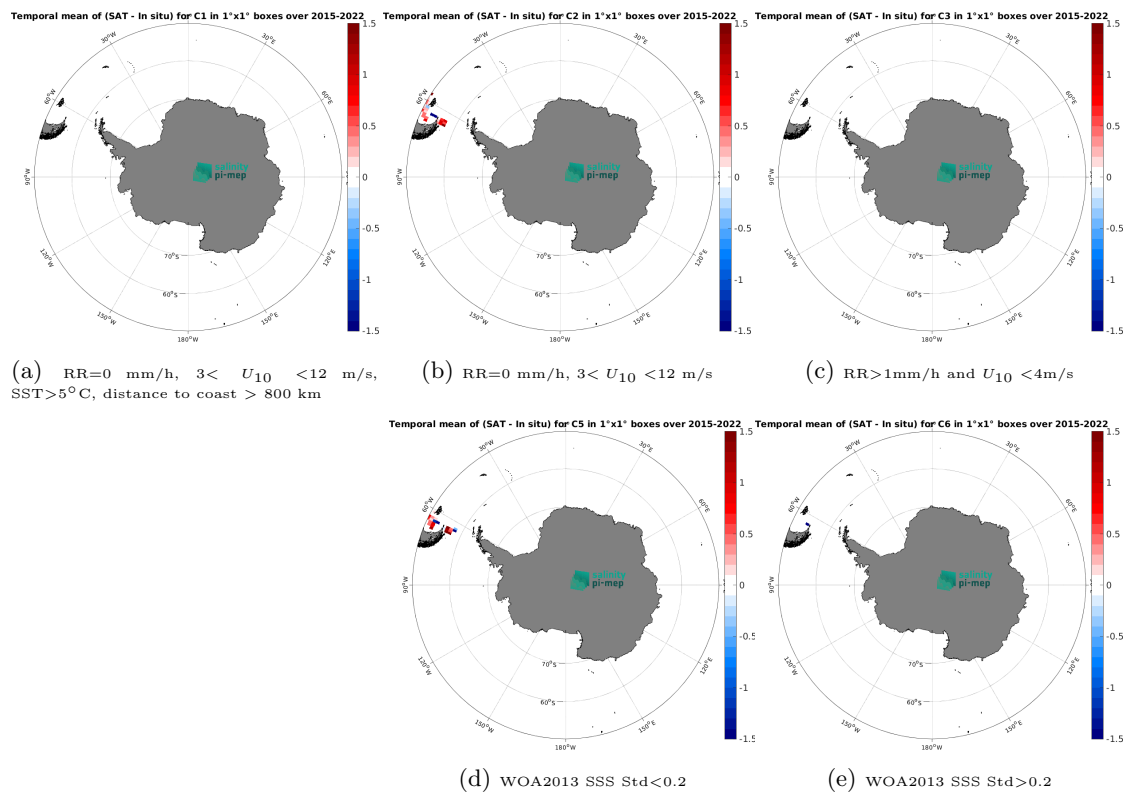
Figure 14: Temporal mean gridded over spatial boxes of size 1^\circ \times 1^\circ of \Delta\text{SSS} (SMAP SSS L2 v6 - 40 km (RSS) - TSG (CSIC-UTM)) for 5 different subdatasets corresponding to: RR=0 mm/h, 3 < U_{10} < 12 m/s, SST > 5°C, distance to coast > 800 km (a), RR=0 mm/h, 3 < U_{10} < 12 m/s (b), RR > 1mm/h and U_{10} < 4 m/s (c), WOA2013 SSS Std < 0.2 (d), WOA2013 SSS Std > 0.2 (e).
