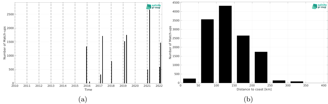
Figure 2: Number of match-ups between TSG (CSIC-UTM) and SMAP SSS L2 v6 - 40 km (RSS) SSS as a function of time (a) and as function of the distance to coast (b) over the Southern Ocean Pi-MEP region and for the full satellite product period.
