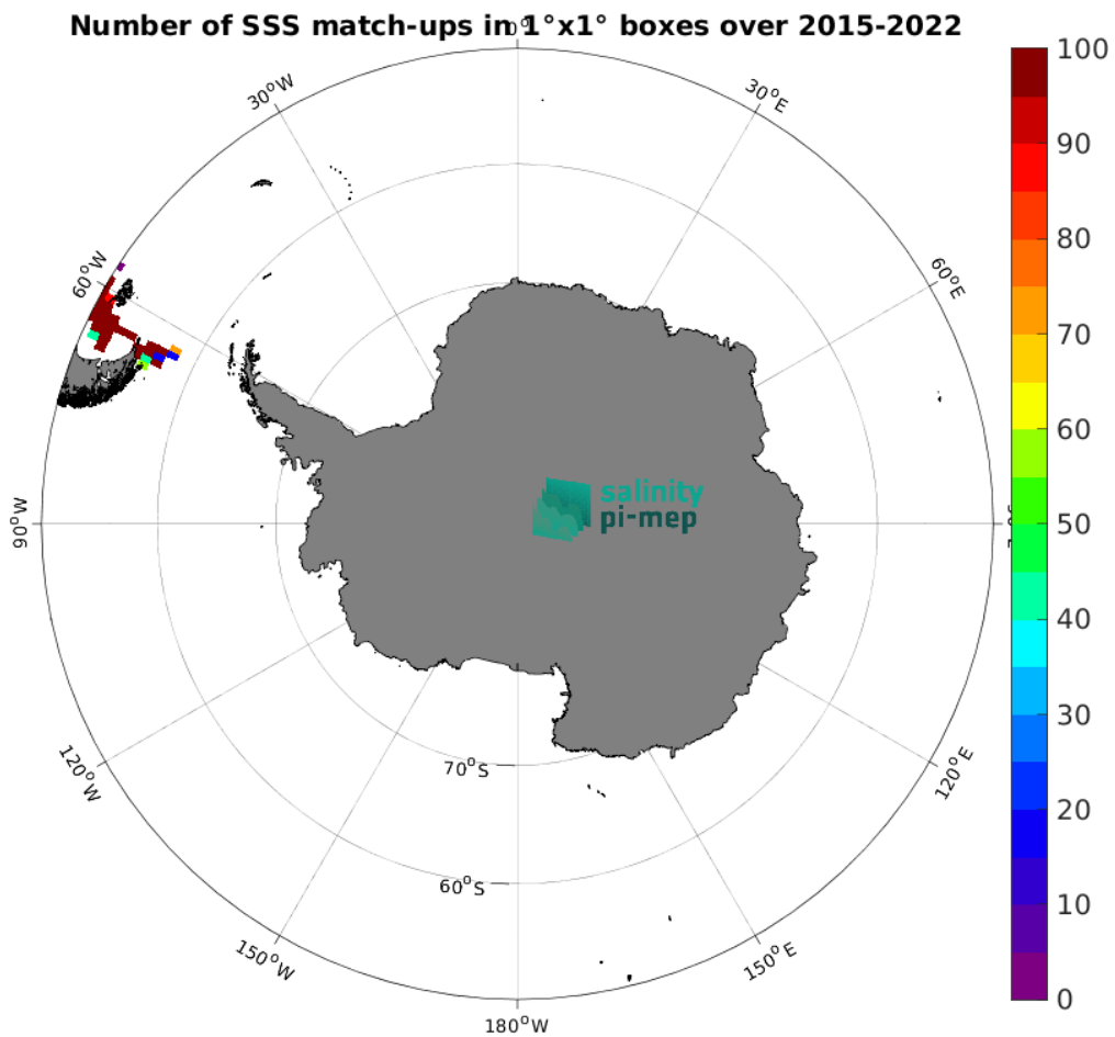
Figure 5: Number of SSS match-ups between TSG (CSIC-UTM) SSS and the SMAP SSS L2 v6 - 40 km (RSS) SSS product for the Southern Ocean Pi-MEP region over 1^\circ \times 1^\circ boxes and for the full satellite product period.
