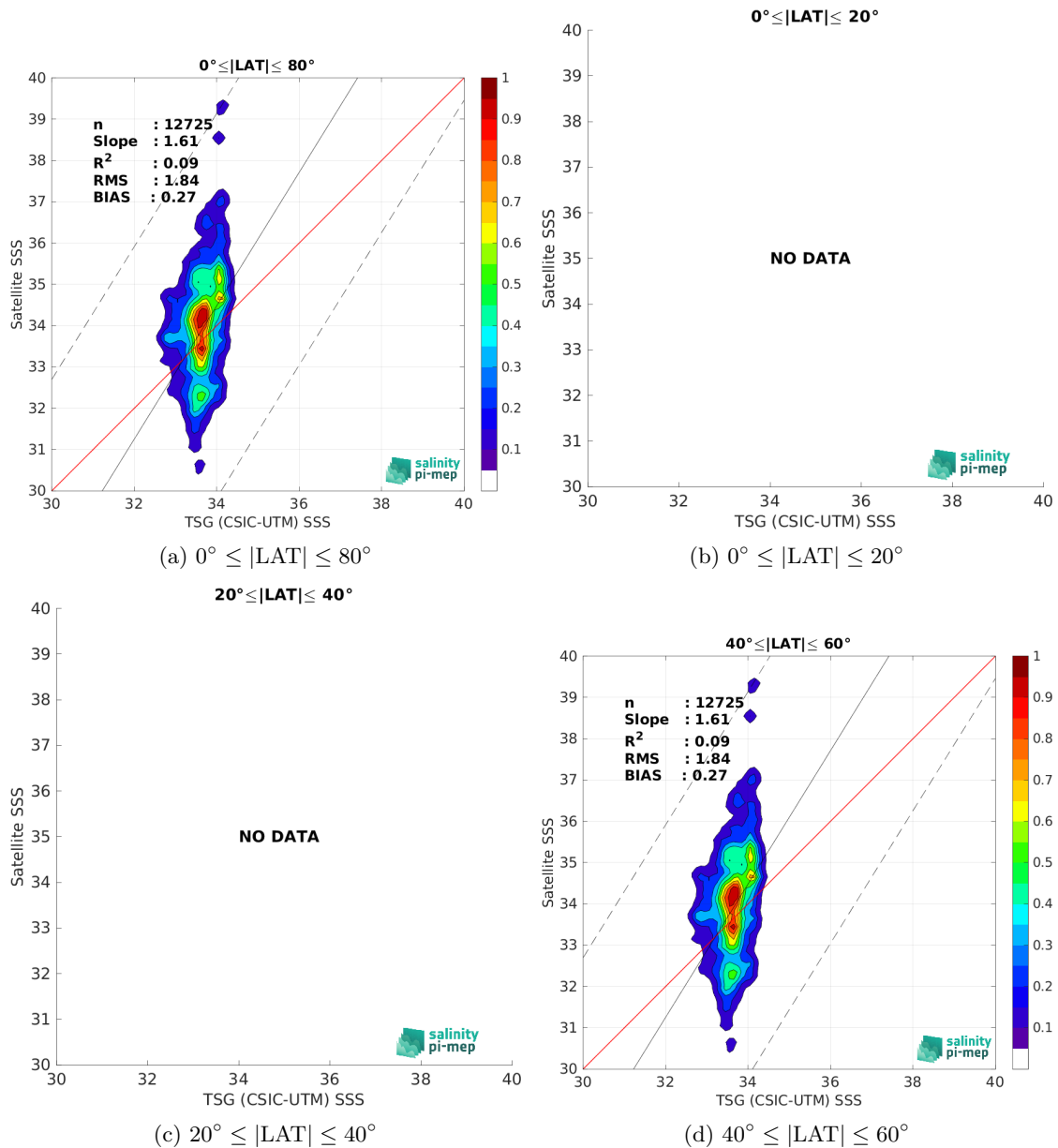
Figure 10: Contour maps of the concentration of SMAP SSS L2 v6 - 40 km (RSS) SSS (y-axis) versus TSG (CSIC-UTM) SSS (x-axis) at match-up pairs for different latitude bands. For each plot, the red line shows x=y . The black thin and dashed lines indicate a linear fit through the data cloud and the \pm 95\% confidence levels, respectively. The number match-up pairs n , the slope and R^2 coefficient of the linear fit, the root mean square (RMS) and the mean bias between satellite and in situ data are indicated for each latitude band in each plots.
