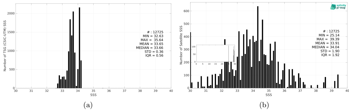
Figure 3: Histograms of SSS from TSG (CSIC-UTM) (a) and SMAP SSS L2 v6 - 40 km (RSS) (b) considering all match-up pairs per bins of 0.1 over the Southern Ocean Pi-MEP region and for the full satellite product period.
