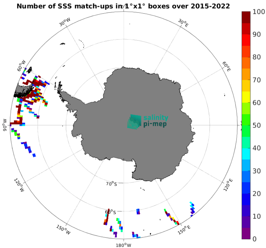
Figure 4: Number of SSS match-ups between TSG (SAMOS) SSS and the SMAP SSS L2 v5 (RSS) SSS product for the Southern Ocean Pi-MEP region over 1^\circ \times 1^\circ boxes and for the full satellite product period.
