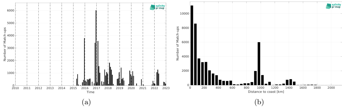
Figure 1: Number of match-ups between TSG (SAMOS) and SMAP SSS L2 v5 (RSS) SSS as a function of time (a) and as function of the distance to coast (b) over the Southern Ocean Pi-MEP region and for the full satellite product period.
