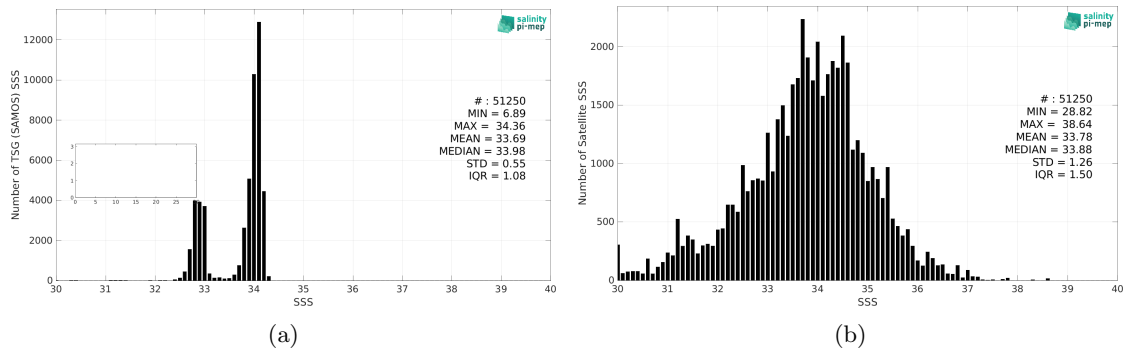
Figure 2: Histograms of SSS from TSG (SAMOS) (a) and SMAP SSS L2 v5 (RSS) (b) considering all match-up pairs per bins of 0.1 over the Southern Ocean Pi-MEP region and for the full satellite product period.
