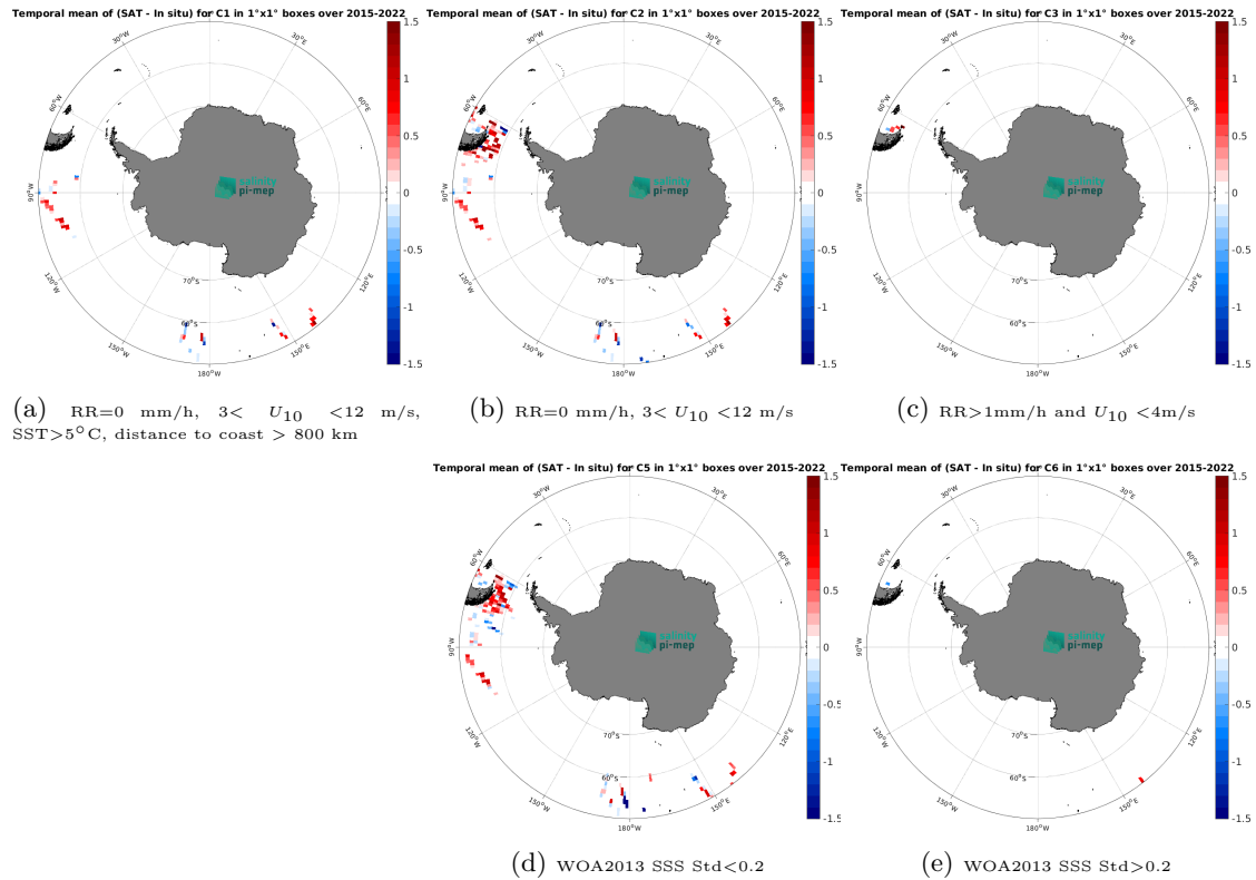
Figure 12: Temporal mean gridded over spatial boxes of size 1^{\circ}\times 1^{\circ} of \Delta\text{SSS} (SMAP SSS L2 v5 (RSS) - TSG (SAMOS)) for 5 different subdatasets corresponding to: \text{RR}=0 mm/h, 3 < U_{10} < 12 m/s, \text{SST}>5^{\circ}\text{C} , distance to coast > 800 km (a), \text{RR}=0 mm/h, 3 < U_{10} < 12 m/s (b), \text{RR}>1 mm/h and U_{10} < 4 m/s (c), WOA2013 SSS Std < 0.2 (d), WOA2013 SSS Std > 0.2 (e).
