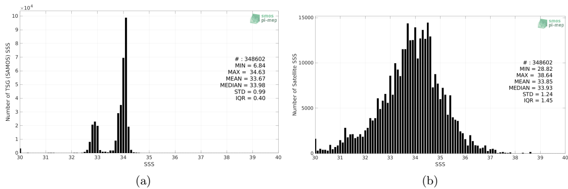
Figure 2: Histograms of SSS from TSG (SAMOS) (a) and SMAP SSS L2 v5 (RSS) (b) considering all match-up pairs per bins of 0.1 over the Southern Ocean Pi-MEP region and for the full satellite product period.
