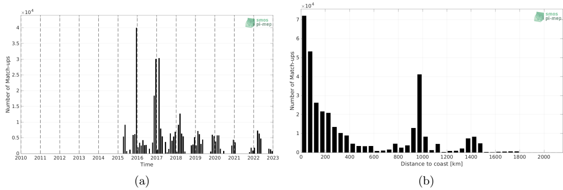
Figure 1: Number of match-ups between TSG (SAMOS) and SMAP SSS L2 v5 (RSS) SSS as a function of time (a) and as function of the distance to coast (b) over the Southern Ocean Pi-MEP region and for the full satellite product period.
