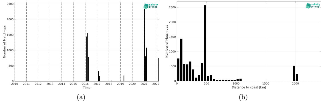
Figure 1: Number of match-ups between TSG (Polarstern) and SMAP SSS L2 v5 (RSS) SSS as a function of time (a) and as function of the distance to coast (b) over the Southern Ocean Pi-MEP region and for the full satellite product period.
