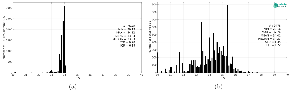
Figure 2: Histograms of SSS from TSG (Polarstern) (a) and SMAP SSS L2 v5 (RSS) (b) considering all match-up pairs per bins of 0.1 over the Southern Ocean Pi-MEP region and for the full satellite product period.
