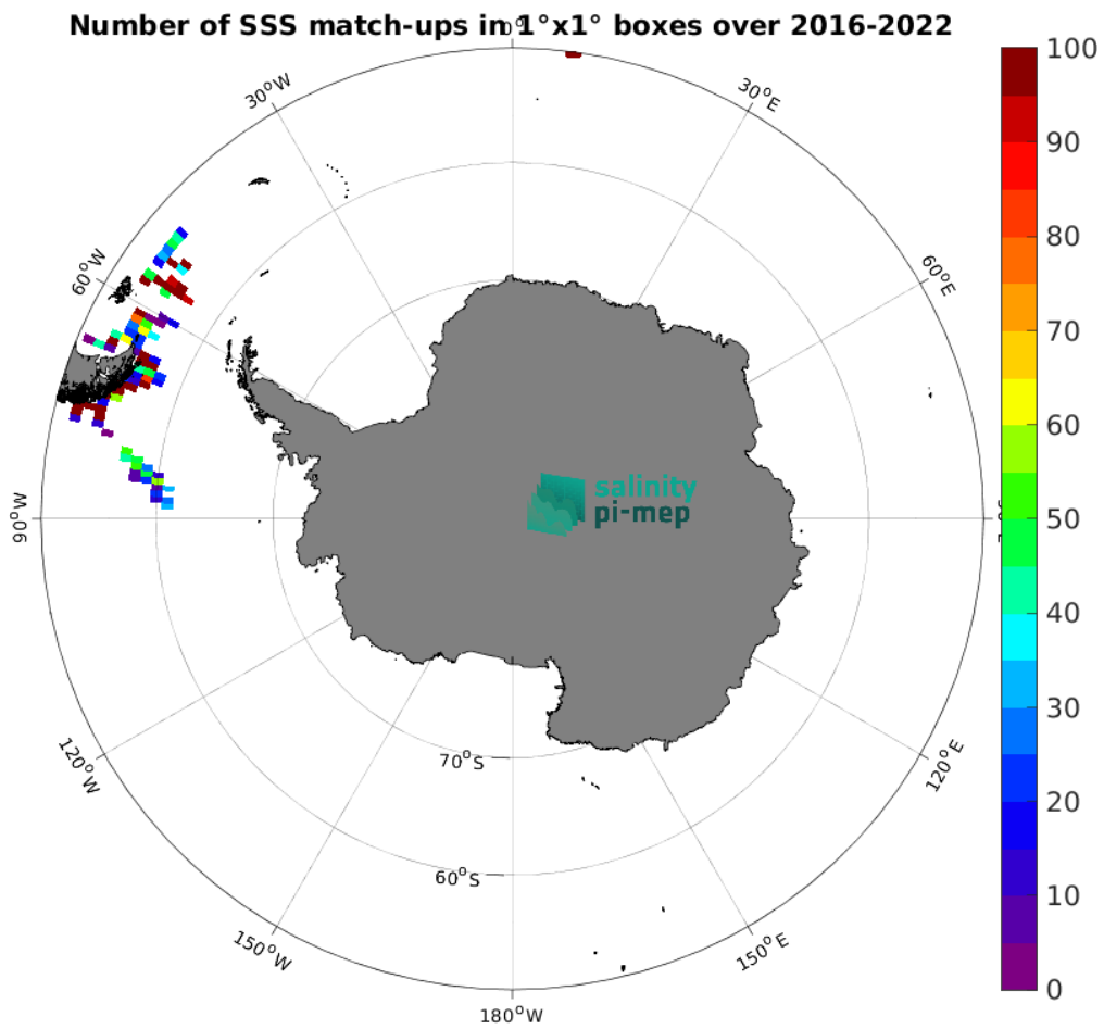
Figure 4: Number of SSS match-ups between TSG (Polarstern) SSS and the SMAP SSS L2 v5 (RSS) SSS product for the Southern Ocean Pi-MEP region over 1^\circ \times 1^\circ boxes and for the full satellite product period.
