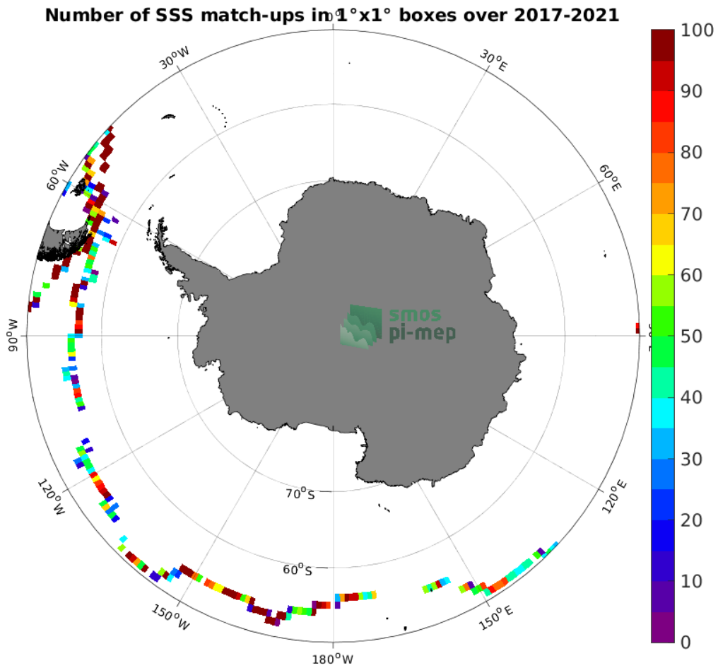
Figure 4: Number of SSS match-ups between TSG (GOSUD-Sailing-ship) SSS and the SMAP SSS L2 v5 (RSS) SSS product for the Southern Ocean Pi-MEP region over 1^\circ \times 1^\circ boxes and for the full satellite product period.
