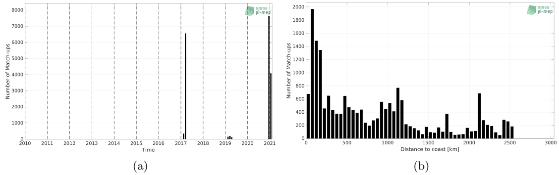
Figure 1: Number of match-ups between TSG (GOSUD-Sailing-ship) and SMAP SSS L2 v5 (RSS) SSS as a function of time (a) and as function of the distance to coast (b) over the Southern Ocean Pi-MEP region and for the full satellite product period.
