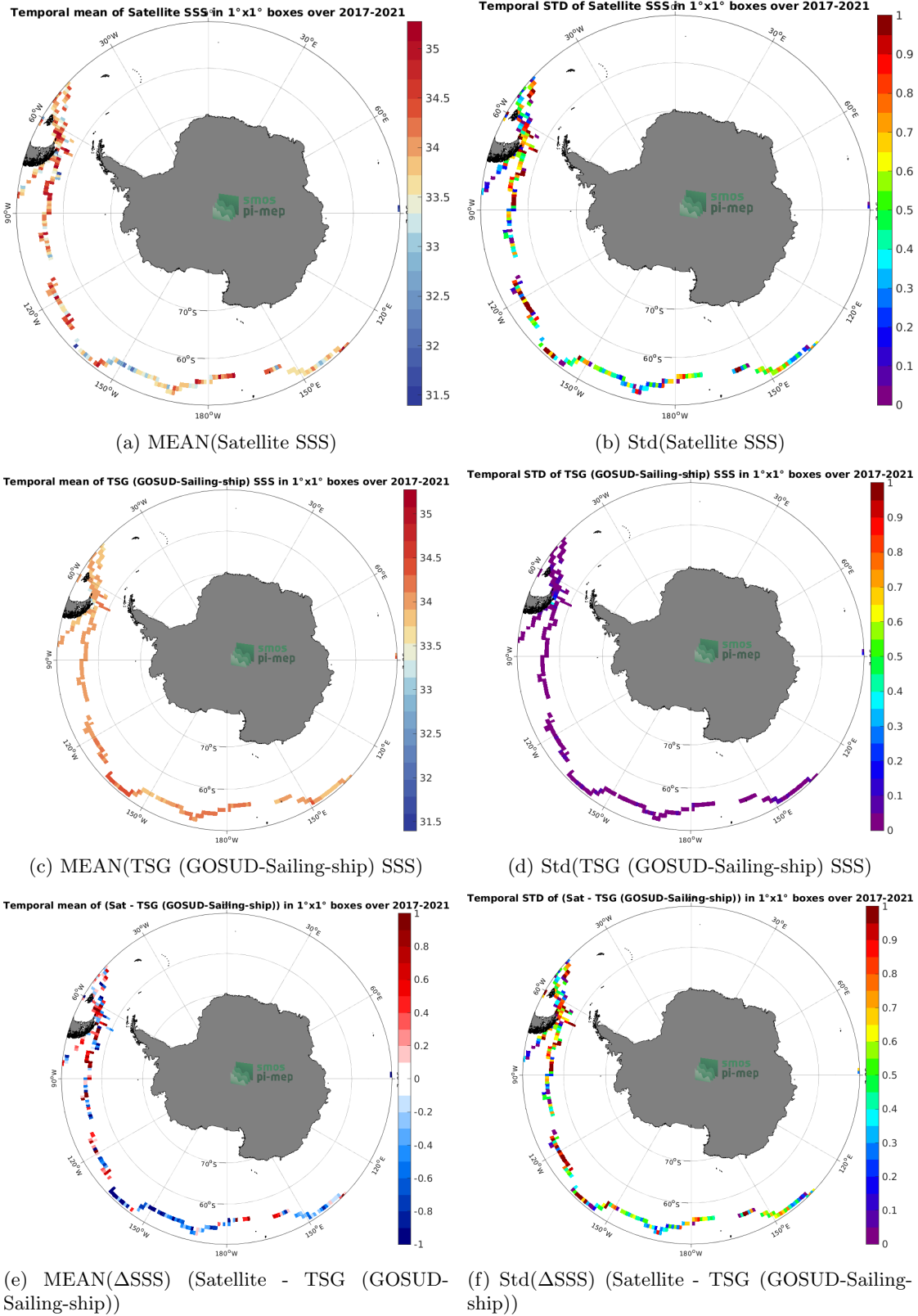
Figure 6: Temporal mean (left) and Std (right), of SSS from SMAP SSS L2 v5 (RSS) (top), TSG (GOSUD-Sailing-ship) (middle), and of \Delta SSS (Satellite - TSG (GOSUD-Sailing-ship)). Only match-up pairs are used to generate these maps.
