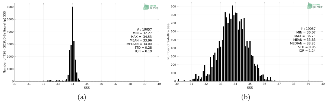
Figure 2: Histograms of SSS from TSG (GOSUD-Sailing-ship) (a) and SMAP SSS L2 v5 (RSS) (b) considering all match-up pairs per bins of 0.1 over the Southern Ocean Pi-MEP region and for the full satellite product period.
