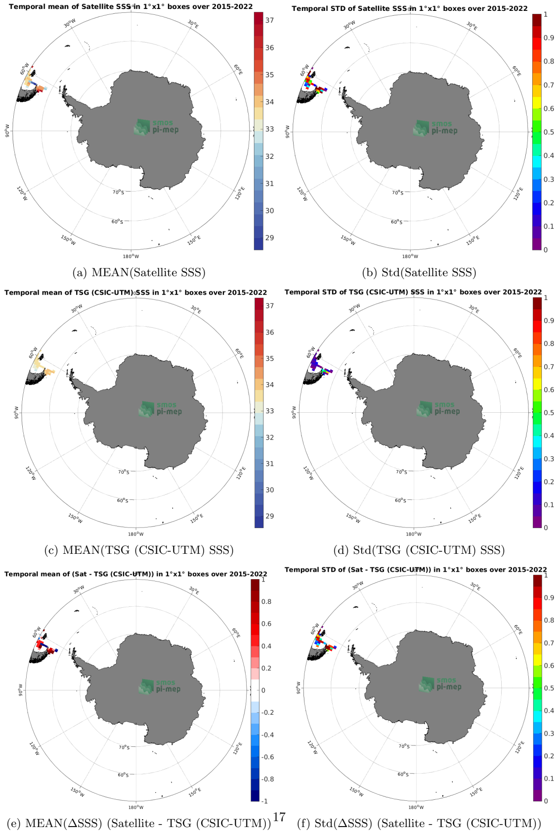
Figure 6: Temporal mean (left) and Std (right) of SSS from SMAP SSS L2 v5 (RSS) (top), TSG (CSIC-UTM) (middle), and of \Delta SSS (Satellite - TSG (CSIC-UTM)). Only match-up pairs are used to generate these maps.
