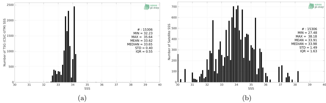
Figure 2: Histograms of SSS from TSG (CSIC-UTM) (a) and SMAP SSS L2 v5 (RSS) (b) considering all match-up pairs per bins of 0.1 over the Southern Ocean Pi-MEP region and for the full satellite product period.
