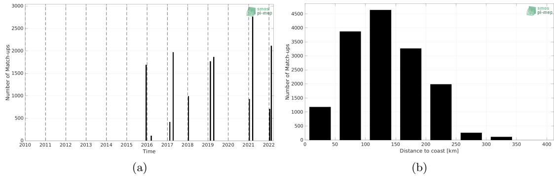
Figure 1: Number of match-ups between TSG (CSIC-UTM) and SMAP SSS L2 v5 (RSS) SSS as a function of time (a) and as function of the distance to coast (b) over the Southern Ocean Pi-MEP region and for the full satellite product period.
