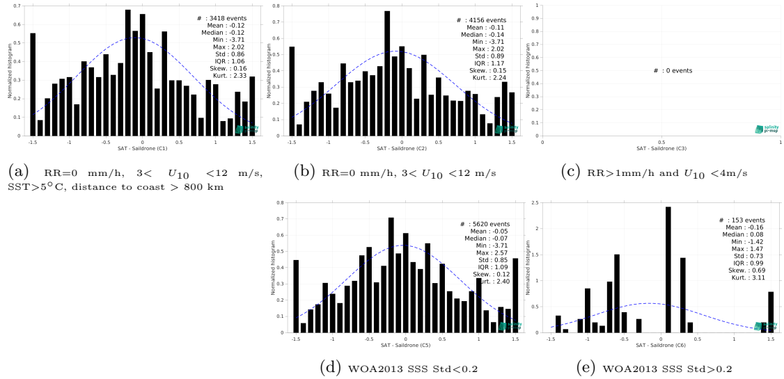
Figure 13: Normalized histogram of \Delta SSS (SMAP SSS L2 v5 (RSS) - Saildrone) for 5 different subdatasets corresponding to: RR=0 mm/h, 3 < U_{10} < 12 m/s, SST > 5°C, distance to coast > 800 km (a), RR=0 mm/h, 3 < U_{10} < 12 m/s (b), RR > 1mm/h and U_{10} < 4 m/s (c), WOA2013 SSS Std < 0.2 (d), WOA2013 SSS Std > 0.2 (e).
