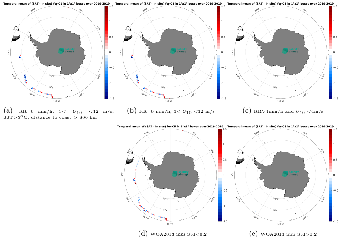
Figure 12: Temporal mean gridded over spatial boxes of size 1^{\circ}\times 1^{\circ} of \Delta\text{SSS} (SMAP SSS L2 v5 (RSS) - Saildrone) for 5 different subdatasets corresponding to: \text{RR}=0 mm/h, 3 < U_{10} < 12 m/s, \text{SST}>5^{\circ}\text{C} , distance to coast > 800 km (a), \text{RR}=0 mm/h, 3 < U_{10} < 12 m/s (b), \text{RR}>1 mm/h and U_{10} < 4 m/s (c), WOA2013 SSS Std <0.2 (d), WOA2013 SSS Std >0.2 (e).
