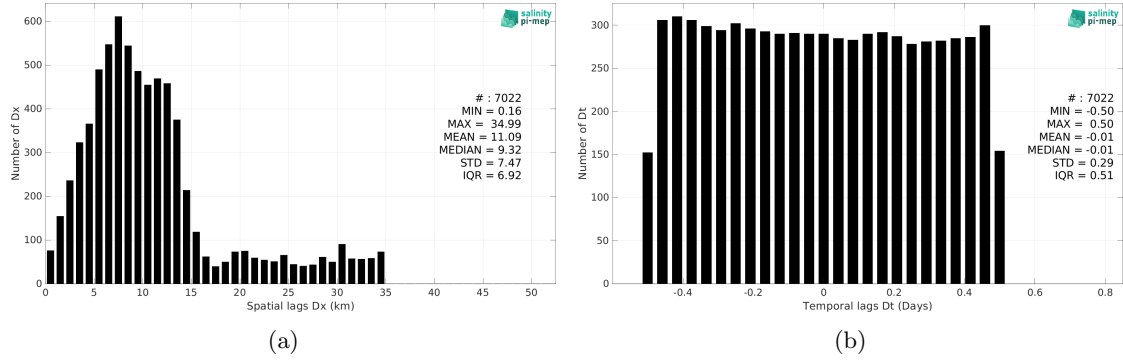
Figure 5: Histograms of the spatial (a) and temporal (b) lags between the location/time of the Saildrone measurement and the date of the corresponding SMAP SSS L2 v5 (RSS) SSS pixel.
