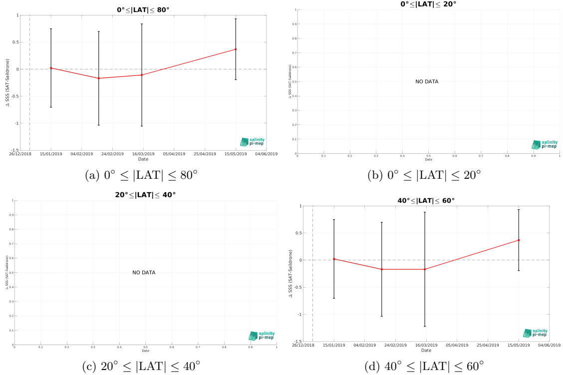
Figure 10: Monthly median (red curves) of \Delta SSS (Satellite - Sairdrone) and \pm 1 Std (black vertical thick bars) as function of time for all the collected Pi-MEP match-up pairs estimated over the Southern Ocean Pi-MEP region and for the full satellite product period are shown for different latitude bands: (a) 80^\circ\text{S}-80^\circ\text{N} , (b) 20^\circ\text{S}-20^\circ\text{N} , (c) 40^\circ\text{S}-20^\circ\text{S} and 20^\circ\text{N}-40^\circ\text{N} and (d) 60^\circ\text{S}-40^\circ\text{S} and 40^\circ\text{N}-60^\circ\text{N} .
