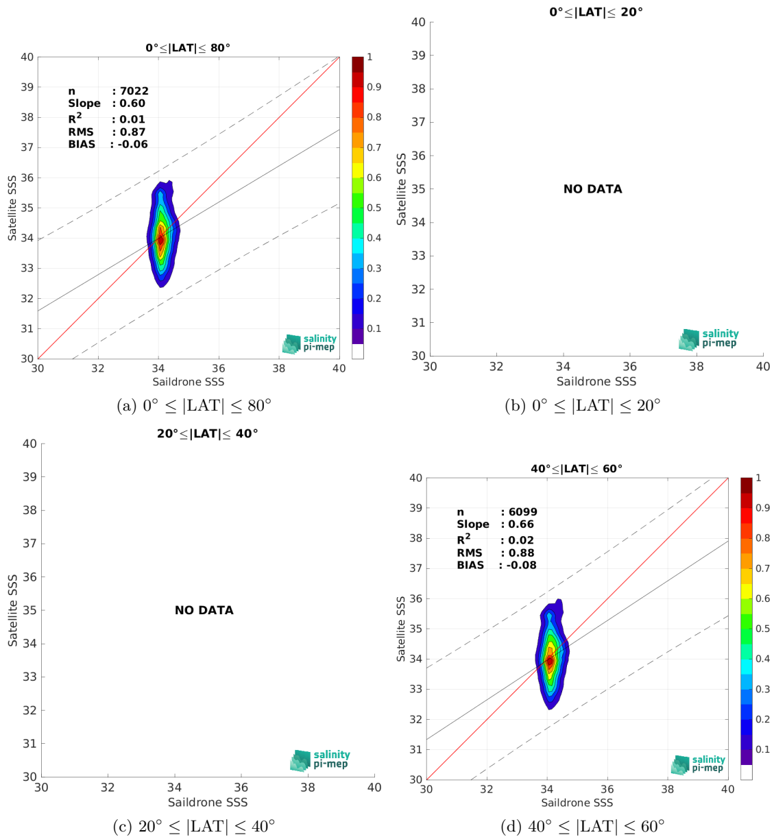
Figure 9: Contour maps of the concentration of SMAP SSS L2 v5 (RSS) SSS (y-axis) versus Saildrone SSS (x-axis) at match-up pairs for different latitude bands. For each plot, the red line shows x=y . The black thin and dashed lines indicate a linear fit through the data cloud and the \pm 95\% confidence levels, respectively. The number match-up pairs n , the slope and R^2 coefficient of the linear fit, the root mean square (RMS) and the mean bias between satellite and in situ data are indicated for each latitude band in each plots.
