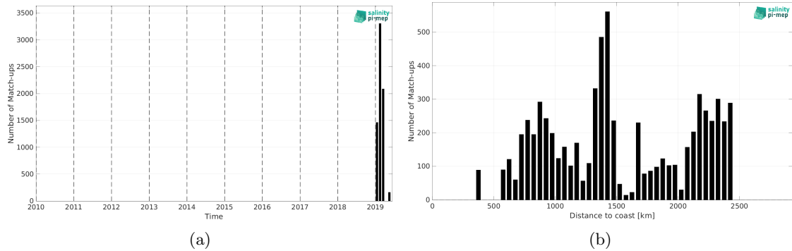
Figure 1: Number of match-ups between Saildrone and SMAP SSS L2 v5 (RSS) SSS as a function of time (a) and as function of the distance to coast (b) over the Southern Ocean Pi-MEP region and for the full satellite product period.
