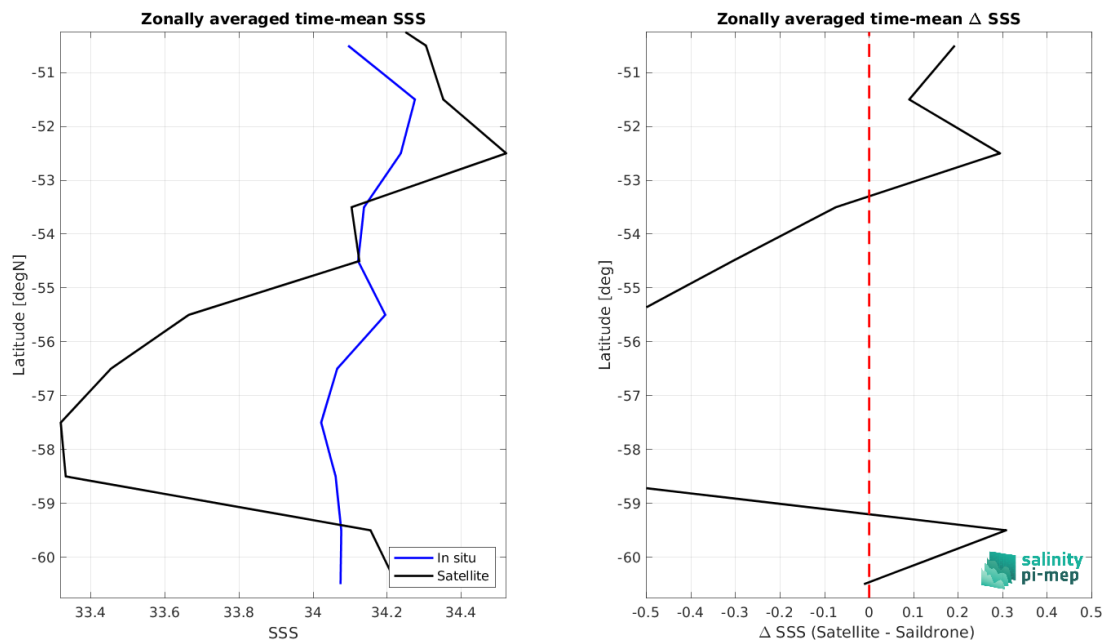
Figure 8: Left panel: Zonal mean SSS from SMAP SSS L2 v5 (RSS) satellite product (black) and from Sairdrone (blue). Right panel: Zonal mean of \Delta SSS (Satellite - Sairdrone) for all the collected Pi-MEP match-up pairs estimated over the full satellite product period.
