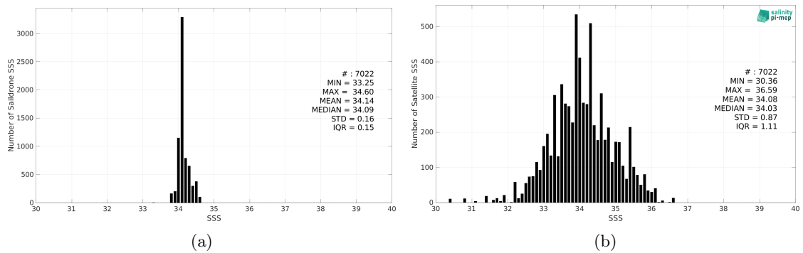
Figure 2: Histograms of SSS from Saildrone (a) and SMAP SSS L2 v5 (RSS) (b) considering all match-up pairs per bins of 0.1 over the Southern Ocean Pi-MEP region and for the full satellite product period.
