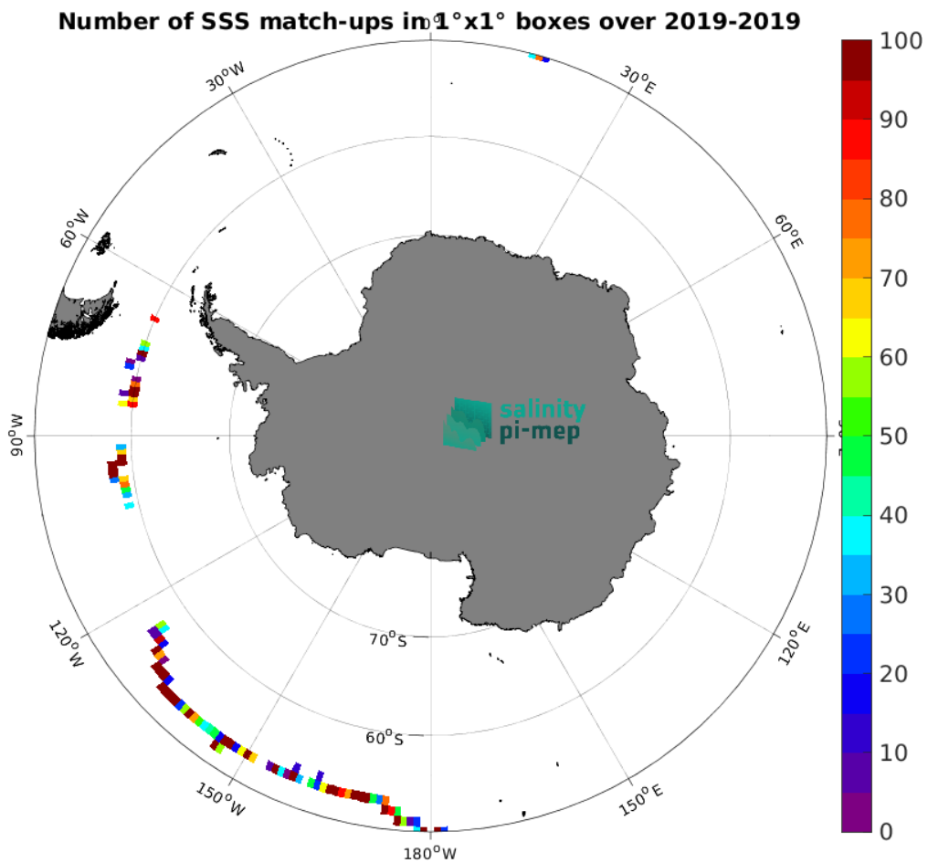
Figure 4: Number of SSS match-ups between Saildrone SSS and the SMAP SSS L2 v5 (RSS) SSS product for the Southern Ocean Pi-MEP region over 1^\circ \times 1^\circ boxes and for the full satellite product period.
