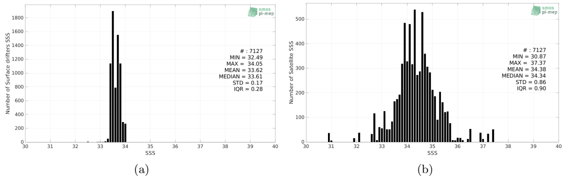
Figure 2: Histograms of SSS from Surface drifters (a) and SMAP SSS L2 v5 (RSS) (b) considering all match-up pairs per bins of 0.1 over the Southern Ocean Pi-MEP region and for the full satellite product period.
