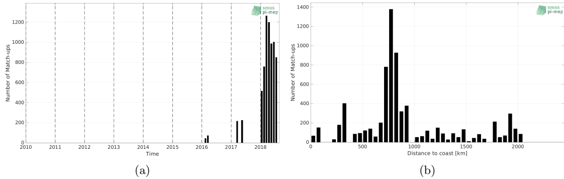
Figure 1: Number of match-ups between Surface drifters and SMAP SSS L2 v5 (RSS) SSS as a function of time (a) and as function of the distance to coast (b) over the Southern Ocean Pi-MEP region and for the full satellite product period.
