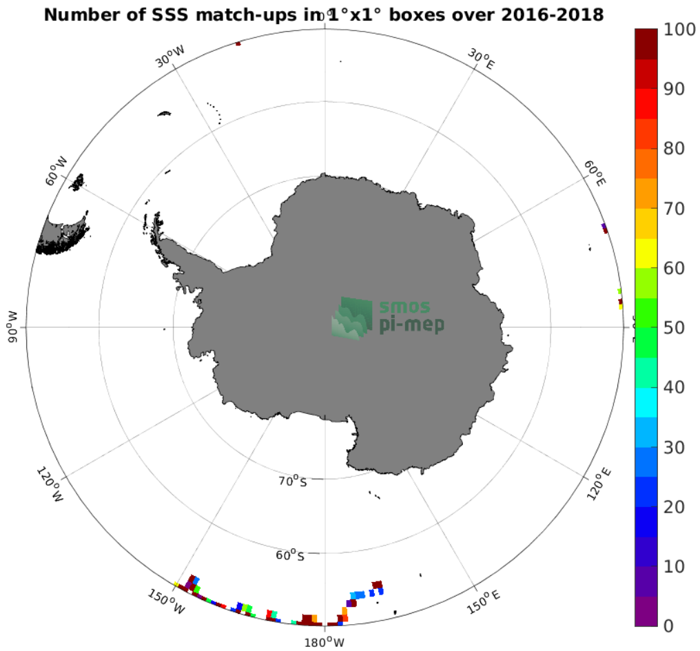
Figure 3: Number of SSS match-ups between Surface drifters SSS and the SMAP SSS L2 v5 (RSS) SSS product for the Southern Ocean Pi-MEP region over 1^\circ \times 1^\circ boxes and for the full satellite product period.
