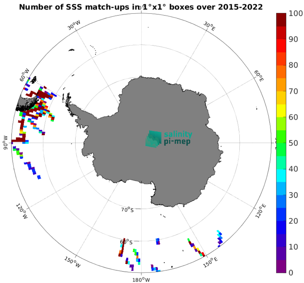
Figure 5: Number of SSS match-ups between TSG (SAMOS) SSS and the SMAP SSS L2 v5.3 (RSS) SSS product for the Southern Ocean Pi-MEP region over 1^\circ \times 1^\circ boxes and for the full satellite product period.
