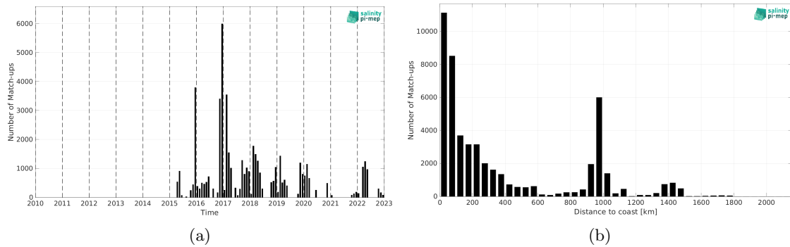
Figure 2: Number of match-ups between TSG (SAMOS) and SMAP SSS L2 v5.3 (RSS) SSS as a function of time (a) and as function of the distance to coast (b) over the Southern Ocean Pi-MEP region and for the full satellite product period.
