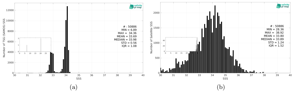
Figure 3: Histograms of SSS from TSG (SAMOS) (a) and SMAP SSS L2 v5.3 (RSS) (b) considering all match-up pairs per bins of 0.1 over the Southern Ocean Pi-MEP region and for the full satellite product period.
