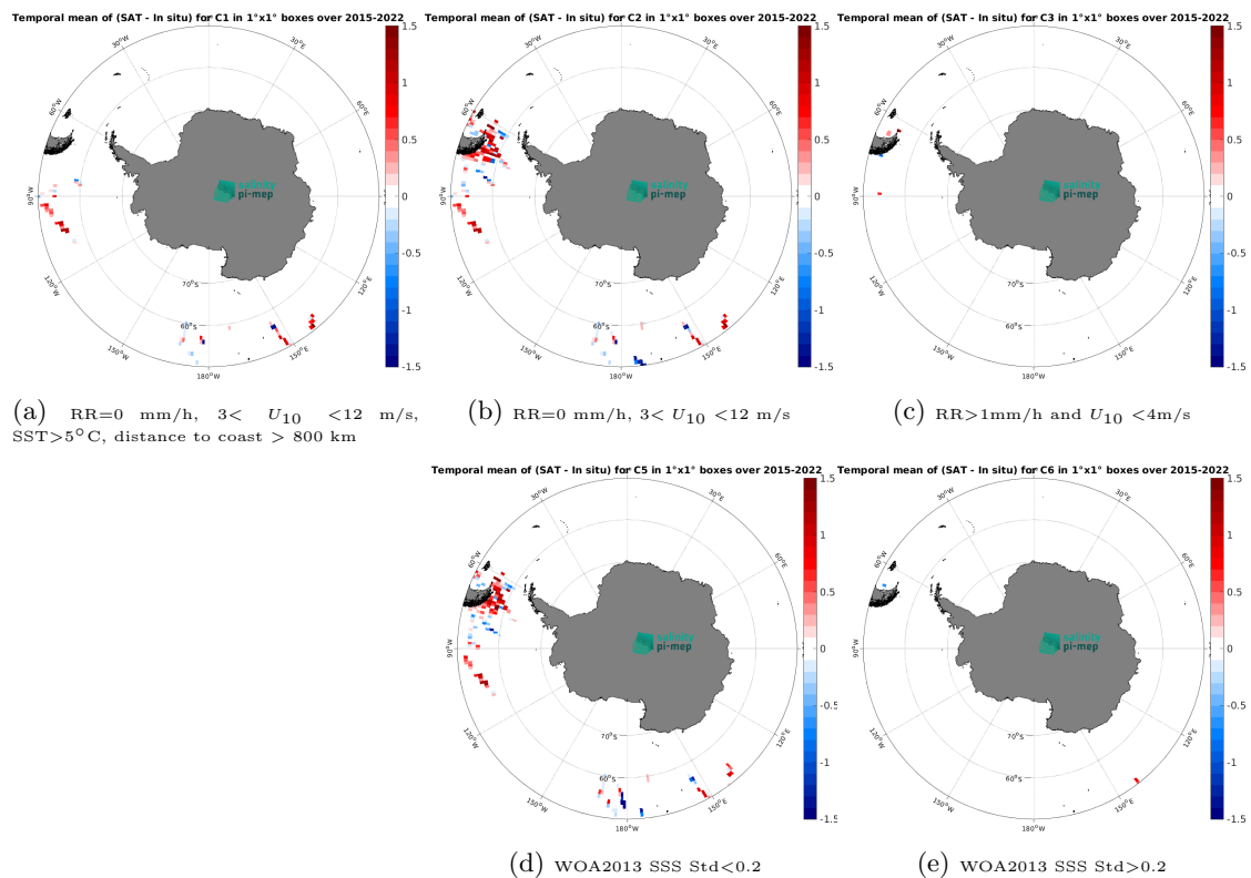
Figure 14: Temporal mean gridded over spatial boxes of size 1^\circ \times 1^\circ of \Delta\text{SSS} (SMAP SSS L2 v5.3 (RSS) - TSG (SAMOS)) for 5 different subdatasets corresponding to:RR=0 mm/h, 3 < U_{10} < 12 m/s, SST>5°C, distance to coast > 800 km (a), RR=0 mm/h, 3 < U_{10} < 12 m/s (b), RR>1mm/h and U_{10} < 4 m/s (c), WOA2013 SSS Std<0.2 (d), WOA2013 SSS Std>0.2 (e).
