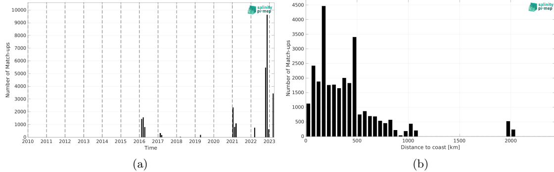
Figure 2: Number of match-ups between TSG (Polarstern) and SMAP SSS L2 v5.3 (RSS) SSS as a function of time (a) and as function of the distance to coast (b) over the Southern Ocean Pi-MEP region and for the full satellite product period.
