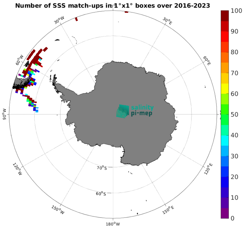
Figure 5: Number of SSS match-ups between TSG (Polarstern) SSS and the SMAP SSS L2 v5.3 (RSS) SSS product for the Southern Ocean Pi-MEP region over 1^\circ \times 1^\circ boxes and for the full satellite product period.
