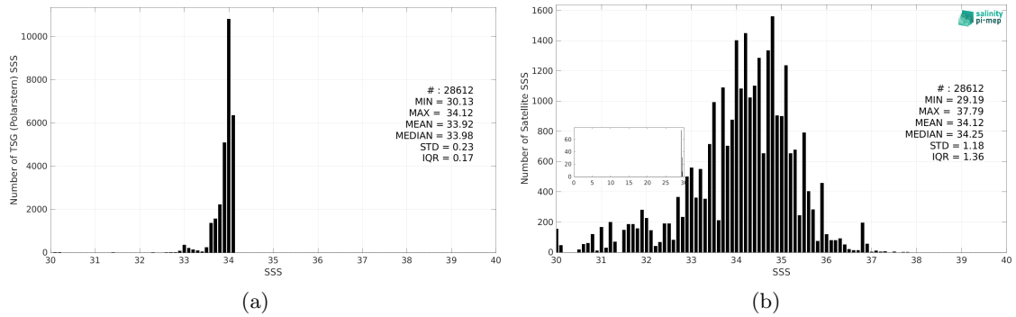
Figure 3: Histograms of SSS from TSG (Polarstern) (a) and SMAP SSS L2 v5.3 (RSS) (b) considering all match-up pairs per bins of 0.1 over the Southern Ocean Pi-MEP region and for the full satellite product period.
