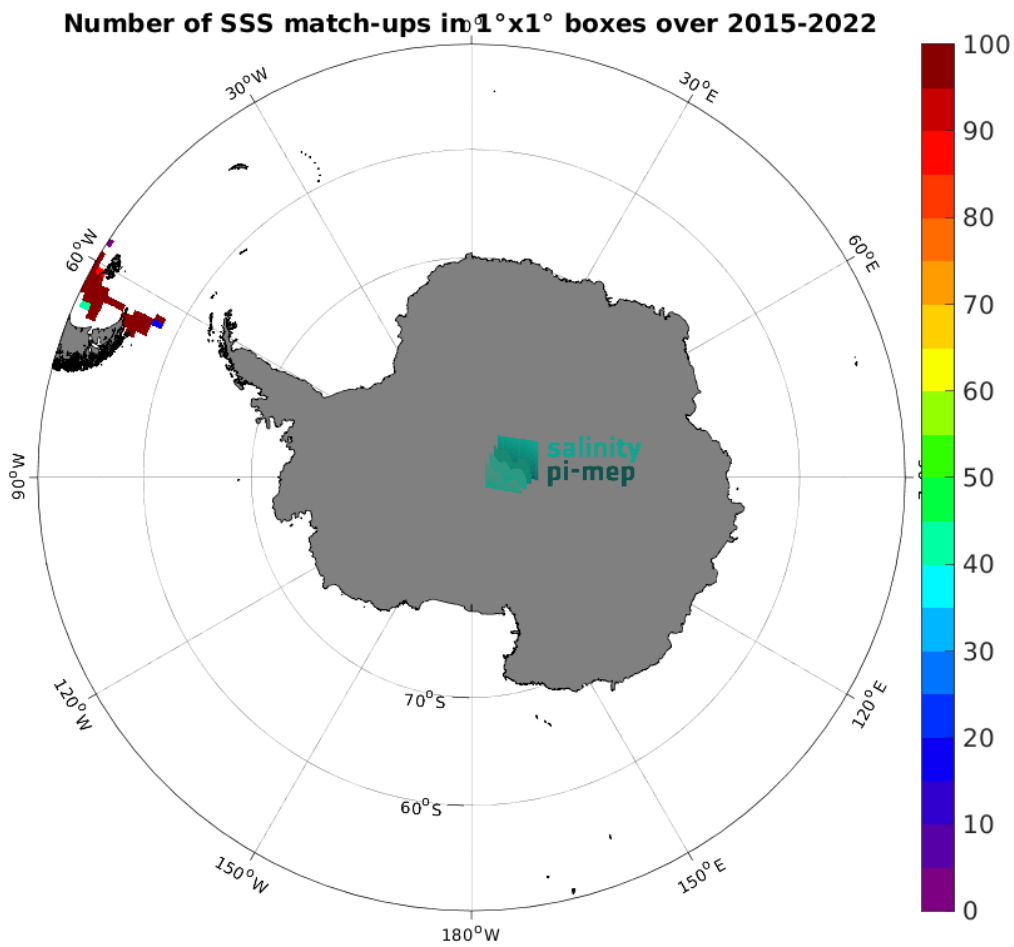
Figure 5: Number of SSS match-ups between TSG (CSIC-UTM) SSS and the SMAP SSS L2 v5.3 (RSS) SSS product for the Southern Ocean Pi-MEP region over 1^\circ \times 1^\circ boxes and for the full satellite product period.
