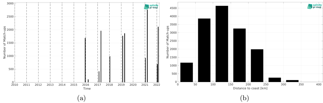
Figure 2: Number of match-ups between TSG (CSIC-UTM) and SMAP SSS L2 v5.3 (RSS) SSS as a function of time (a) and as function of the distance to coast (b) over the Southern Ocean Pi-MEP region and for the full satellite product period.
