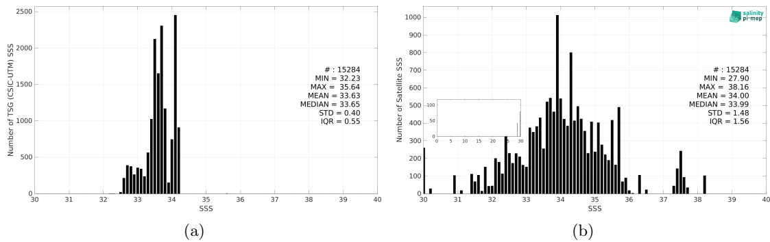
Figure 3: Histograms of SSS from TSG (CSIC-UTM) (a) and SMAP SSS L2 v5.3 (RSS) (b) considering all match-up pairs per bins of 0.1 over the Southern Ocean Pi-MEP region and for the full satellite product period.
