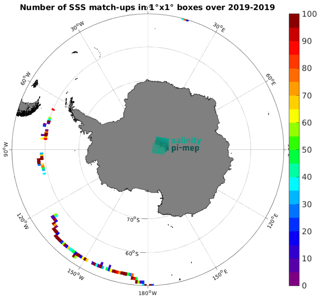
Figure 5: Number of SSS match-ups between Saildrone SSS and the SMAP SSS L2 v5.3 (RSS) SSS product for the Southern Ocean Pi-MEP region over 1^\circ \times 1^\circ boxes and for the full satellite product period.
