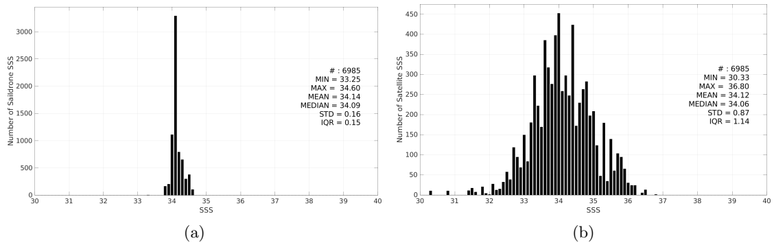
Figure 3: Histograms of SSS from Saildrone (a) and SMAP SSS L2 v5.3 (RSS) (b) considering all match-up pairs per bins of 0.1 over the Southern Ocean Pi-MEP region and for the full satellite product period.
