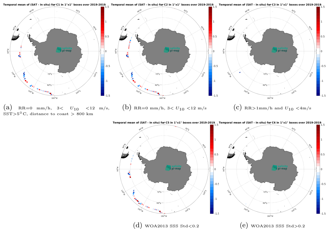
Figure 14: Temporal mean gridded over spatial boxes of size 1^\circ \times 1^\circ of \Delta\text{SSS} (SMAP SSS L2 v5.3 (RSS) - Saildrone) for 5 different subdatasets corresponding to:RR=0 mm/h, 3 < U_{10} < 12 m/s, SST > 5^\circ\text{C} , distance to coast > 800 km (a), RR=0 mm/h, 3 < U_{10} < 12 m/s (b), RR > 1 mm/h and U_{10} < 4 m/s (c), WOA2013 SSS Std < 0.2 (d), WOA2013 SSS Std > 0.2 (e).
