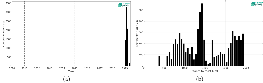
Figure 2: Number of match-ups between Saildrone and SMAP SSS L2 v5.3 (RSS) SSS as a function of time (a) and as function of the distance to coast (b) over the Southern Ocean Pi-MEP region and for the full satellite product period.
