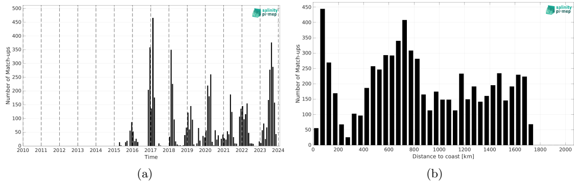
Figure 2: Number of match-ups between Marine mammals and SMAP SSS L2 v5.3 (RSS) SSS as a function of time (a) and as function of the distance to coast (b) over the Southern Ocean Pi-MEP region and for the full satellite product period.
