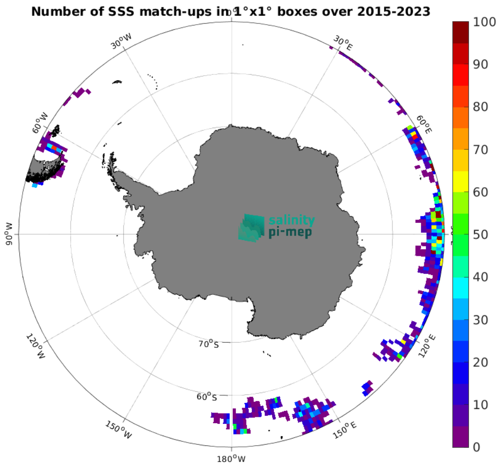
Figure 5: Number of SSS match-ups between Marine mammals SSS and the SMAP SSS L2 v5.3 (RSS) SSS product for the Southern Ocean Pi-MEP region over 1^\circ \times 1^\circ boxes and for the full satellite product period.
