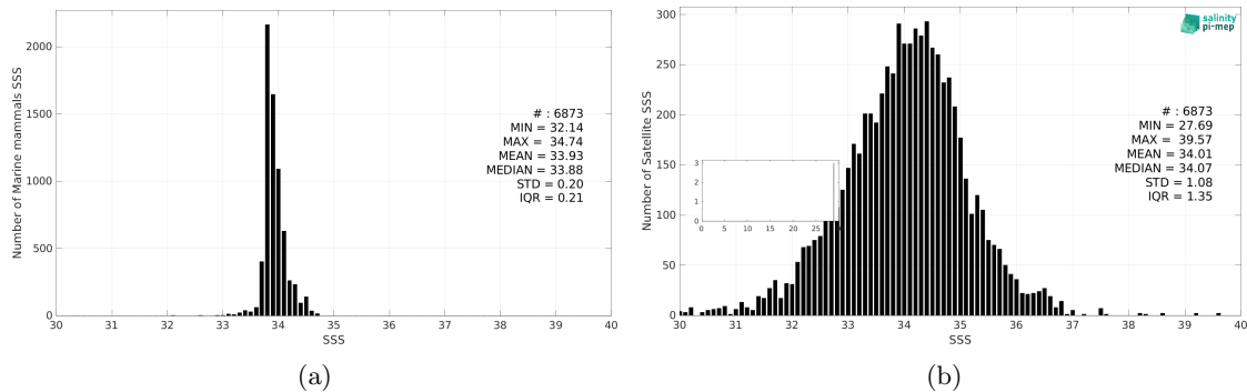
Figure 3: Histograms of SSS from Marine mammals (a) and SMAP SSS L2 v5.3 (RSS) (b) considering all match-up pairs per bins of 0.1 over the Southern Ocean Pi-MEP region and for the full satellite product period.
