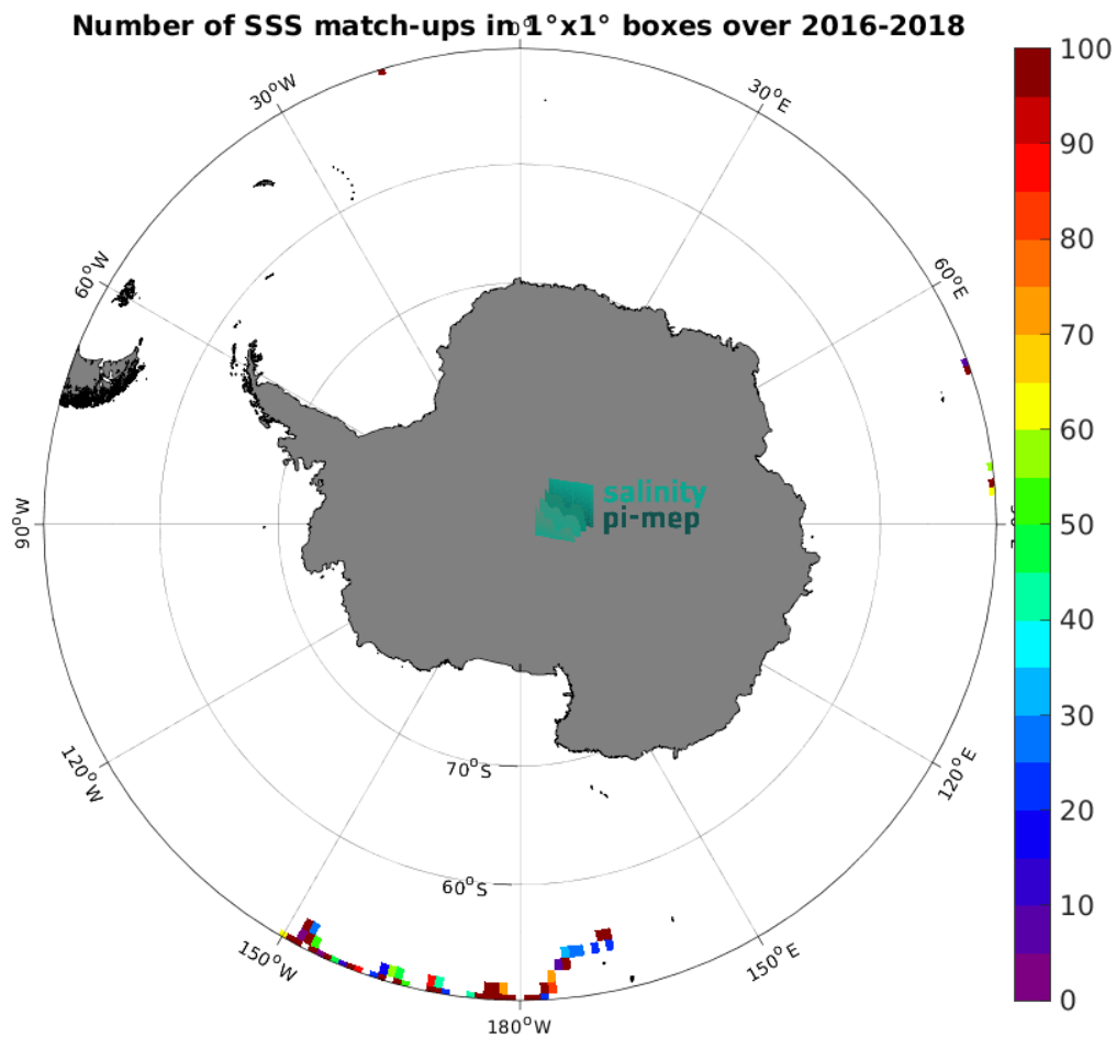
Figure 4: Number of SSS match-ups between Surface drifters SSS and the SMAP SSS L2 v5.3 (RSS) SSS product for the Southern Ocean Pi-MEP region over 1^{\circ} \times 1^{\circ} boxes and for the full satellite product period.
