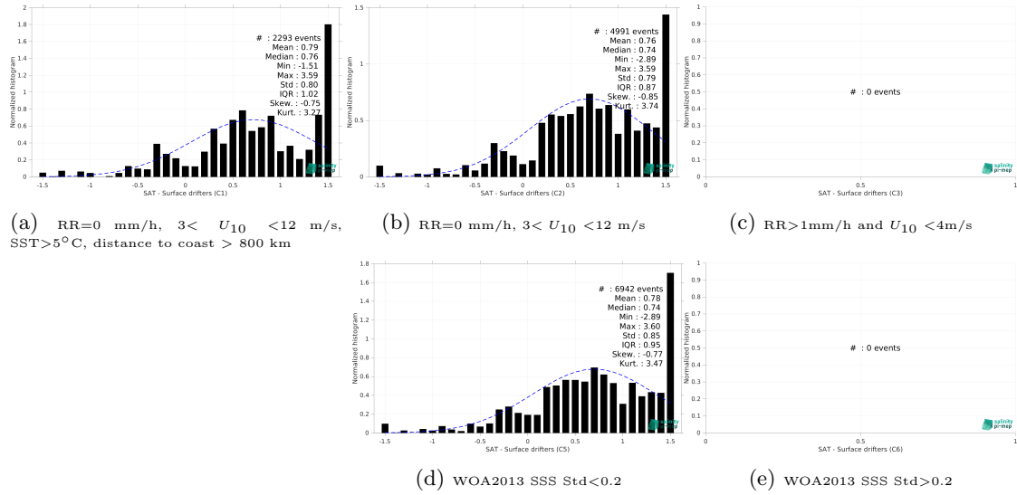
Figure 14: Normalized histogram of \Delta SSS (SMAP SSS L2 v5.3 (RSS) - Surface drifters) for 5 different subdatasets corresponding to: RR=0 mm/h, 3 < U_{10} < 12 m/s, SST>5°C, distance to coast > 800 km (a), RR=0 mm/h, 3 < U_{10} < 12 m/s (b), RR>1mm/h and U_{10} < 4 m/s (c), WOA2013 SSS Std<0.2 (d), WOA2013 SSS Std>0.2 (e).
