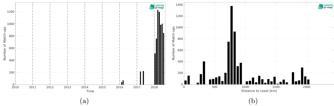
Figure 2: Number of match-ups between Surface drifters and SMAP SSS L2 v5.3 (RSS) SSS as a function of time (a) and as function of the distance to coast (b) over the Southern Ocean Pi-MEP region and for the full satellite product period.
