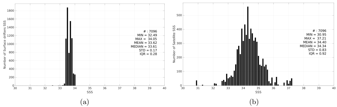
Figure 3: Histograms of SSS from Surface drifters (a) and SMAP SSS L2 v5.3 (RSS) (b) considering all match-up pairs per bins of 0.1 over the Southern Ocean Pi-MEP region and for the full satellite product period.
