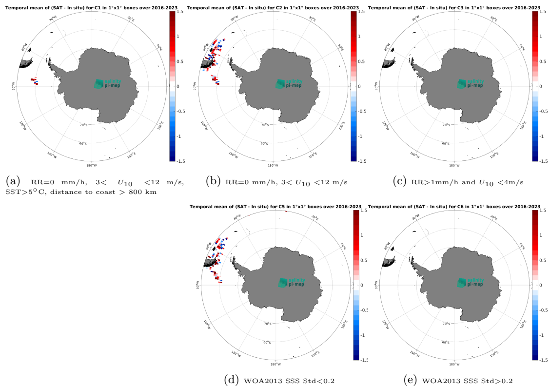
Figure 14: Temporal mean gridded over spatial boxes of size 1^\circ \times 1^\circ of \Delta SSS (SMAP SSS L2 v5.3 - 40 km (RSS) - TSG (Polarstern)) for 5 different subdatasets corresponding to:RR=0 mm/h, 3 < U_{10} < 12 m/s, SST >5^\circ C, distance to coast > 800 km (a), RR=0 mm/h, 3 < U_{10} < 12 m/s (b), RR >1 mm/h and U_{10} < 4 m/s (c), WOA2013 SSS Std <0.2 (d), WOA2013 SSS Std >0.2 (e).
