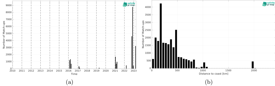
Figure 2: Number of match-ups between TSG (Polarstern) and SMAP SSS L2 v5.3 - 40 km (RSS) SSS as a function of time (a) and as function of the distance to coast (b) over the Southern Ocean Pi-MEP region and for the full satellite product period.
