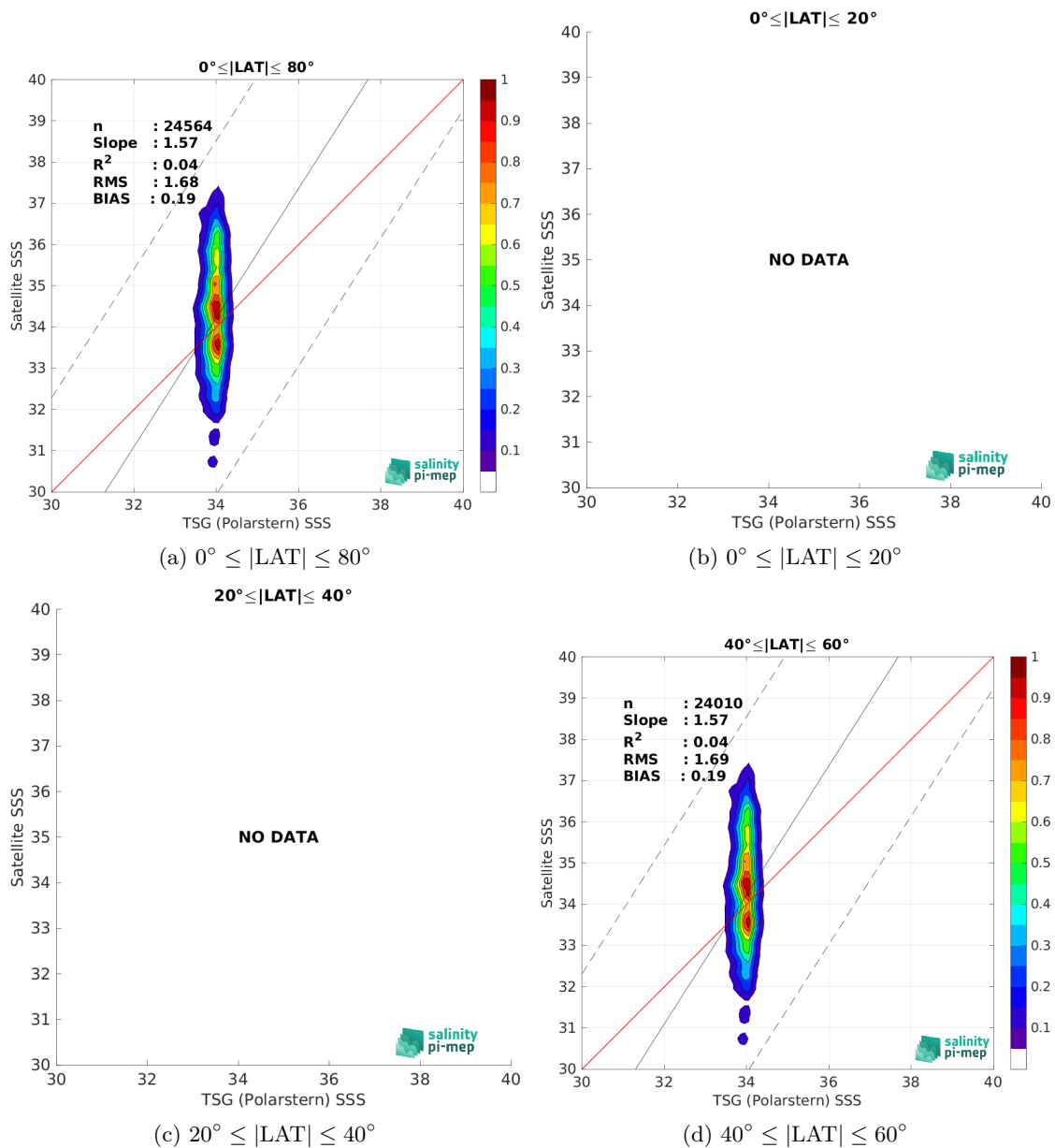
Figure 10: Contour maps of the concentration of SMAP SSS L2 v5.3 - 40 km (RSS) SSS (y-axis) versus TSG (Polarstern) SSS (x-axis) at match-up pairs for different latitude bands. For each plot, the red line shows x=y . The black thin and dashed lines indicate a linear fit through the data cloud and the \pm 95\% confidence levels, respectively. The number match-up pairs n , the slope and R^2 coefficient of the linear fit, the root mean square (RMS) and the mean bias between satellite and in situ data are indicated for each latitude band in each plot.
