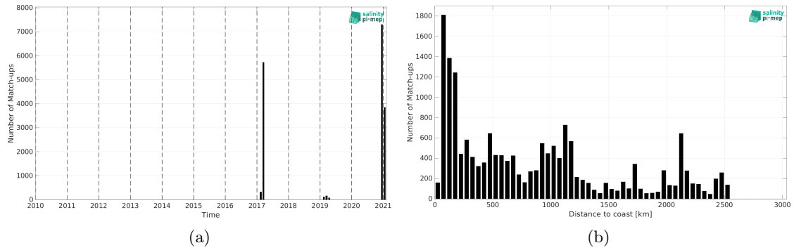
Figure 2: Number of match-ups between TSG (GOSUD-Sailing-ship) and SMAP SSS L2 v5.3 - 40 km (RSS) SSS as a function of time (a) and as function of the distance to coast (b) over the Southern Ocean Pi-MEP region and for the full satellite product period.
