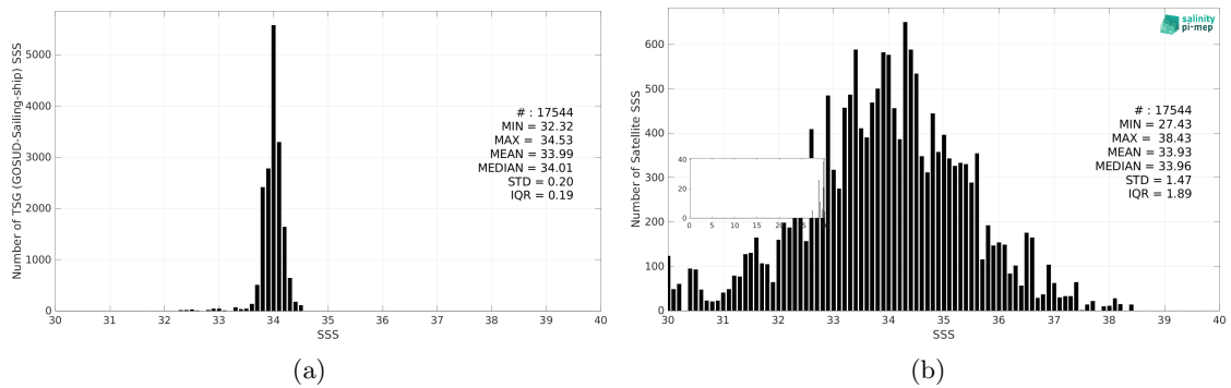
Figure 3: Histograms of SSS from TSG (GOSUD-Sailing-ship) (a) and SMAP SSS L2 v5.3 - 40 km (RSS) (b) considering all match-up pairs per bins of 0.1 over the Southern Ocean Pi-MEP region and for the full satellite product period.
