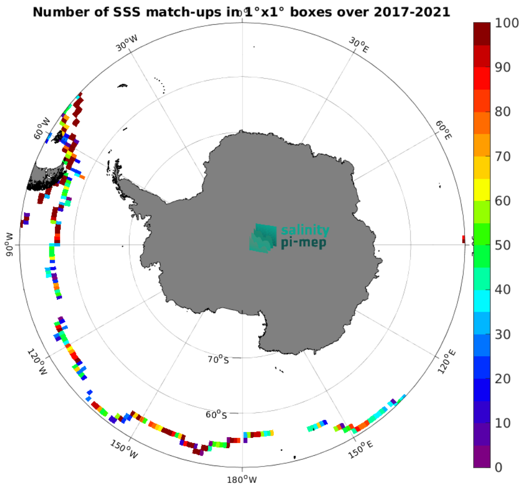
Figure 5: Number of SSS match-ups between TSG (GOSUD-Sailing-ship) SSS and the SMAP SSS L2 v5.3 - 40 km (RSS) SSS product for the Southern Ocean Pi-MEP region over 1^\circ \times 1^\circ boxes and for the full satellite product period.
