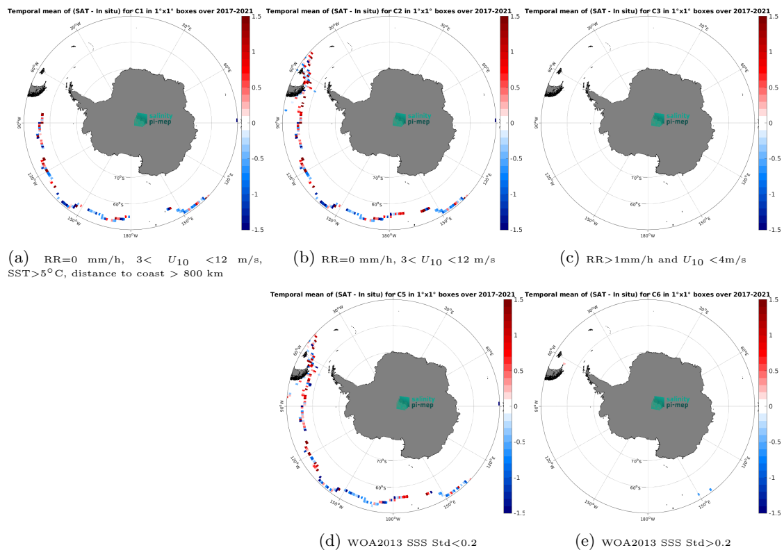
Figure 14: Temporal mean gridded over spatial boxes of size 1^\circ \times 1^\circ of \Delta\text{SSS} (SMAP SSS L2 v5.3 - 40 km (RSS) - TSG (GOSUD-Sailing-ship)) for 5 different subdatasets corresponding to:RR=0 mm/h, 3 < U_{10} < 12 m/s, SST>5°C, distance to coast > 800 km (a), RR=0 mm/h, 3 < U_{10} < 12 m/s (b), RR>1mm/h and U_{10} < 4 m/s (c), WOA2013 SSS Std<0.2 (d), WOA2013 SSS Std>0.2 (e).
