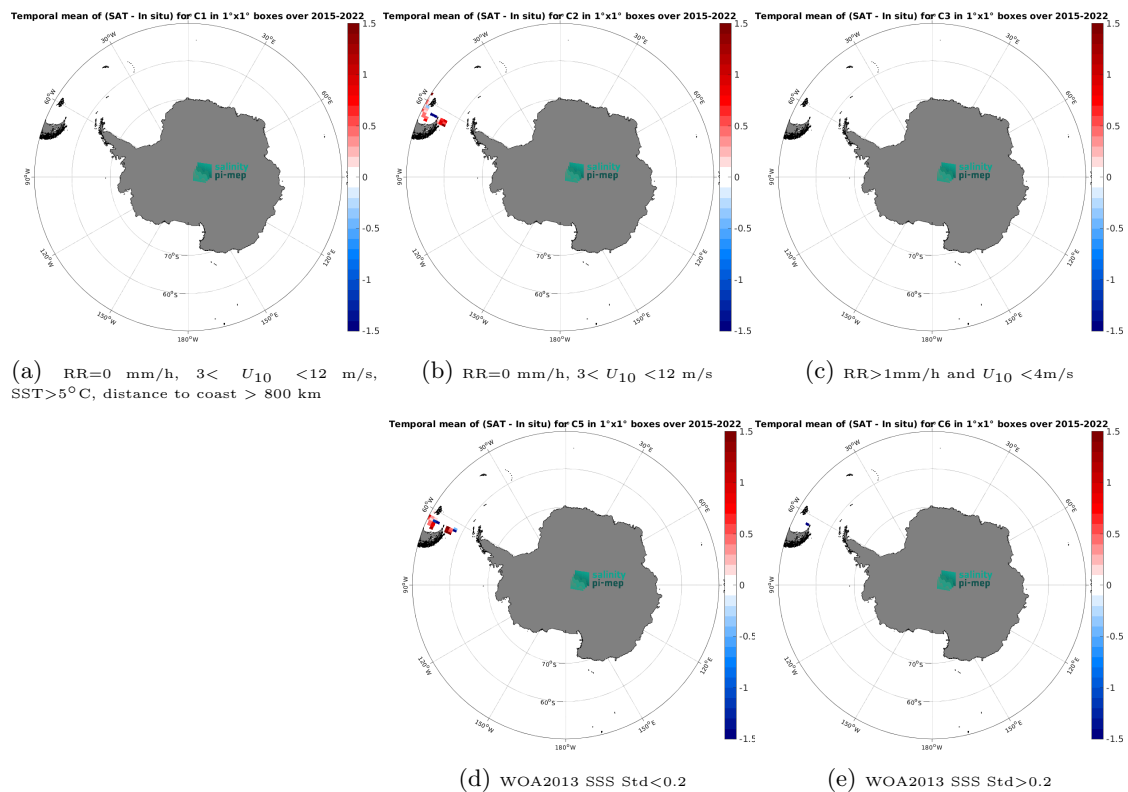
Figure 14: Temporal mean gridded over spatial boxes of size 1^\circ \times 1^\circ of \Delta\text{SSS} (SMAP SSS L2 v5.3 - 40 km (RSS) - TSG (CSIC-UTM)) for 5 different subdatasets corresponding to:RR=0 mm/h, 3 < U_{10} < 12 m/s, SST>5°C, distance to coast > 800 km (a), RR=0 mm/h, 3 < U_{10} < 12 m/s (b), RR>1mm/h and U_{10} < 4 m/s (c), WOA2013 SSS Std<0.2 (d), WOA2013 SSS Std>0.2 (e).
