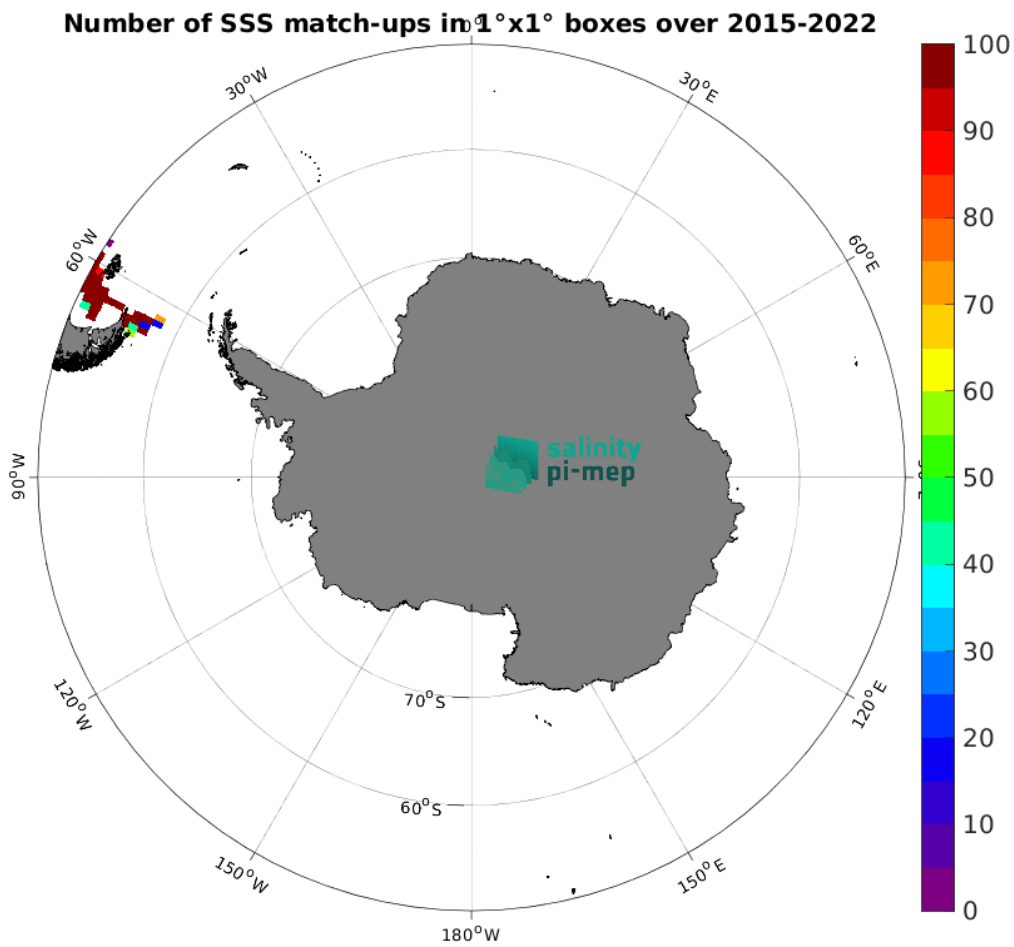
Figure 5: Number of SSS match-ups between TSG (CSIC-UTM) SSS and the SMAP SSS L2 v5.3 - 40 km (RSS) SSS product for the Southern Ocean Pi-MEP region over 1^{\circ} \times 1^{\circ} boxes and for the full satellite product period.
