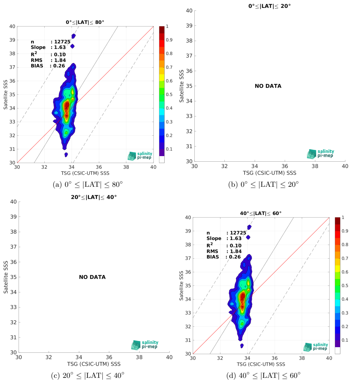
Figure 10: Contour maps of the concentration of SMAP SSS L2 v5.3 - 40 km (RSS) SSS (y-axis) versus TSG (CSIC-UTM) SSS (x-axis) at match-up pairs for different latitude bands. For each plot, the red line shows x=y . The black thin and dashed lines indicate a linear fit through the data cloud and the \pm 95\% confidence levels, respectively. The number match-up pairs n , the slope and R^2 coefficient of the linear fit, the root mean square (RMS) and the mean bias between satellite and in situ data are indicated for each latitude band in each plots.
