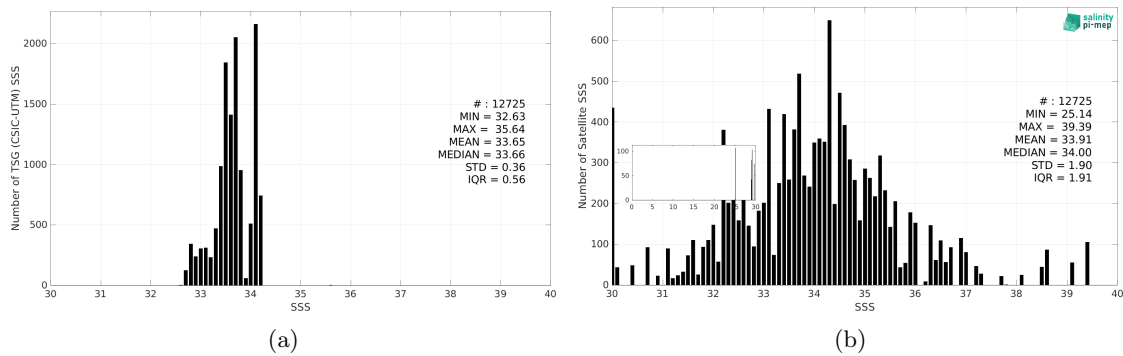
Figure 3: Histograms of SSS from TSG (CSIC-UTM) (a) and SMAP SSS L2 v5.3 - 40 km (RSS) (b) considering all match-up pairs per bins of 0.1 over the Southern Ocean Pi-MEP region and for the full satellite product period.
