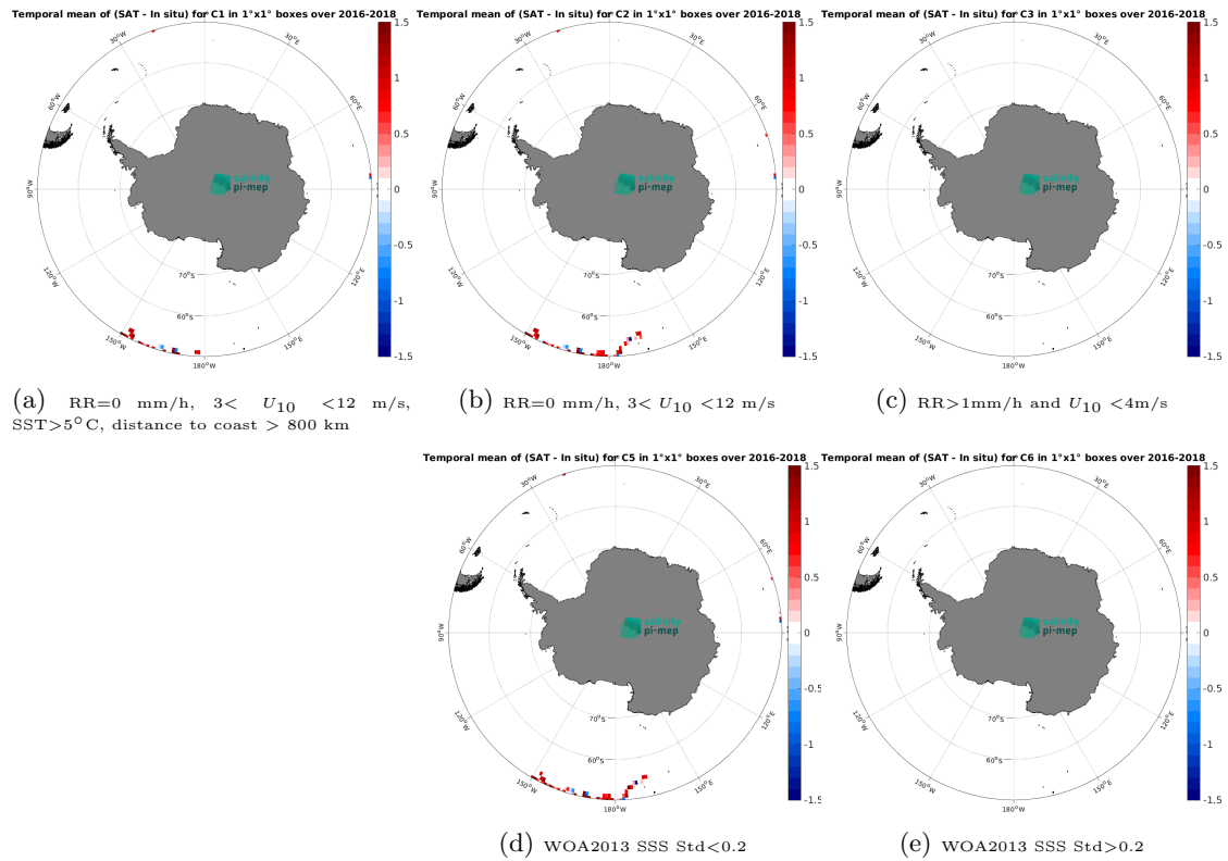
Figure 13: Temporal mean gridded over spatial boxes of size 1^\circ \times 1^\circ of \Delta SSS (SMAP SSS L2 v5.3 - 40 km (RSS) - Surface drifters) for 5 different subdatasets corresponding to:RR=0 mm/h, 3 < U_{10} < 12 m/s, SST > 5^\circ\text{C} , distance to coast > 800 km (a), RR=0 mm/h, 3 < U_{10} < 12 m/s (b), RR > 1 mm/h and U_{10} < 4 m/s (c), WOA2013 SSS Std < 0.2 (d), WOA2013 SSS Std > 0.2 (e).
