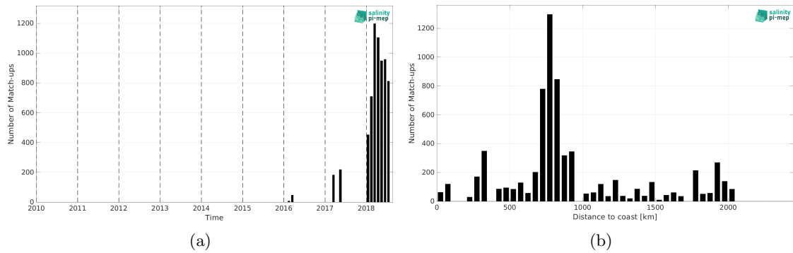
Figure 2: Number of match-ups between Surface drifters and SMAP SSS L2 v5.3 - 40 km (RSS) SSS as a function of time (a) and as function of the distance to coast (b) over the Southern Ocean Pi-MEP region and for the full satellite product period.
