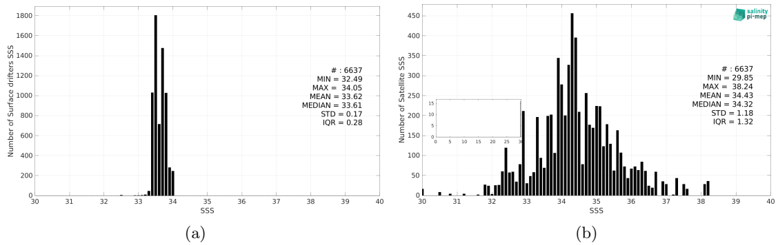
Figure 3: Histograms of SSS from Surface drifters (a) and SMAP SSS L2 v5.3 - 40 km (RSS) (b) considering all match-up pairs per bins of 0.1 over the Southern Ocean Pi-MEP region and for the full satellite product period.
