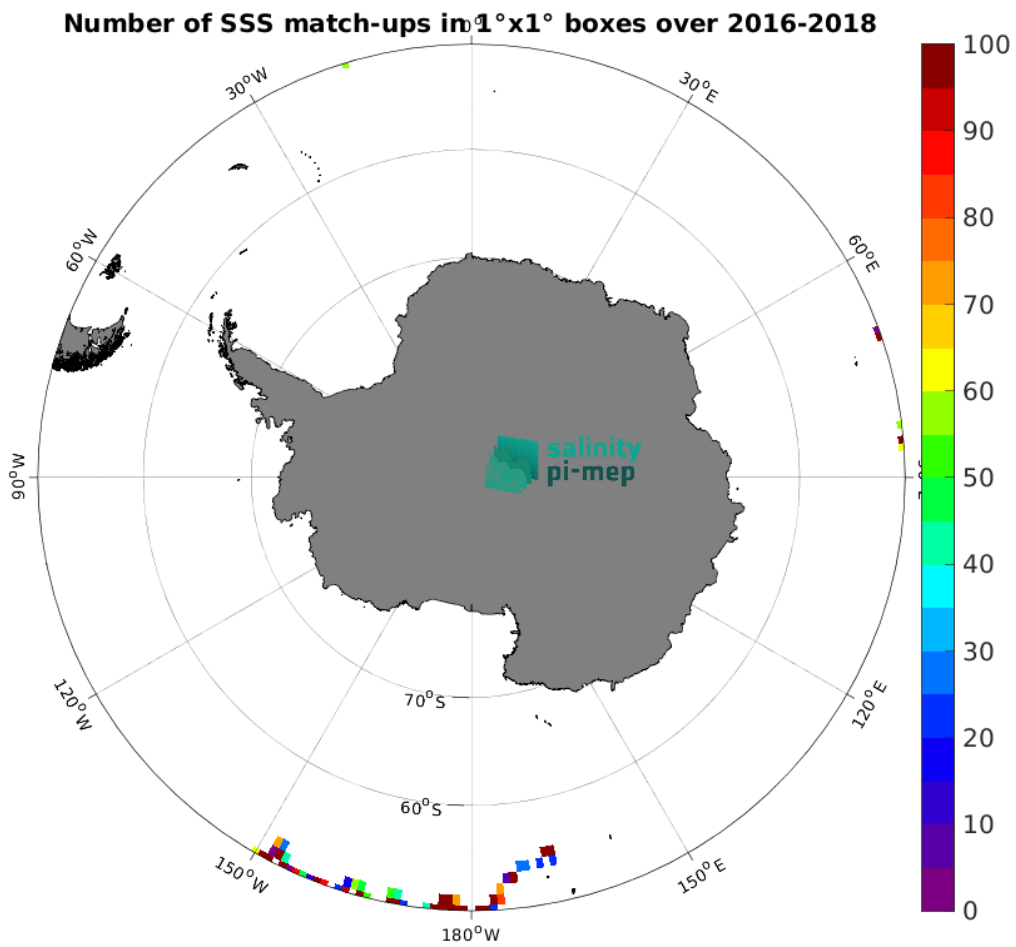
Figure 4: Number of SSS match-ups between Surface drifters SSS and the SMAP SSS L2 v5.3 - 40 km (RSS) SSS product for the Southern Ocean Pi-MEP region over 1^\circ \times 1^\circ boxes and for the full satellite product period.
