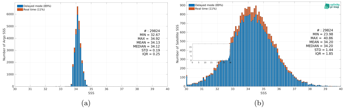
Figure 3: Histograms of SSS from Argo (a) and SMAP SSS L2 v5.3 - 40 km (RSS) (b) considering all match-up pairs per bins of 0.1 over the Southern Ocean Pi-MEP region and for the full satellite product period.
