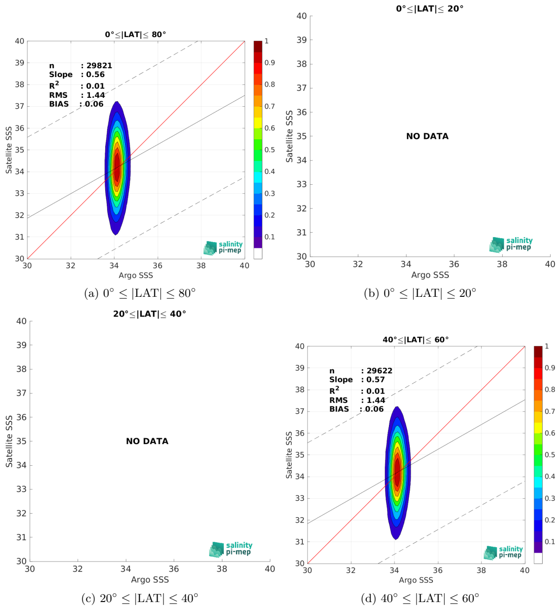
Figure 10: Contour maps of the concentration of SMAP SSS L2 v5.3 - 40 km (RSS) SSS (y-axis) versus Argo SSS (x-axis) at match-up pairs for different latitude bands. For each plot, the red line shows x=y . The black thin and dashed lines indicate a linear fit through the data cloud and the \pm 95\% confidence levels, respectively. The number match-up pairs n , the slope and R^2 coefficient of the linear fit, the root mean square (RMS) and the mean bias between satellite and in situ data are indicated for each latitude band in each plots.
