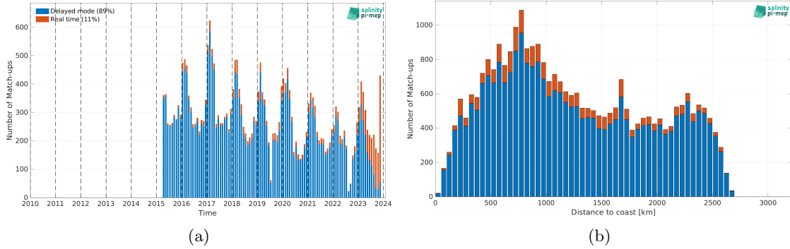
Figure 2: Number of match-ups between Argo and SMAP SSS L2 v5.3 - 40 km (RSS) SSS as a function of time (a) and as function of the distance to coast (b) over the Southern Ocean Pi-MEP region and for the full satellite product period.
