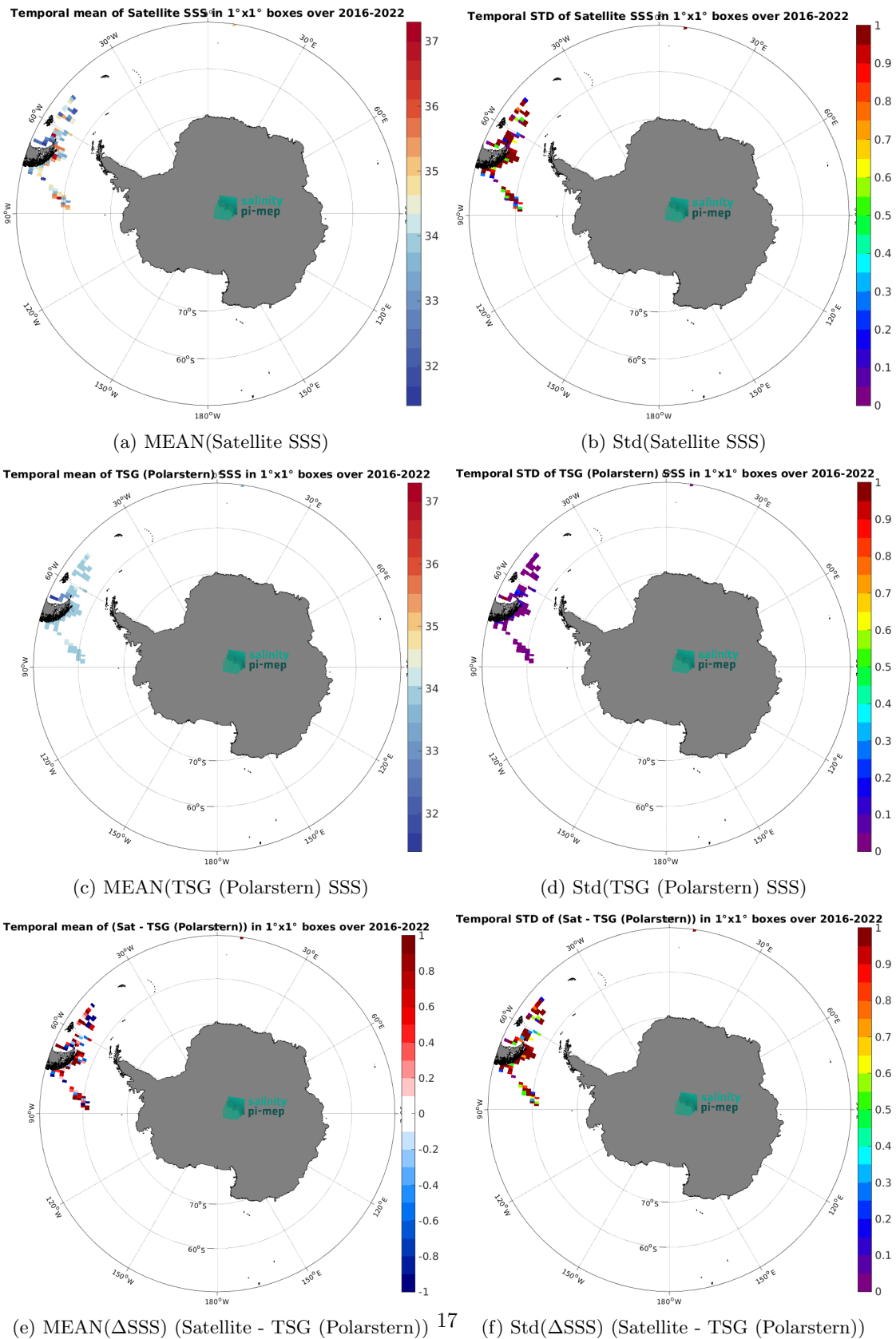
Figure 6: Temporal mean (left) and Std (right) of SSS from SMAP SSS L2 v5 - 40 km (RSS) (top), TSG (Polarstern) (middle), and of \Delta SSS (Satellite - TSG (Polarstern)). Only match-up pairs are used to generate these maps.
