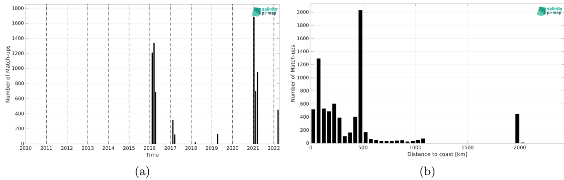
Figure 1: Number of match-ups between TSG (Polarstern) and SMAP SSS L2 v5 - 40 km (RSS) SSS as a function of time (a) and as function of the distance to coast (b) over the Southern Ocean Pi-MEP region and for the full satellite product period.
