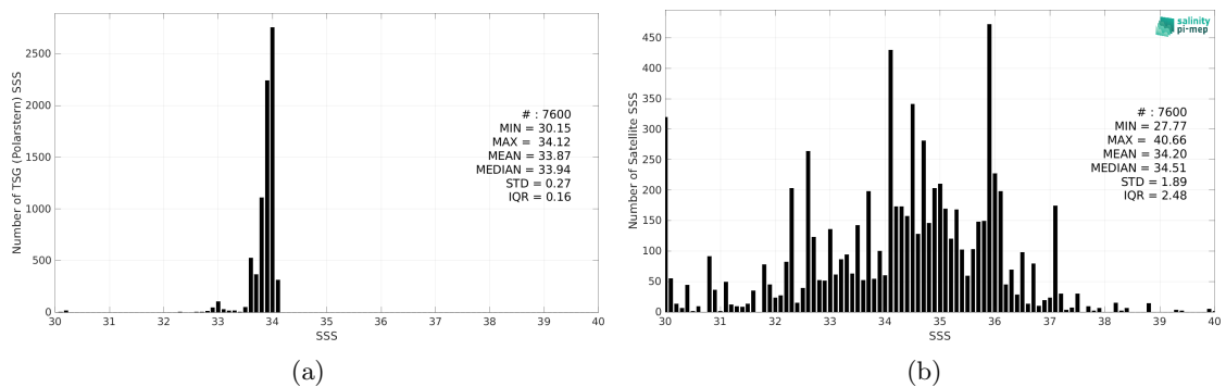
Figure 2: Histograms of SSS from TSG (Polarstern) (a) and SMAP SSS L2 v5 - 40 km (RSS) (b) considering all match-up pairs per bins of 0.1 over the Southern Ocean Pi-MEP region and for the full satellite product period.
