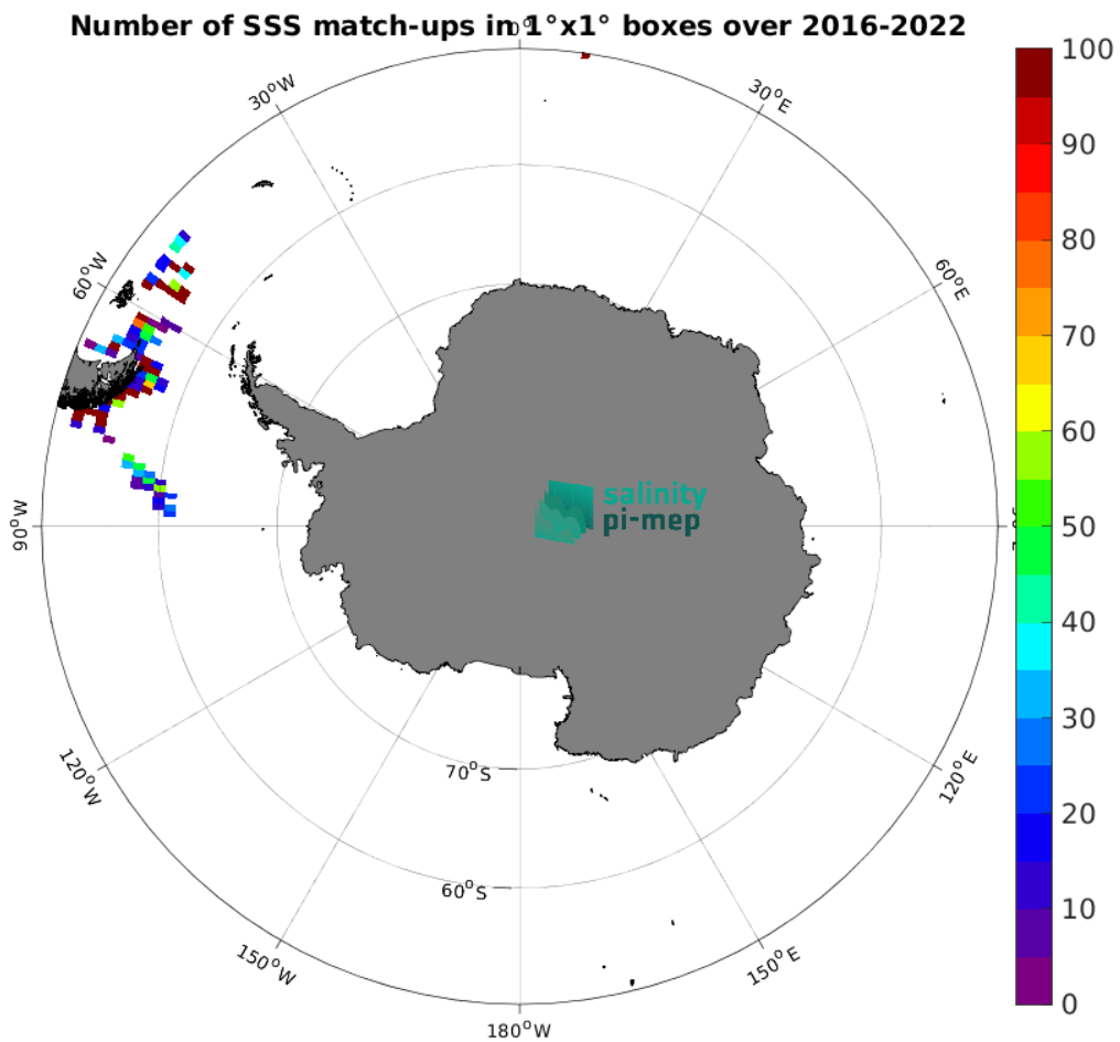
Figure 4: Number of SSS match-ups between TSG (Polarstern) SSS and the SMAP SSS L2 v5 - 40 km (RSS) SSS product for the Southern Ocean Pi-MEP region over 1^\circ \times 1^\circ boxes and for the full satellite product period.
