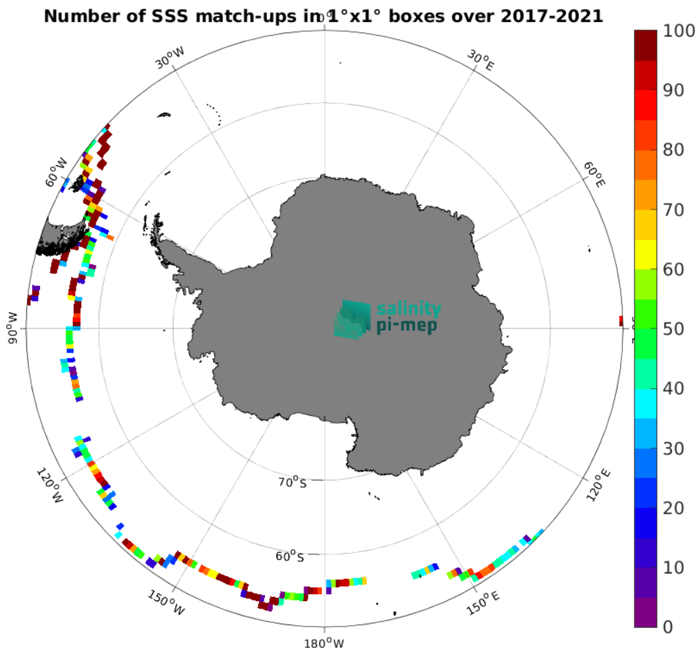
Figure 4: Number of SSS match-ups between TSG (GOSUD-Sailing-ship) SSS and the SMAP SSS L2 v5 - 40 km (RSS) SSS product for the Southern Ocean Pi-MEP region over 1^{\circ} \times 1^{\circ} boxes and for the full satellite product period.
