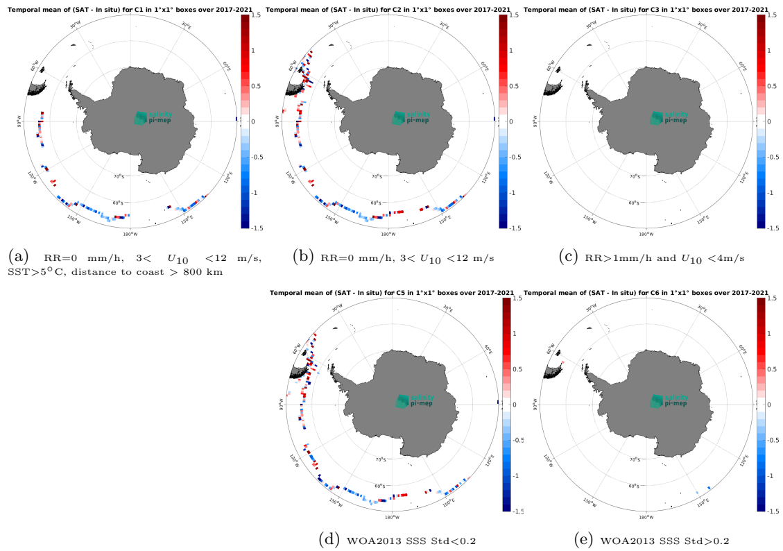
Figure 12: Temporal mean gridded over spatial boxes of size 1^\circ \times 1^\circ of \Delta\text{SSS} (SMAP SSS L2 v5 - 40 km (RSS) - TSG (GOSUD-Sailing-ship)) for 5 different subdatasets corresponding to: RR=0 mm/h, 3 < U_{10} < 12 m/s, SST > 5^\circ\text{C} , distance to coast > 800 km (a), RR=0 mm/h, 3 < U_{10} < 12 m/s (b), RR > 1 mm/h and U_{10} < 4 m/s (c), WOA2013 SSS Std < 0.2 (d), WOA2013 SSS Std > 0.2 (e).
