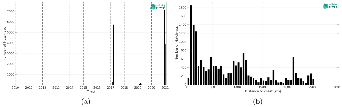
Figure 1: Number of match-ups between TSG (GOSUD-Sailing-ship) and SMAP SSS L2 v5 - 40 km (RSS) SSS as a function of time (a) and as function of the distance to coast (b) over the Southern Ocean Pi-MEP region and for the full satellite product period.
