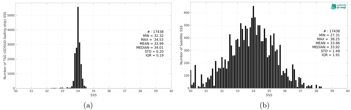
Figure 2: Histograms of SSS from TSG (GOSUD-Sailing-ship) (a) and SMAP SSS L2 v5 - 40 km (RSS) (b) considering all match-up pairs per bins of 0.1 over the Southern Ocean Pi-MEP region and for the full satellite product period.
