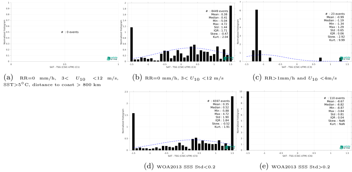
Figure 13: Normalized histogram of \Delta\text{SSS} (SMAP SSS L2 v5 - 40 km (RSS) - TSG (CSIC-UTM)) for 5 different subdatasets corresponding to: RR=0 mm/h, 3 < U_{10} < 12 m/s, SST > 5^{\circ}\text{C} , distance to coast > 800 km (a), RR=0 mm/h, 3 < U_{10} < 12 m/s (b), RR > 1\text{mm/h} and U_{10} < 4\text{m/s} (c), WOA2013 SSS Std < 0.2 (d), WOA2013 SSS Std > 0.2 (e).
