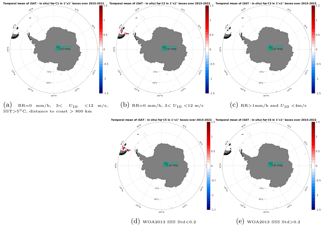
Figure 12: Temporal mean gridded over spatial boxes of size 1^{\circ}\times 1^{\circ} of \Delta\text{SSS} (SMAP SSS L2 v5 - 40 km (RSS) - TSG (CSIC-UTM)) for 5 different subdatasets corresponding to: \text{RR}=0 mm/h, 3 < U_{10} < 12 m/s, \text{SST}>5^{\circ}\text{C} , distance to coast > 800 km (a), \text{RR}=0 mm/h, 3 < U_{10} < 12 m/s (b), \text{RR}>1 mm/h and U_{10} < 4 m/s (c), WOA2013 SSS Std < 0.2 (d), WOA2013 SSS Std > 0.2 (e).
