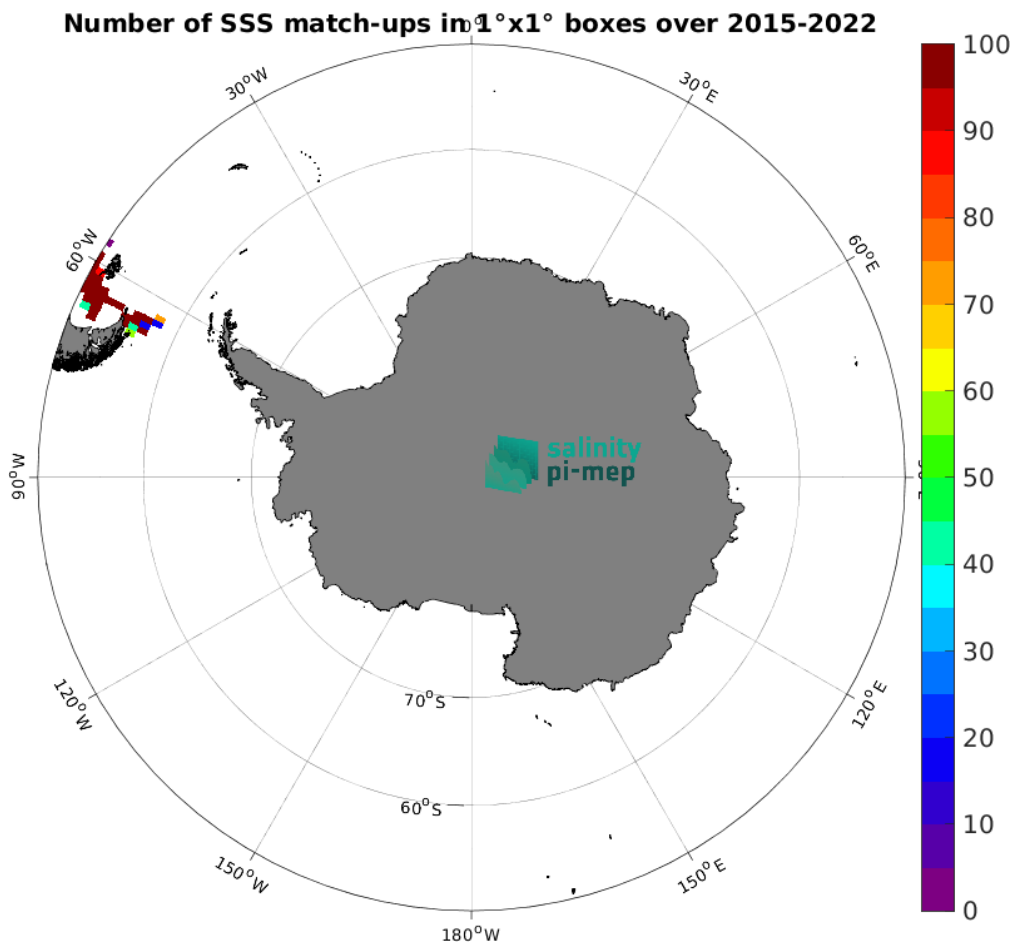
Figure 4: Number of SSS match-ups between TSG (CSIC-UTM) SSS and the SMAP SSS L2 v5 - 40 km (RSS) SSS product for the Southern Ocean Pi-MEP region over 1^\circ \times 1^\circ boxes and for the full satellite product period.
