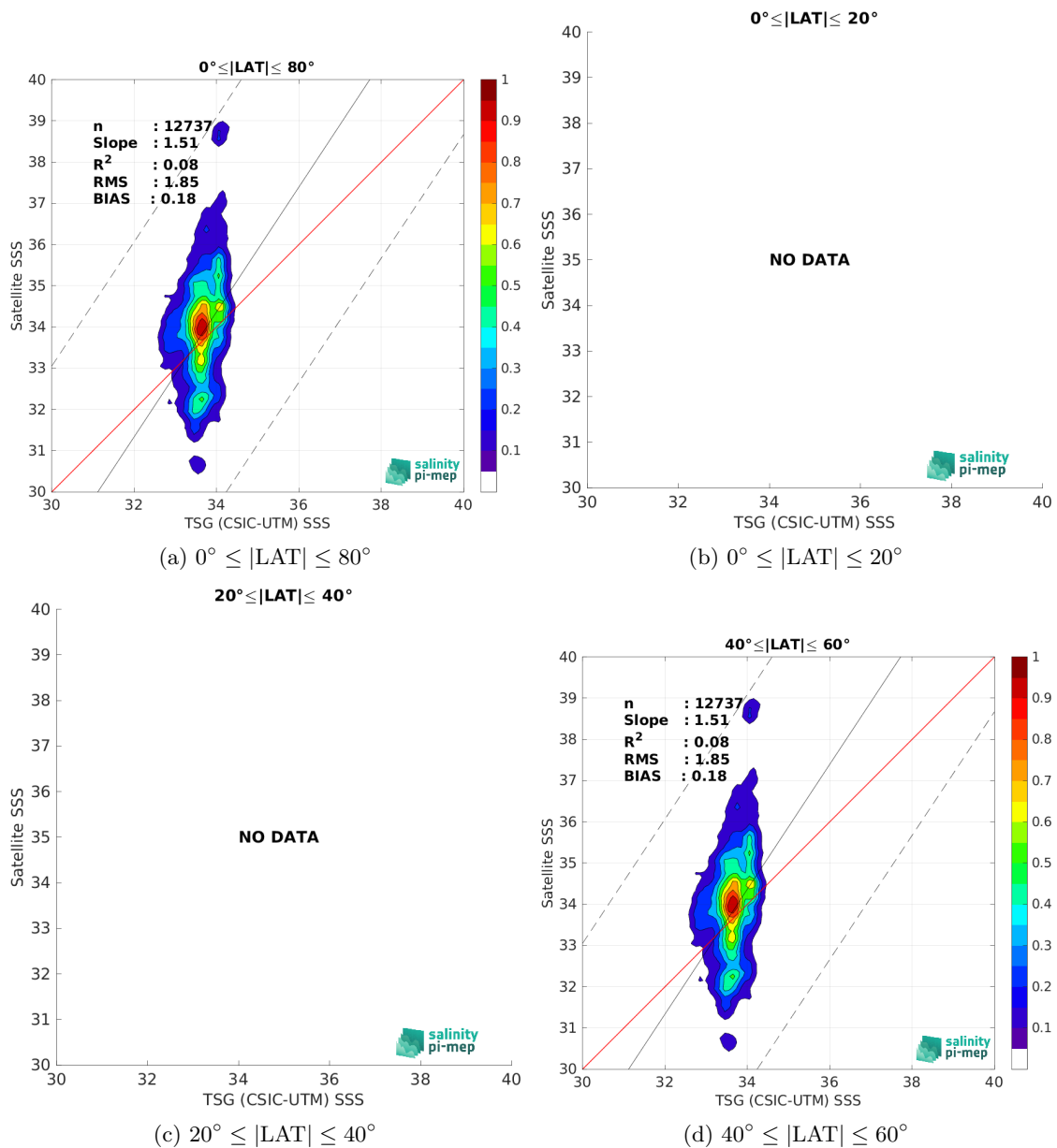
Figure 9: Contour maps of the concentration of SMAP SSS L2 v5 - 40 km (RSS) SSS (y-axis) versus TSG (CSIC-UTM) SSS (x-axis) at match-up pairs for different latitude bands. For each plot, the red line shows x=y . The black thin and dashed lines indicate a linear fit through the data cloud and the \pm 95\% confidence levels, respectively. The number match-up pairs n , the slope and R^2 coefficient of the linear fit, the root mean square (RMS) and the mean bias between satellite and in situ data are indicated for each latitude band in each plots.
