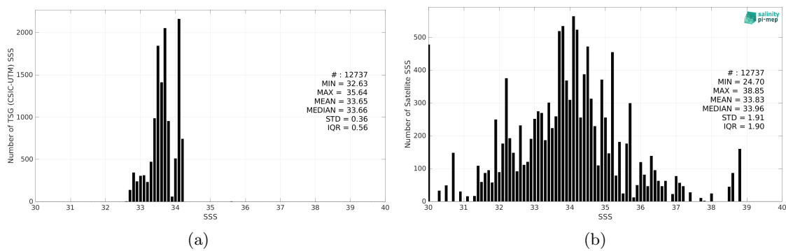
Figure 2: Histograms of SSS from TSG (CSIC-UTM) (a) and SMAP SSS L2 v5 - 40 km (RSS) (b) considering all match-up pairs per bins of 0.1 over the Southern Ocean Pi-MEP region and for the full satellite product period.
