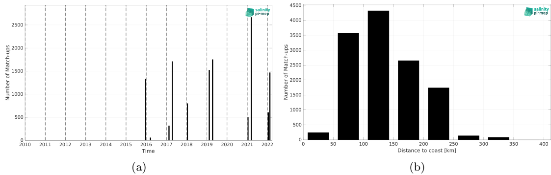
Figure 1: Number of match-ups between TSG (CSIC-UTM) and SMAP SSS L2 v5 - 40 km (RSS) SSS as a function of time (a) and as function of the distance to coast (b) over the Southern Ocean Pi-MEP region and for the full satellite product period.
