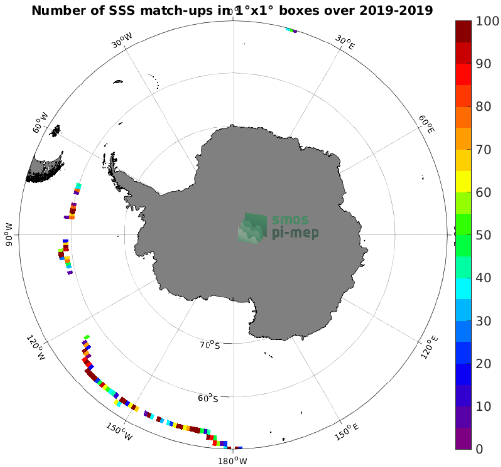
Figure 4: Number of SSS match-ups between Saildrone SSS and the SMAP SSS L2 v5 - 40 km (RSS) SSS product for the Southern Ocean Pi-MEP region over 1^\circ \times 1^\circ boxes and for the full satellite product period.
