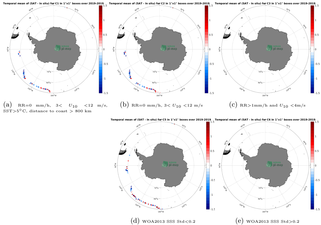
Figure 12: Temporal mean gridded over spatial boxes of size 1^{\circ}\times 1^{\circ} of \Delta\text{SSS} (SMAP SSS L2 v5 - 40 km (RSS) - Sairdrone) for 5 different subdatasets corresponding to: \text{RR}=0 mm/h, 3 < U_{10} < 12 m/s, \text{SST}>5^{\circ}\text{C} , distance to coast > 800 km (a), \text{RR}=0 mm/h, 3 < U_{10} < 12 m/s (b), \text{RR}>1 mm/h and U_{10} < 4 m/s (c), WOA2013 SSS Std <0.2 (d), WOA2013 SSS Std >0.2 (e).
