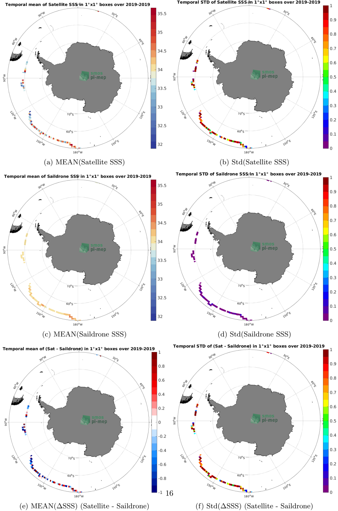
Figure 6: Temporal mean (left) and Std (right) of SSS from SMAP SSS L2 v5 - 40 km (RSS) (top), Saildrone (middle), and of \Delta SSS (Satellite - Saildrone). Only match-up pairs are used to generate these maps.
