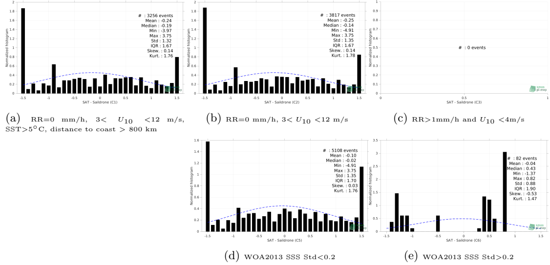
Figure 13: Normalized histogram of \Delta SSS (SMAP SSS L2 v5 - 40 km (RSS) - Saildrone) for 5 different subdatasets corresponding to: RR=0 mm/h, 3 < U_{10} < 12 m/s, SST > 5°C, distance to coast > 800 km (a), RR=0 mm/h, 3 < U_{10} < 12 m/s (b), RR > 1mm/h and U_{10} < 4 m/s (c), WOA2013 SSS Std < 0.2 (d), WOA2013 SSS Std > 0.2 (e).
