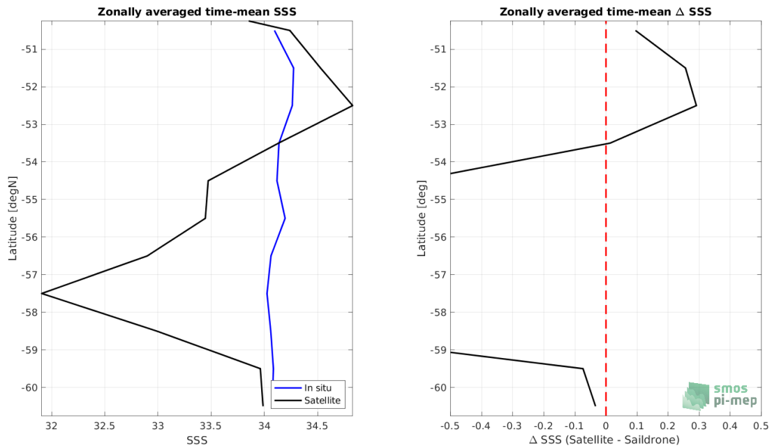
Figure 8: Left panel: Zonal mean SSS from SMAP SSS L2 v5 - 40 km (RSS) satellite product (black) and from Sairdrone (blue). Right panel: Zonal mean of \Delta SSS (Satellite - Sairdrone) for all the collected Pi-MEP match-up pairs estimated over the full satellite product period.
