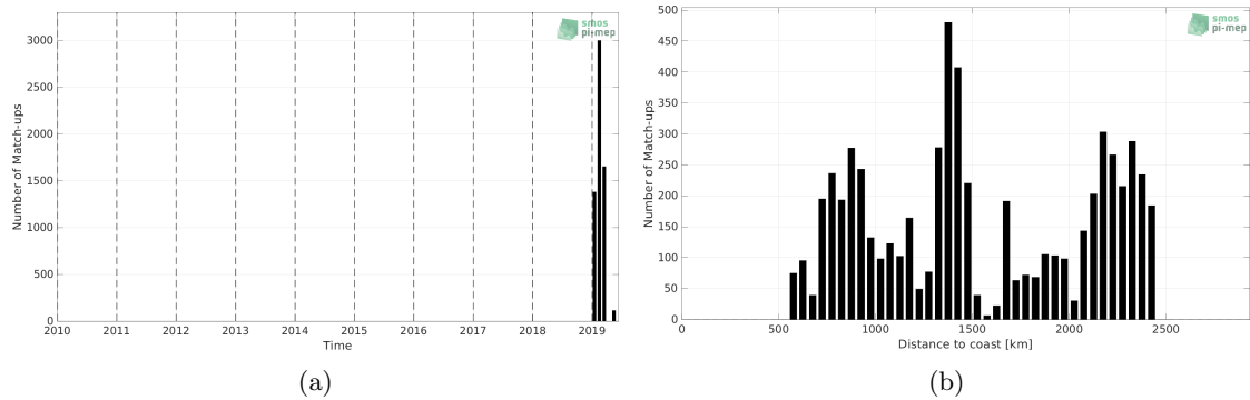
Figure 1: Number of match-ups between Saildrone and SMAP SSS L2 v5 - 40 km (RSS) SSS as a function of time (a) and as function of the distance to coast (b) over the Southern Ocean Pi-MEP region and for the full satellite product period.
