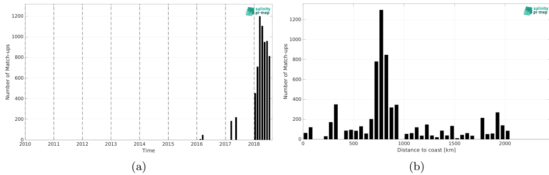
Figure 1: Number of match-ups between Surface drifters and SMAP SSS L2 v5 - 40 km (RSS) SSS as a function of match-up time (a) and as function of the distance to coast (b) over the Southern Ocean Pi-MEP region and for the full satellite product period.
