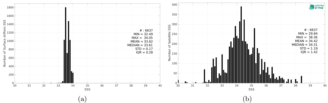
Figure 2: Histograms of SSS from Surface drifters (a) and SMAP SSS L2 v5 - 40 km (RSS) (b) considering all match-up pairs per bins of 0.1 over the Southern Ocean Pi-MEP region and for the full satellite product period.
