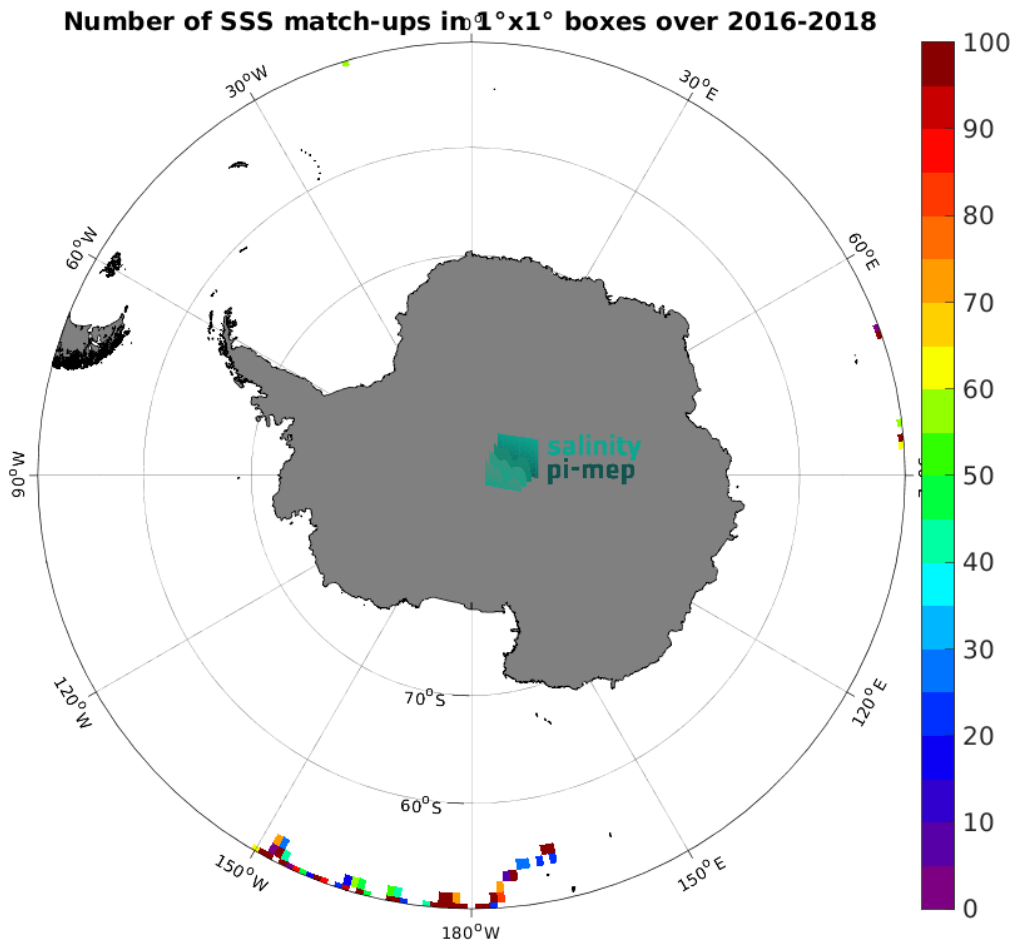
Figure 3: Number of SSS match-ups between Surface drifters SSS and the SMAP SSS L2 v5 - 40 km (RSS) SSS product for the Southern Ocean Pi-MEP region over 1^\circ \times 1^\circ boxes and for the full satellite product period.
