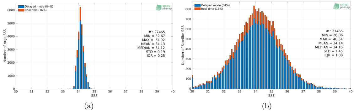
Figure 2: Histograms of SSS from Argo (a) and SMAP SSS L2 v5 - 40 km (RSS) (b) considering all match-up pairs per bins of 0.1 over the Southern Ocean Pi-MEP region and for the full satellite product period.
