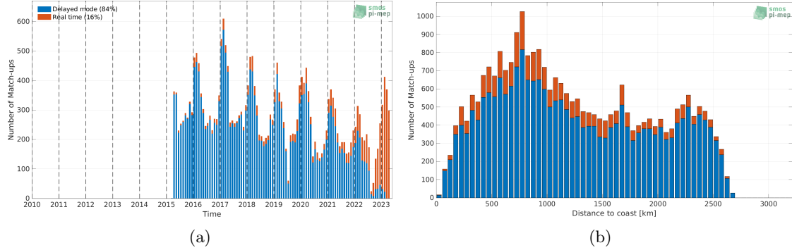
Figure 1: Number of match-ups between Argo and SMAP SSS L2 v5 - 40 km (RSS) SSS as a function of time (a) and as function of the distance to coast (b) over the Southern Ocean Pi-MEP region and for the full satellite product period.
