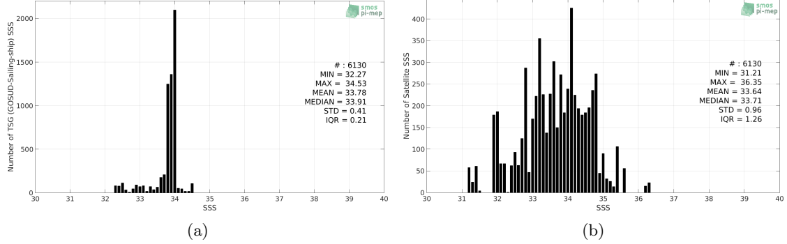
Figure 2: Histograms of SSS from TSG (GOSUD-Sailing-ship) (a) and SMAP SSS L2 v4 (RSS) (b) considering all match-up pairs per bins of 0.1 over the Southern Ocean Pi-MEP region and for the full satellite product period.
