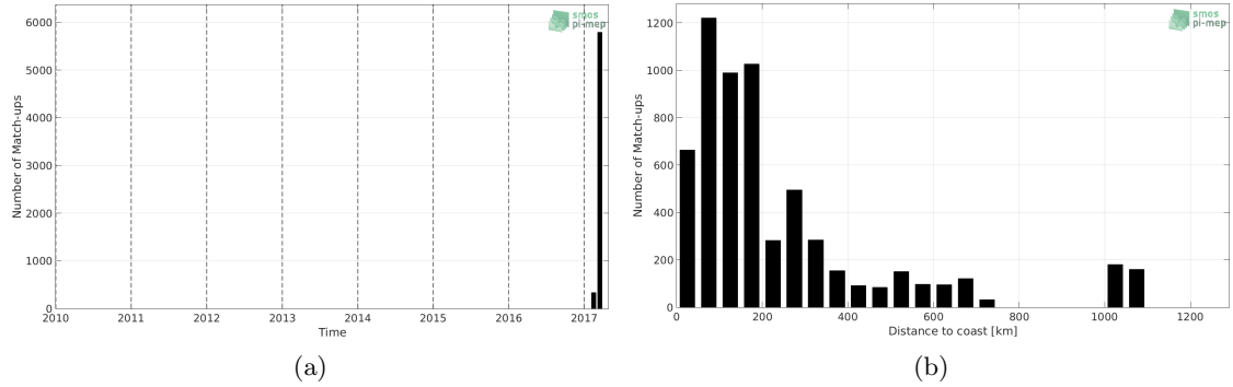
Figure 1: Number of match-ups between TSG (GOSUD-Sailing-ship) and SMAP SSS L2 v4 (RSS) SSS as a function of time (a) and as function of the distance to coast (b) over the Southern Ocean Pi-MEP region and for the full satellite product period.
