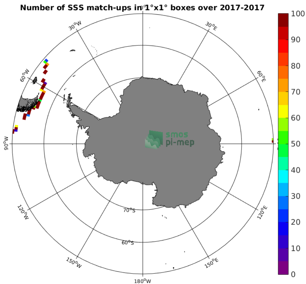
Figure 4: Number of SSS match-ups between TSG (GOSUD-Sailing-ship) SSS and the SMAP SSS L2 v4 (RSS) SSS product for the Southern Ocean Pi-MEP region over 1^\circ \times 1^\circ boxes and for the full satellite product period.
