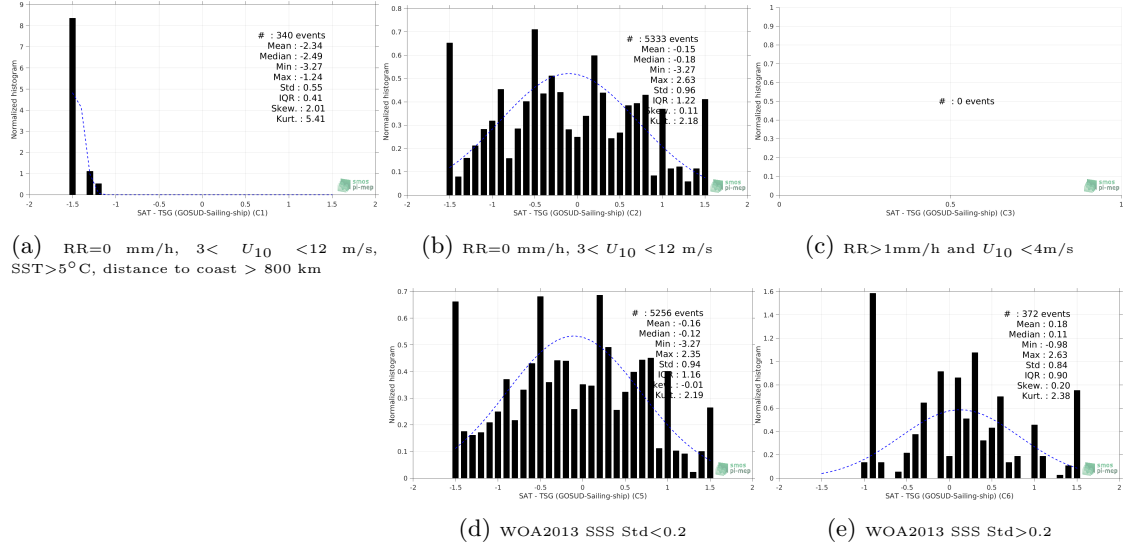
Figure 13: Normalized histogram of \Delta\text{SSS} (SMAP SSS L2 v4 (RSS) - TSG (GOSUD-Sailing-ship)) for 5 different subdatasets corresponding to: \text{RR}=0 \text{ mm/h} , 3 < U_{10} < 12 \text{ m/s} , \text{SST} > 5^\circ\text{C} , distance to coast > 800 \text{ km} (a), \text{RR}=0 \text{ mm/h} , 3 < U_{10} < 12 \text{ m/s} (b), \text{RR} > 1 \text{ mm/h} and U_{10} < 4 \text{ m/s} (c), WOA2013 SSS Std < 0.2 (d), WOA2013 SSS Std > 0.2 (e).
