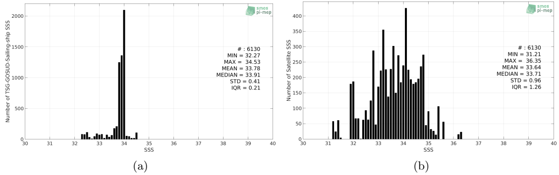
Figure 2: Histograms of SSS from TSG-GOSUD-Sailing-ship (a) and SMAP-L2-RSS-V4 (b) considering all match-up pairs per bins of 0.1 over the Southern Ocean Pi-MEP region and for the full satellite product period.
