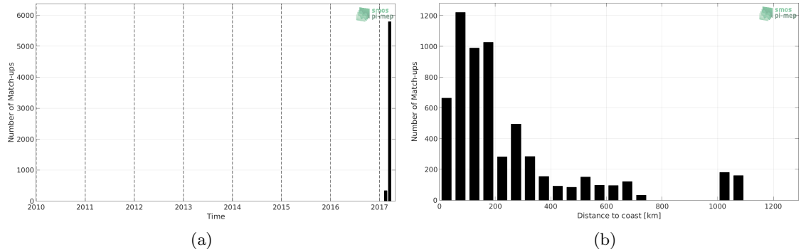
Figure 1: Number of match-ups between TSG-GOSUD-Sailing-ship and SMAP-L2-RSS-V4 SSS as a function of time (a) and as function of the distance to coast (b) over the Southern Ocean Pi-MEP region and for the full satellite product period.
