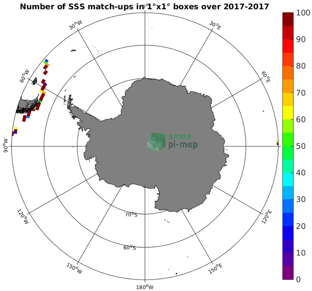
Figure 4: Number of SSS match-ups between TSG-GOSUD-Sailing-ship SSS and the SMAP-L2-RSS-V4 SSS product for the Southern Ocean Pi-MEP region over 1^\circ \times 1^\circ boxes and for the full satellite product period.
