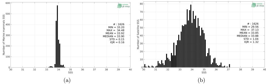
Figure 2: Histograms of SSS from Marine mammals (a) and SMAP SSS L2 v4 (RSS) (b) considering all match-up pairs per bins of 0.1 over the Southern Ocean Pi-MEP region and for the full satellite product period.
