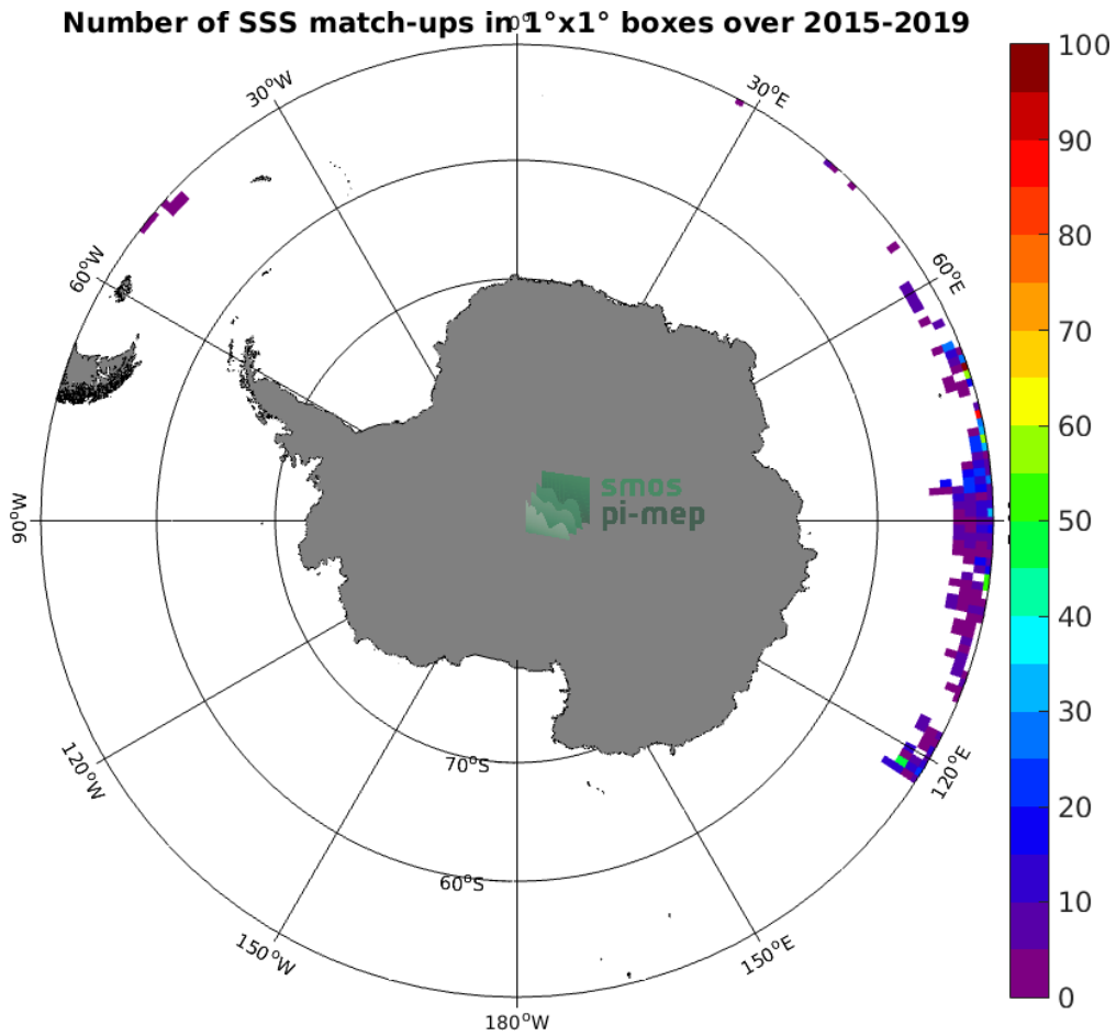
Figure 4: Number of SSS match-ups between Marine mammals SSS and the SMAP SSS L2 v4 (RSS) SSS product for the Southern Ocean Pi-MEP region over 1^\circ \times 1^\circ boxes and for the full satellite product period.
