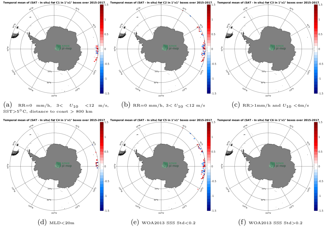
Figure 12: Temporal mean gridded over spatial boxes of size 1^{\circ}\times 1^{\circ} of \Delta\text{SSS} (SMAP SSS L2 v4 (RSS) - Sea mammals) for 6 different subdatasets corresponding to: \text{RR}=0 mm/h, 3 < U_{10} < 12 m/s, \text{SST}>5^{\circ}\text{C} , distance to coast > 800 km (a), \text{RR}=0 mm/h, 3 < U_{10} < 12 m/s (b), \text{RR}>1\text{mm/h} and U_{10} < 4\text{m/s} (c), \text{MLD}<20\text{m} (d), \text{WOA2013 SSS Std}<0.2 (e), \text{WOA2013 SSS Std}>0.2 (f).
