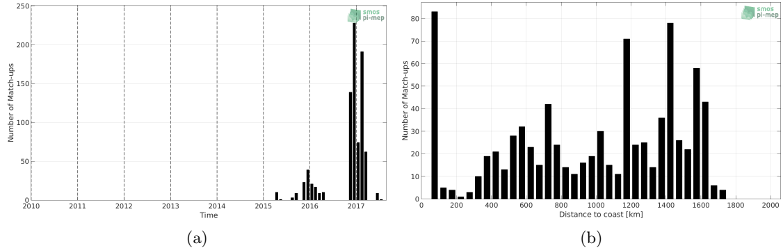
Figure 1: Number of match-ups between Sea mammals and SMAP-L2-RSS-V4 SSS as a function of time (a) and as function of the distance to coast (b) over the Southern Ocean Pi-MEP region and for the full satellite product period.
