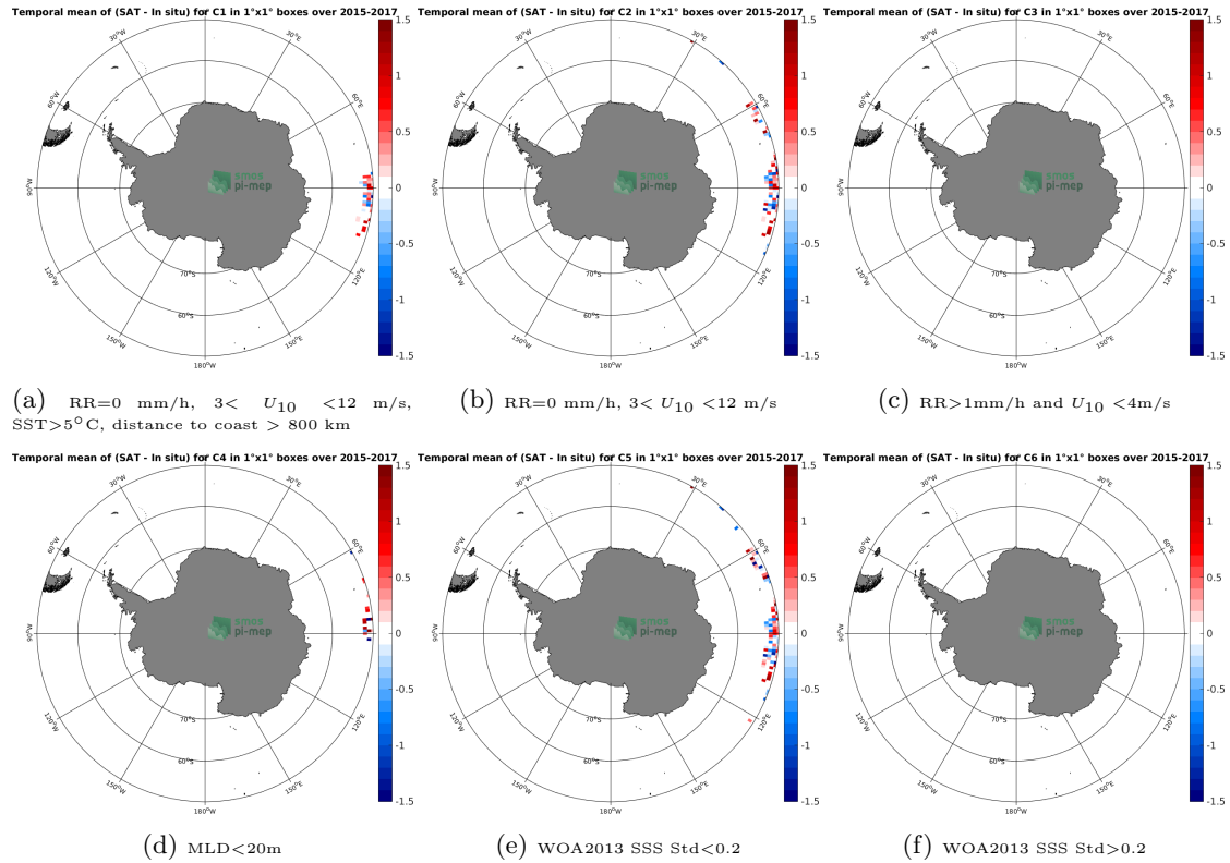
Figure 12: Temporal mean gridded over spatial boxes of size 1^{\circ}\times 1^{\circ} of \Delta\text{SSS} (SMAP-L2-RSS-V4 - Sea mammals) for 6 different subdatasets corresponding to: \text{RR}=0 mm/h, 3 < U_{10} < 12 m/s, \text{SST} > 5^{\circ}\text{C} , distance to coast > 800 km (a), \text{RR}=0 mm/h, 3 < U_{10} < 12 m/s (b), \text{RR} > 1 mm/h and U_{10} < 4 m/s (c), \text{MLD} < 20\text{m} (d), \text{WOA2013 SSS Std} < 0.2 (e), \text{WOA2013 SSS Std} > 0.2 (f).
