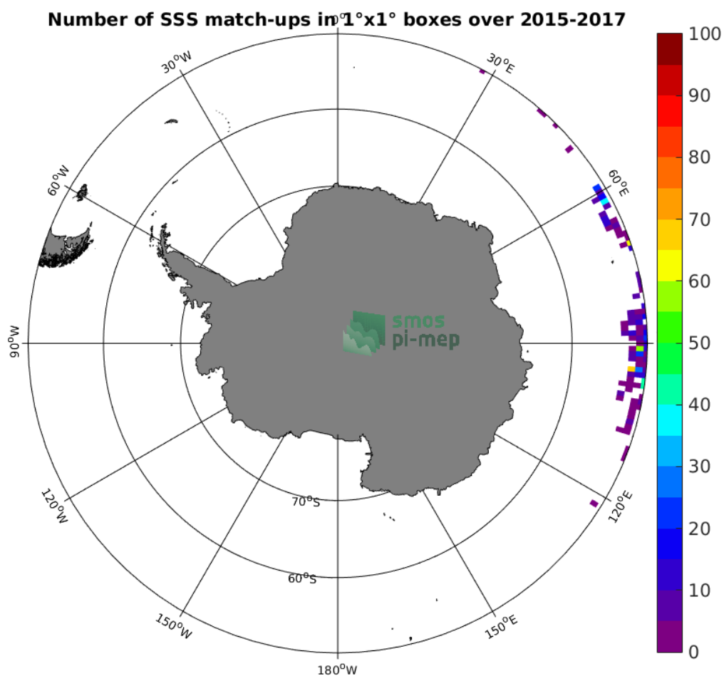
Figure 4: Number of SSS match-ups between Sea mammals SSS and the SMAP-L2-RSS-V4 SSS product for the Southern Ocean Pi-MEP region over 1^\circ \times 1^\circ boxes and for the full satellite product period.
