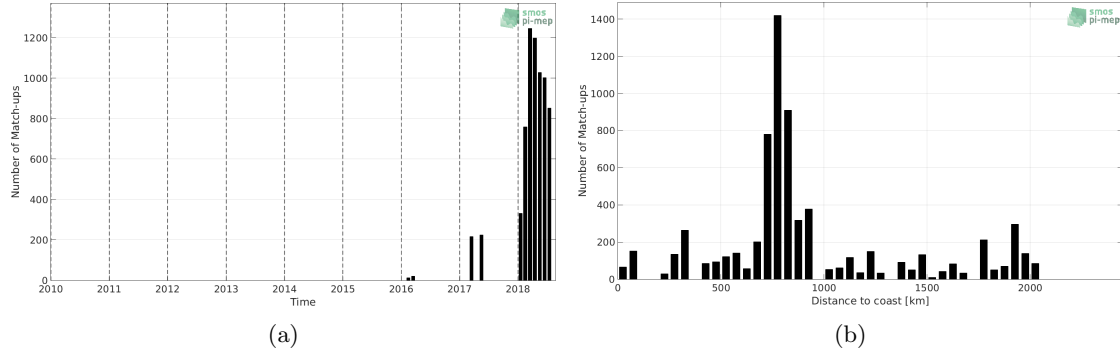
Figure 1: Number of match-ups between Surface drifters and SMAP SSS L2 v4 (RSS) SSS as a function of time (a) and as function of the distance to coast (b) over the Southern Ocean Pi-MEP region and for the full satellite product period.
