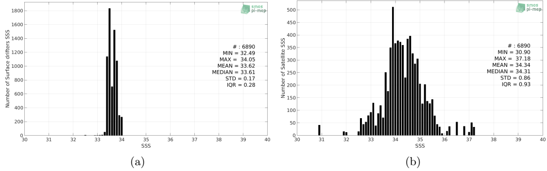
Figure 2: Histograms of SSS from Surface drifters (a) and SMAP SSS L2 v4 (RSS) (b) considering all match-up pairs per bins of 0.1 over the Southern Ocean Pi-MEP region and for the full satellite product period.
