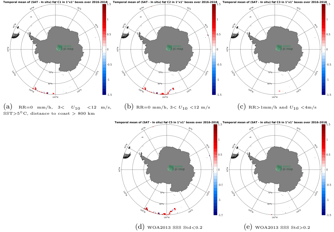
Figure 11: Temporal mean gridded over spatial boxes of size 1^{\circ}\times 1^{\circ} of \Delta\text{SSS} (SMAP SSS L2 v4 (RSS) - Surface drifters) for 5 different subdatasets corresponding to:RR=0 mm/h, 3 < U_{10} < 12 m/s, SST >5^{\circ}\text{C} , distance to coast > 800 km (a), RR=0 mm/h, 3 < U_{10} < 12 m/s (b), RR >1 mm/h and U_{10} < 4 m/s (c), WOA2013 SSS Std <0.2 (d), WOA2013 SSS Std >0.2 (e).
