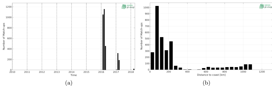
Figure 1: Number of match-ups between TSG-POLARSTERN and SMAP-L2-RSS-V3-70KM SSS as a function of time (a) and as function of the distance to coast (b) over the Southern Ocean Pi-MEP region and for the full satellite product period.
