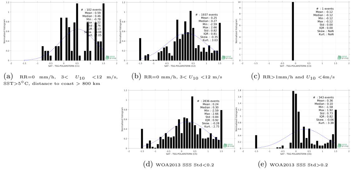
Figure 13: Normalized histogram of \Delta SSS (SMAP-L2-RSS-V3-70KM - TSG-POLARSTERN) for 5 different subdatasets corresponding to: RR=0 mm/h, 3 < U_{10} < 12 m/s, SST > 5°C, distance to coast > 800 km (a), RR=0 mm/h, 3 < U_{10} < 12 m/s (b), RR > 1mm/h and U_{10} < 4 m/s (c), WOA2013 SSS Std < 0.2 (d), WOA2013 SSS Std > 0.2 (e).
