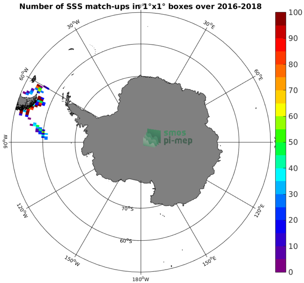
Figure 4: Number of SSS match-ups between TSG-POLARSTERN SSS and the SMAP-L2-RSS-V3-70KM SSS product for the Southern Ocean Pi-MEP region over 1°x1° boxes and for the full satellite product period.
