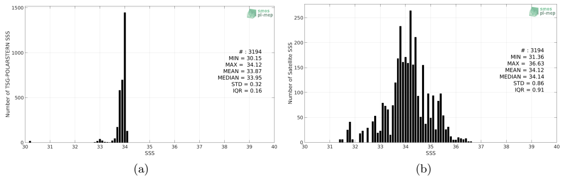
Figure 2: Histograms of SSS from TSG-POLARSTERN (a) and SMAP-L2-RSS-V3-70KM (b) considering all match-up pairs per bins of 0.1 over the Southern Ocean Pi-MEP region and for the full satellite product period.
