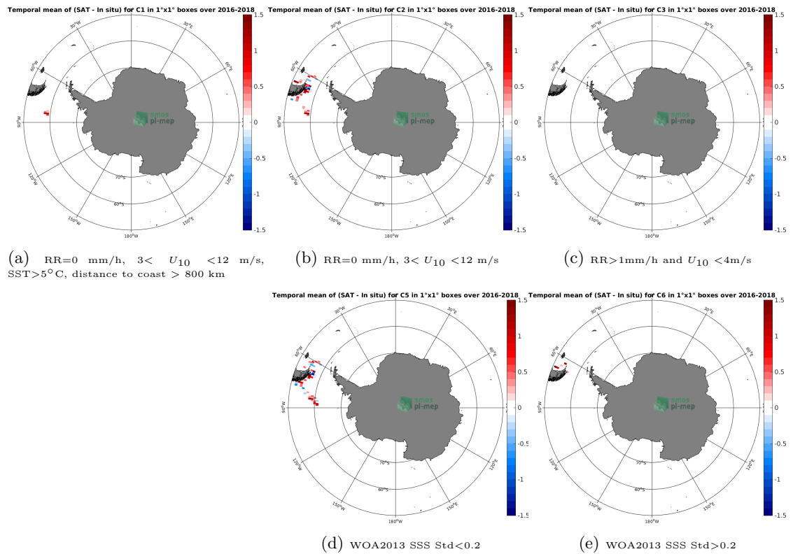
Figure 12: Temporal mean gridded over spatial boxes of size 1^\circ \times 1^\circ of \Delta SSS (SMAP-L2-RSS-V3-70KM - TSG-POLARSTERN) for 5 different subdatasets corresponding to:RR=0 mm/h, 3 < U_{10} < 12 m/s, SST >5^\circ C, distance to coast > 800 km (a), RR=0 mm/h, 3 < U_{10} < 12 m/s (b), RR >1 mm/h and U_{10} < 4 m/s (c), WOA2013 SSS Std <0.2 (d), WOA2013 SSS Std >0.2 (e).
