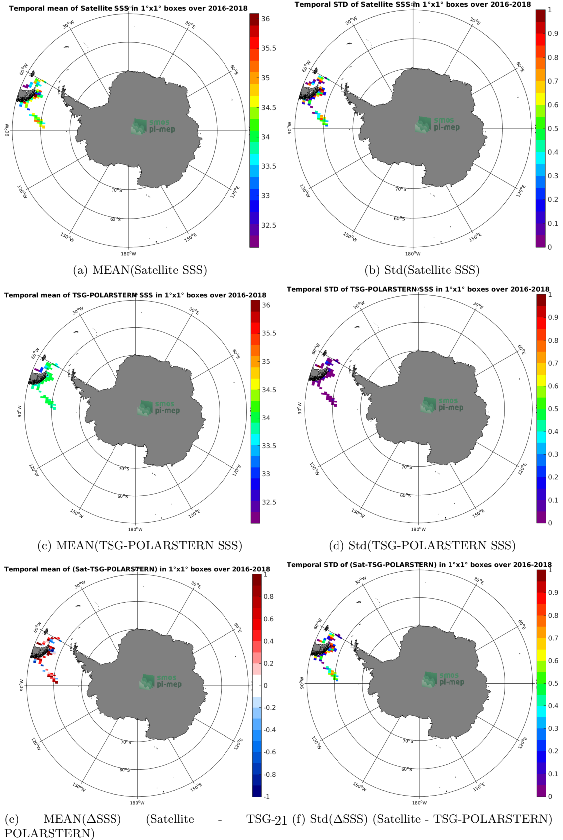
Figure 6: Temporal mean (left) and Std (right) of SSS from SMAP-L2-RSS-V3-70KM (top), TSG-POLARSTERN (middle), and of \Delta SSS (Satellite - TSG-POLARSTERN). Only match-up pairs are used to generate these maps.
