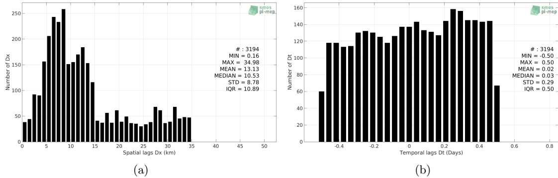
Figure 5: Histograms of the spatial (a) and temporal (b) lags between the time of the TSG-POLARSTERN measurements and the date of the corresponding SMAP-L2-RSS-V3-70KM SSS product.
