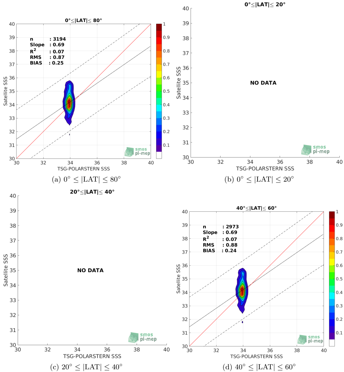
Figure 9: Contour maps of the concentration of SMAP-L2-RSS-V3-70KM SSS (y-axis) versus TSG-POLARSTERN SSS (x-axis) at match-up pairs for different latitude bands. For each plot, the red line shows x=y . The black thin and dashed lines indicate a linear fit through the data cloud and the \pm 95\% confidence levels, respectively. The number match-up pairs n , the slope and R^2 coefficient of the linear fit, the root mean square (RMS) and the mean bias between satellite and in situ data are indicated for each latitude band in each plots.
