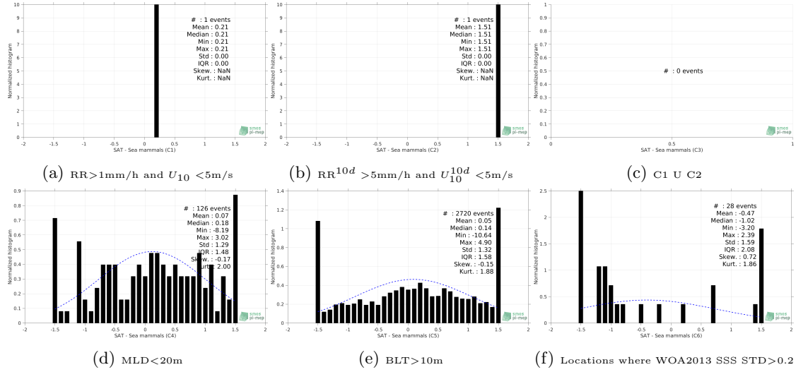
Figure 13: Normalized histogram of \Delta\text{SSS} (SMAP-L2-RSS-V3-70KM - Sea mammals) for 6 different subdatasets corresponding to: RR > 1\text{mm/h} and U_{10} < 5\text{m/s} (a), RR^{10d} > 5\text{mm/h} and U_{10}^{10d} < 5\text{m/s} (b), C1 U C2 (c), MLD < 20\text{m} (d), BLT > 10\text{m} (e), Locations where WOA2013 SSS STD > 0.2 (f).
