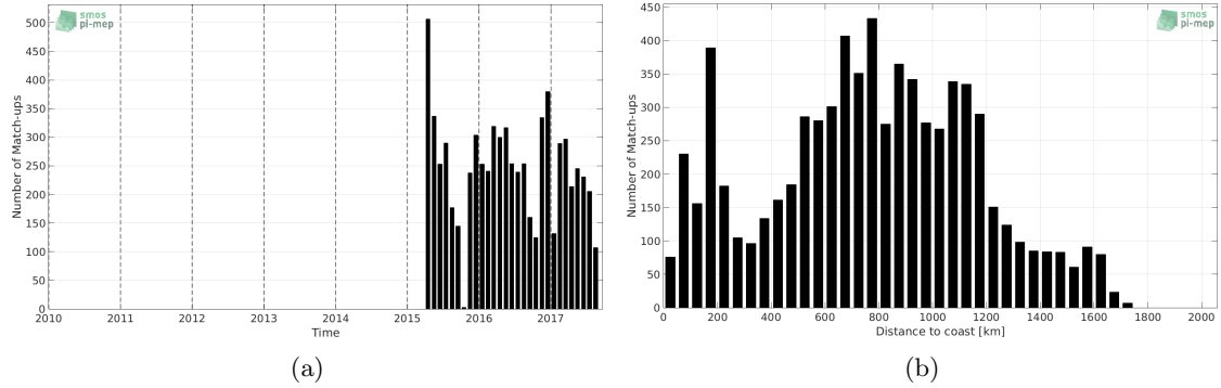
Figure 1: Number of match-ups between Sea mammals and SMAP-L2-RSS-V3-70KM SSS as a function of time (a) and as function of the distance to coast (b) over the Southern Ocean Pi-MEP region and for the full satellite product period.
