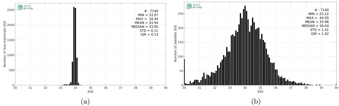
Figure 2: Histograms of SSS from Sea mammals (a) and SMAP-L2-RSS-V3-70KM (b) considering all match-up pairs per bins of 0.1 over the Southern Ocean Pi-MEP region and for the full satellite product period.
