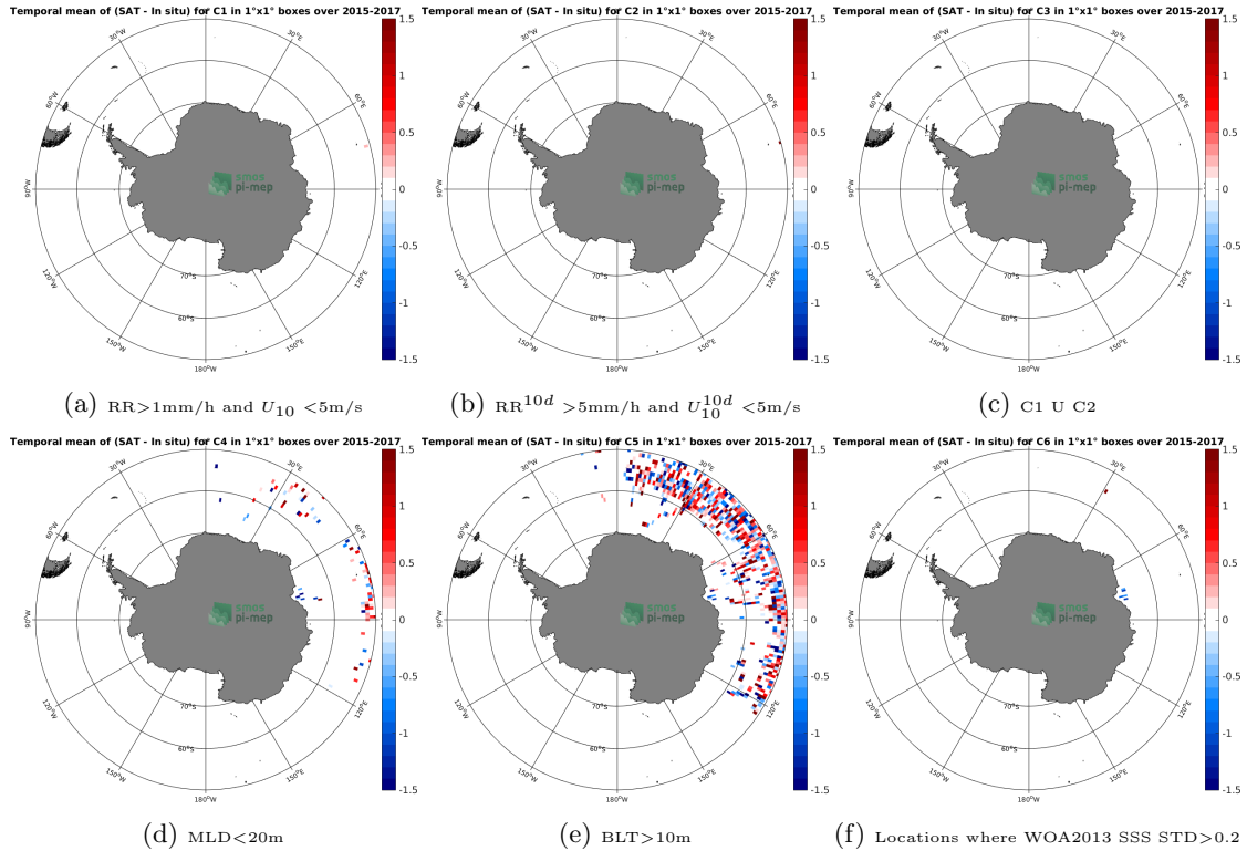
Figure 12: Temporal mean gridded over spatial boxes of size 1^\circ \times 1^\circ of \Delta SSS (SMAP-L2-RSS-V3-70KM - Sea mammals) for 6 different subdatasets corresponding to:RR>1mm/h and U_{10} < 5m/s (a), RR^{10d} > 5mm/h and U_{10}^{10d} < 5m/s (b), C1 U C2 (c),MLD<20m (d),BLT>10m (e),Locations where WOA2013 SSS STD>0.2 (f).
