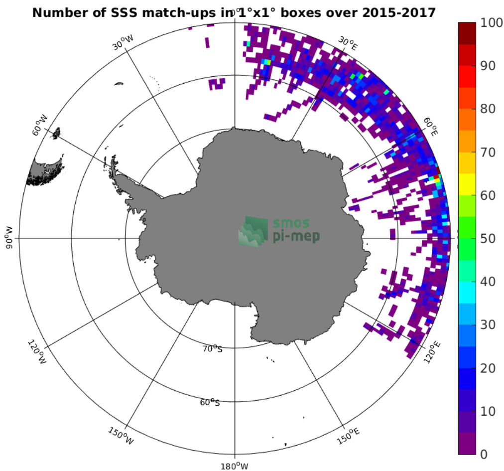
Figure 4: Number of SSS match-ups between Sea mammals SSS and the SMAP-L2-RSS-V3-70KM SSS product for the Southern Ocean Pi-MEP region over 1°x1° boxes and for the full satellite product period.
