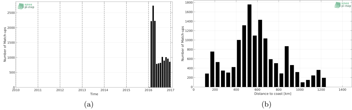
Figure 1: Number of match-ups between Surface drifters and SMAP-L2-RSS-V3-70KM SSS as a function of time (a) and as function of the distance to coast (b) over the Southern Ocean Pi-MEP region and for the full satellite product period.
