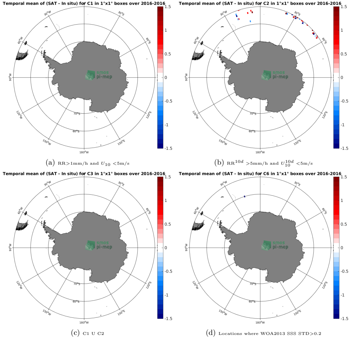
Figure 11: Temporal mean gridded over spatial boxes of size 1^\circ \times 1^\circ of \Delta SSS (SMAP-L2-RSS-V3-70KM - Surface drifters) for 4 different subdatasets corresponding to:RR > 1mm/h and U_{10} < 5 m/s (a), RR^{10d} > 5 mm/h and U_{10}^{10d} < 5 m/s (b), C1 U C2 (c),Locations where WOA2013 SSS STD > 0.2 (d).
