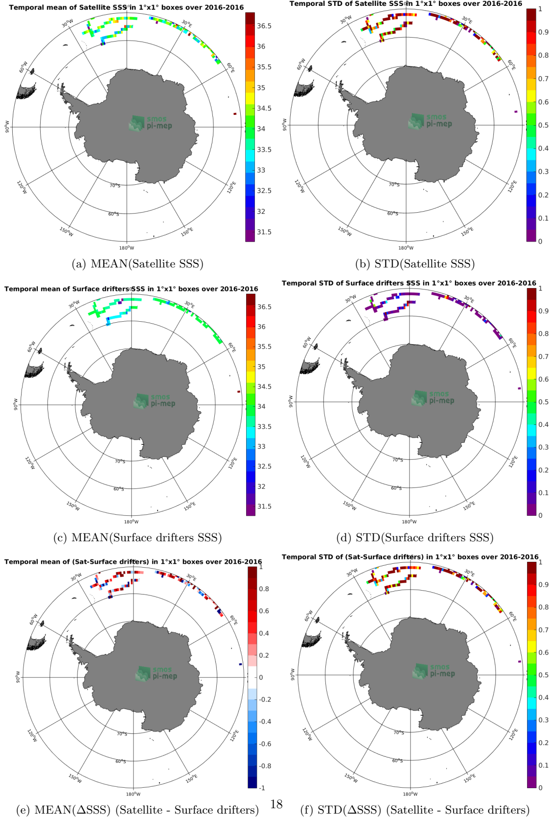
Figure 5: Temporal mean (left) and STD (right) of SSS from SMAP-L2-RSS-V3-70KM (top), Surface drifters (middle), and of \Delta SSS (Satellite - Surface drifters). Only match-up pairs are used to generate these maps.
