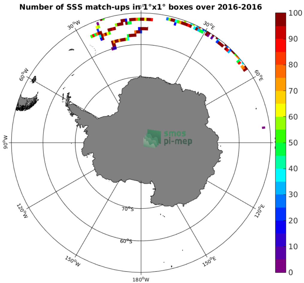
Figure 3: Number of SSS match-ups between Surface drifters SSS and the SMAP-L2-RSS-V3-70KM SSS product for the Southern Ocean Pi-MEP region over 1^\circ \times 1^\circ boxes and for the full satellite product period.
