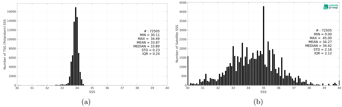
Figure 2: Histograms of SSS from TSG (Polarstern) (a) and SMAP SSS L2 v5.0 (JPL) (b) considering all match-up pairs per bins of 0.1 over the Southern Ocean Pi-MEP region and for the full satellite product period.
