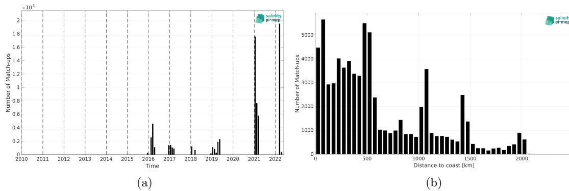
Figure 1: Number of match-ups between TSG (Polarstern) and SMAP SSS L2 v5.0 (JPL) SSS as a function of time (a) and as function of the distance to coast (b) over the Southern Ocean Pi-MEP region and for the full satellite product period.
