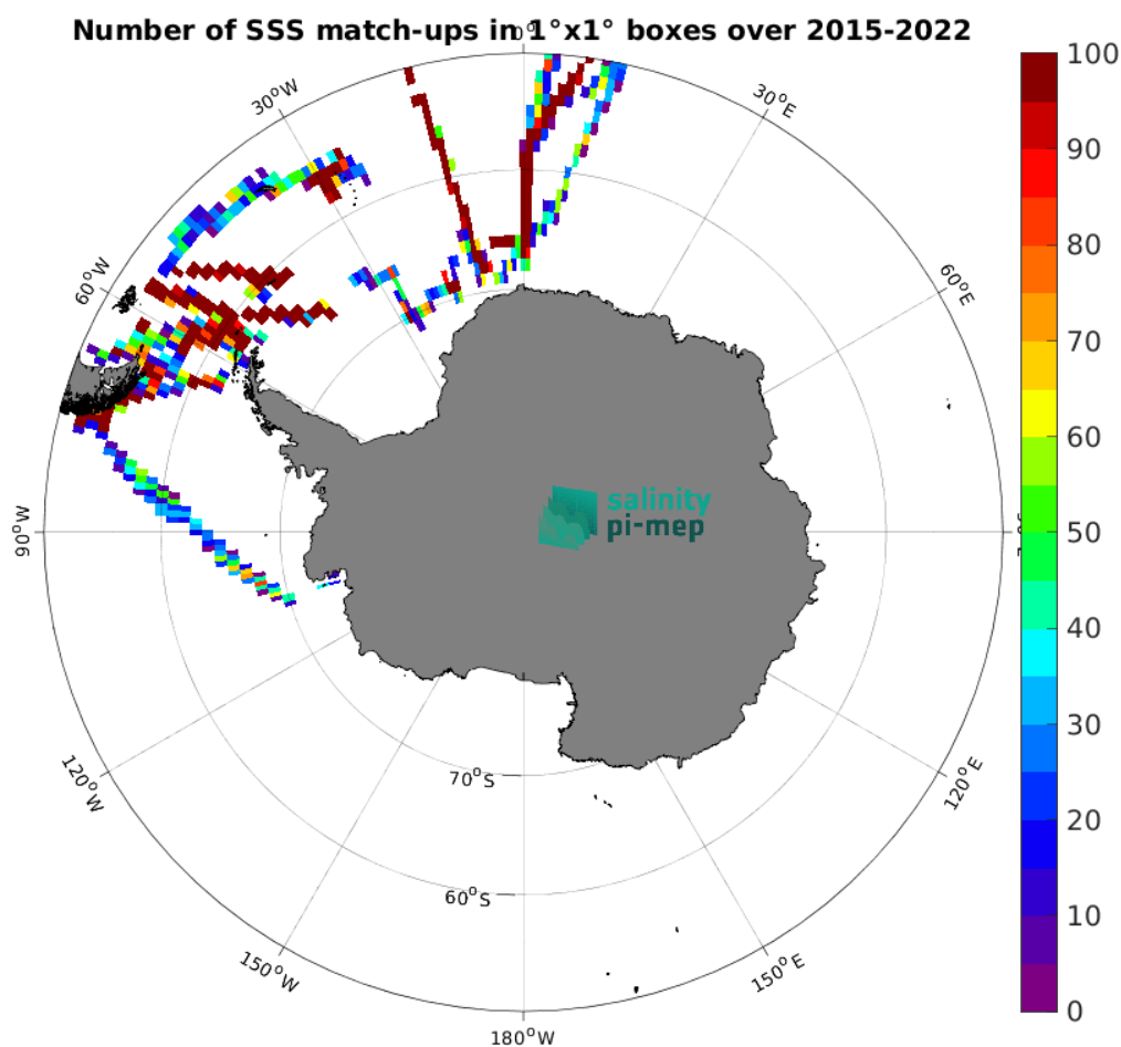
Figure 4: Number of SSS match-ups between TSG (Polarstern) SSS and the SMAP SSS L2 v5.0 (JPL) SSS product for the Southern Ocean Pi-MEP region over 1^\circ \times 1^\circ boxes and for the full satellite product period.
