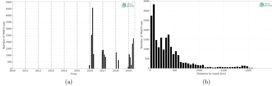
Figure 1: Number of match-ups between TSG (Polarstern) and SMAP SSS L2 v5.0 (JPL) SSS as a function of time (a) and as function of the distance to coast (b) over the Southern Ocean Pi-MEP region and for the full satellite product period.
