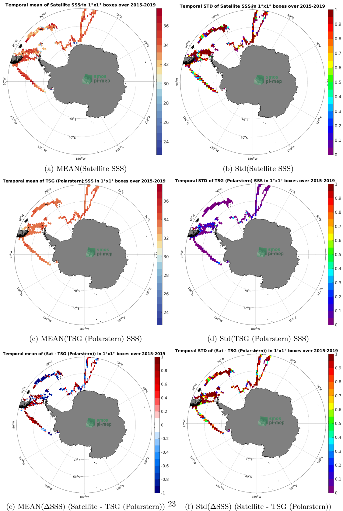
Figure 6: Temporal mean (left) and Std (right) of SSS from SMAP SSS L2 v5.0 (JPL) (top), TSG (Polarstern) (middle), and of \Delta SSS (Satellite - TSG (Polarstern)). Only match-up pairs are used to generate these maps.
