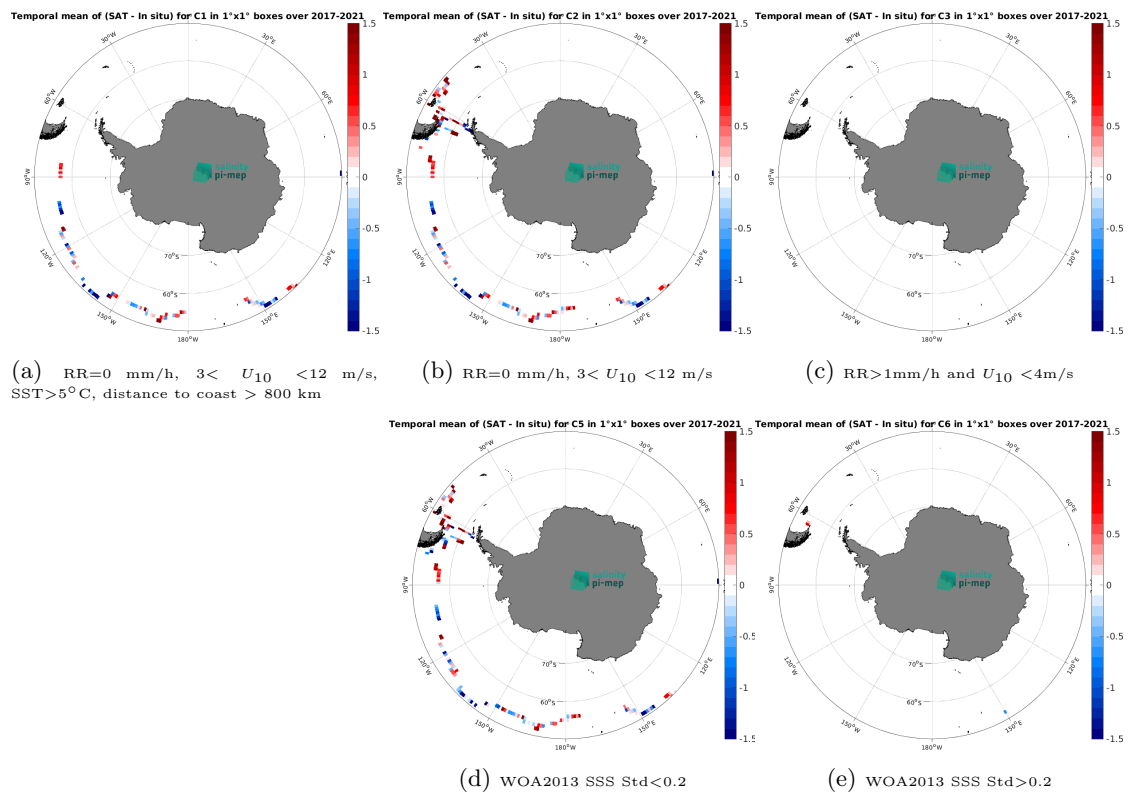
Figure 14: Temporal mean gridded over spatial boxes of size 1^\circ \times 1^\circ of \Delta SSS (SMAP SSS L2 v5.0 (JPL) - TSG (GOSUD-Sailing-ship)) for 5 different subdatasets corresponding to:RR=0 mm/h, 3 < U_{10} < 12 m/s, SST>5°C, distance to coast > 800 km (a), RR=0 mm/h, 3 < U_{10} < 12 m/s (b), RR>1mm/h and U_{10} < 4 m/s (c), WOA2013 SSS Std<0.2 (d), WOA2013 SSS Std>0.2 (e).
