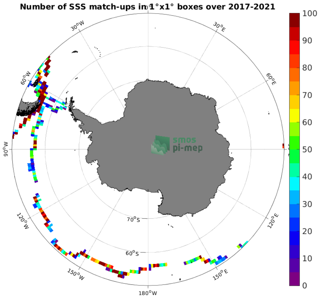
Figure 4: Number of SSS match-ups between TSG (GOSUD-Sailing-ship) SSS and the SMAP SSS L2 v5.0 (JPL) SSS product for the Southern Ocean Pi-MEP region over 1^\circ \times 1^\circ boxes and for the full satellite product period.
