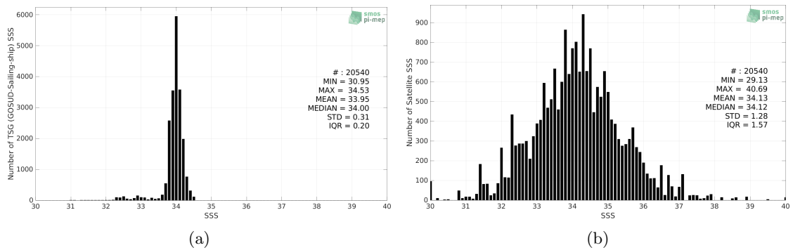
Figure 2: Histograms of SSS from TSG (GOSUD-Sailing-ship) (a) and SMAP SSS L2 v5.0 (JPL) (b) considering all match-up pairs per bins of 0.1 over the Southern Ocean Pi-MEP region and for the full satellite product period.
